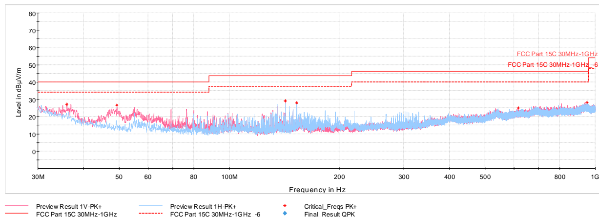
Plot 7-38. Radiated Spurious Emissions below 1GHz (HDR4 ePA – Ch.38, Pol. H & V, with AC/DC Adapter + Magnetic Charger)
