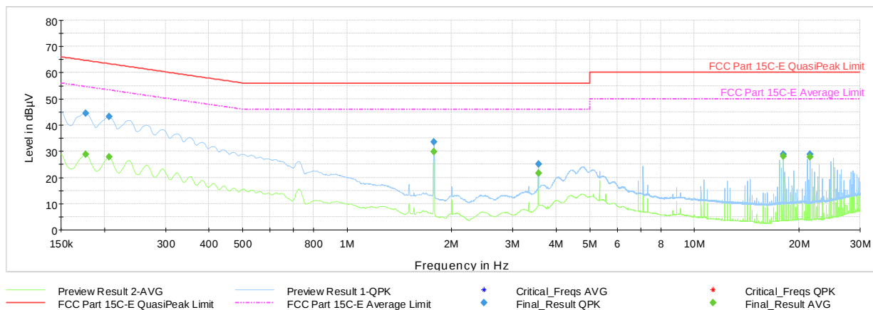
Plot 7-43. AC Line-Conducted Emissions (L1, GFSK ePA – Ch.39 with AC/DC Adapter + Magnetic Charger)
