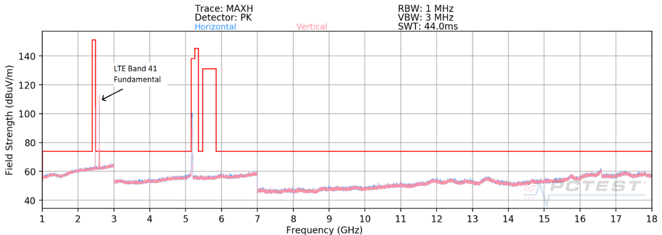
Plot 7-34. Radiated Spurious Emissions above 1GHz – Simultaneous Transmission
