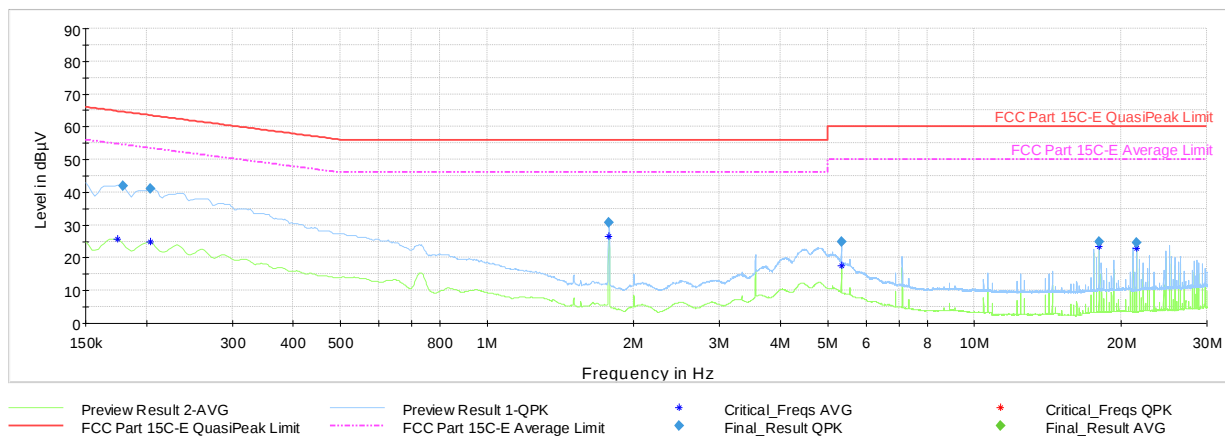
Plot 7-44. AC Line-Conducted Emissions (N, GFSK ePA – Ch.39 with AC/DC Adapter + Magnetic Charger)
