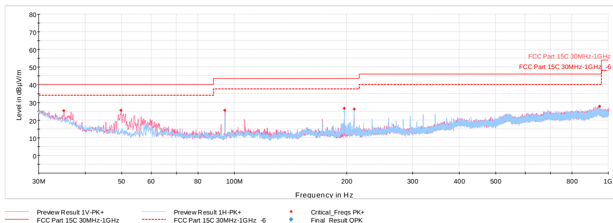
Plot 7-42. Radiated Spurious Emissions below 1GHz - Simultaneous Transmission with AC/DC Adapter + Magnetic Charger
