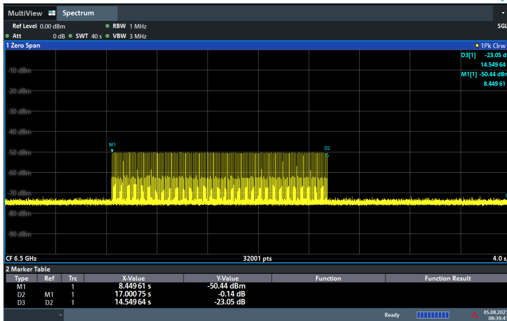
Plot 7-11. Cessation Time – Mode2 (Ch. 5, 6.5 GHz)
