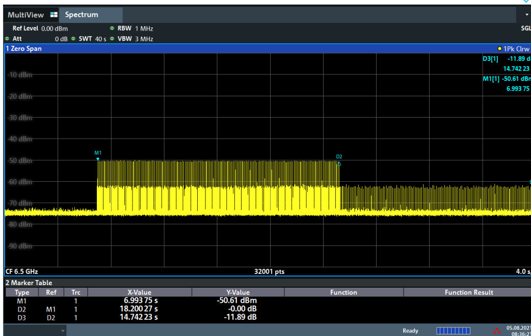
Plot 7-9. Cessation Time – Mode1 (Ch. 5, 6.5 GHz)
