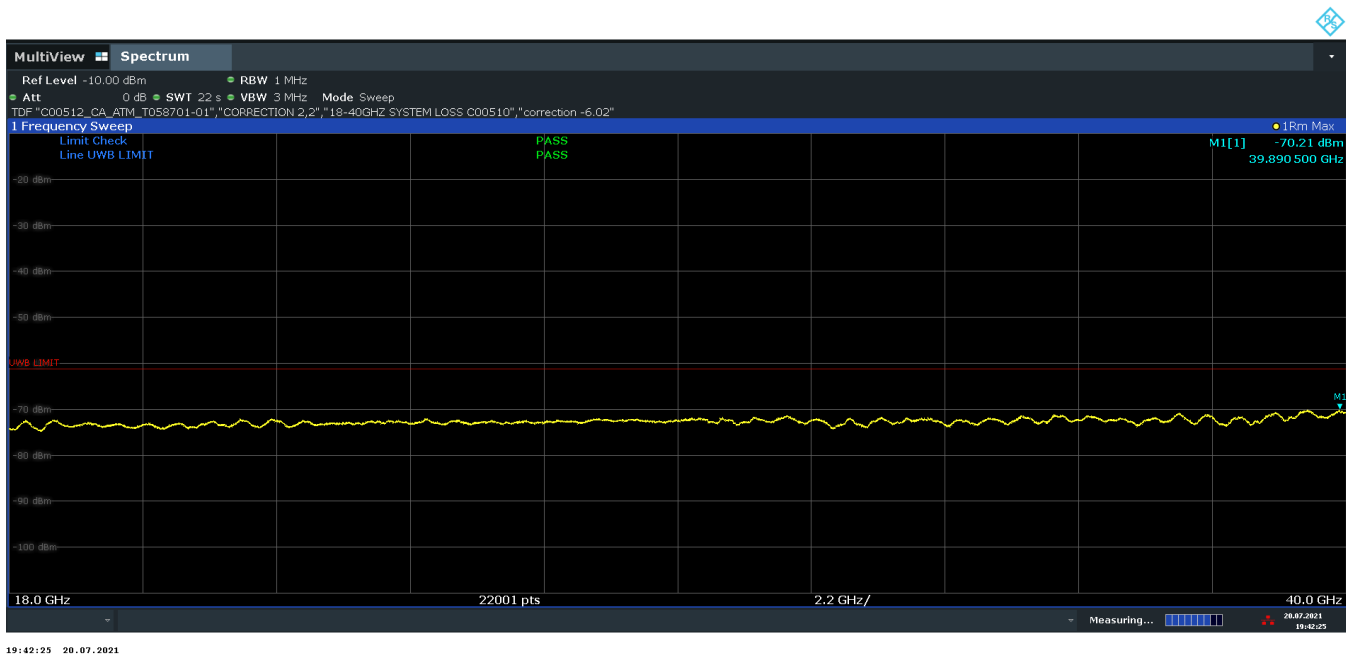
Plot 7-38. Radiated Spurious Emission 18-40GHz (Ch. 9, Config 3, Payload 125 Ant. Pol. V)
