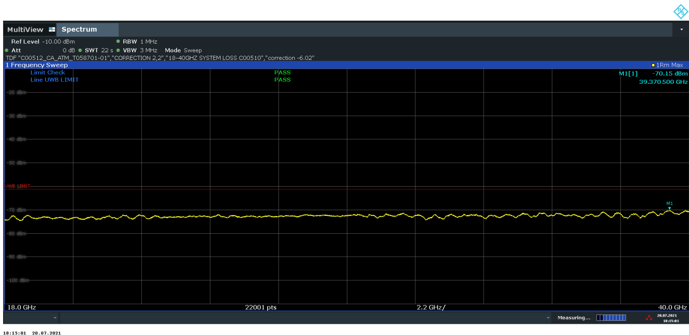
Plot 7-37. Radiated Spurious Emission 18-40GHz (Ch. 9, Config 3, Payload 125 Ant. Pol. H)
