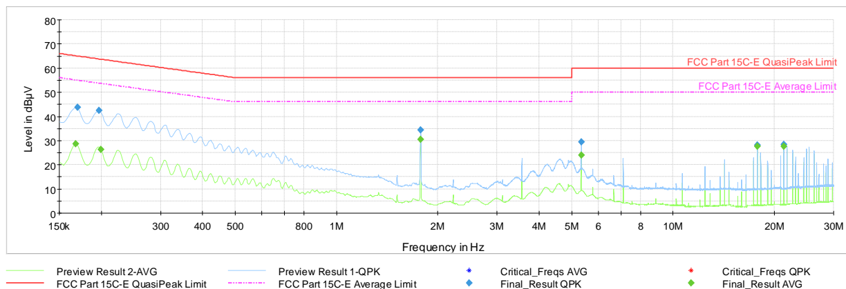
Plot 7-43. AC Line Conducted (Ch. 9, Config 3, Payload 125 L1, with AC/DC Adapter + Magnetic Charger)
