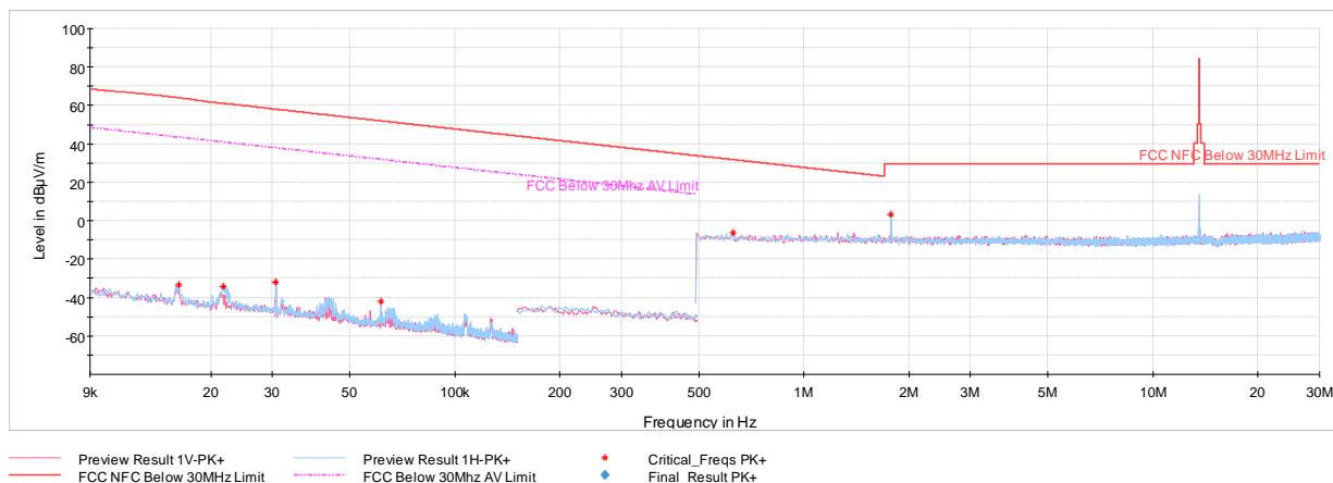
Plot 7-9. Radiated Spurious Emissions 9kHz – 30MHz (Reader 10% ASK 1 out of 256, with AC/DC Adapter and Magnetic Charger)
