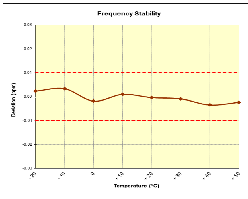
Figure 7-3. Frequency Stability Plot (CE A 848kbps)
