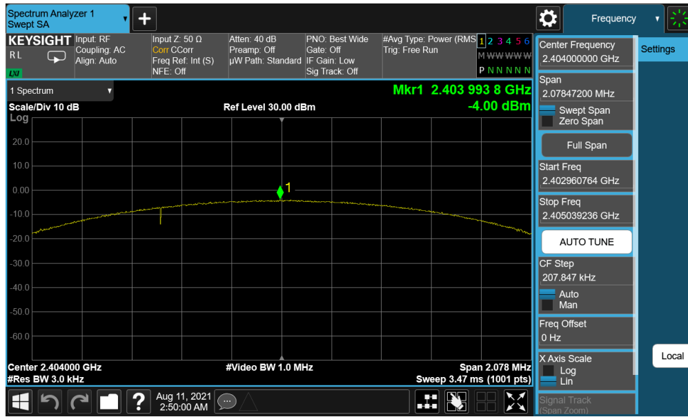
Plot 7-13. Power Spectral Density Plot (Bluetooth (LE), 2Mbps, ePA – Ch. 1)
