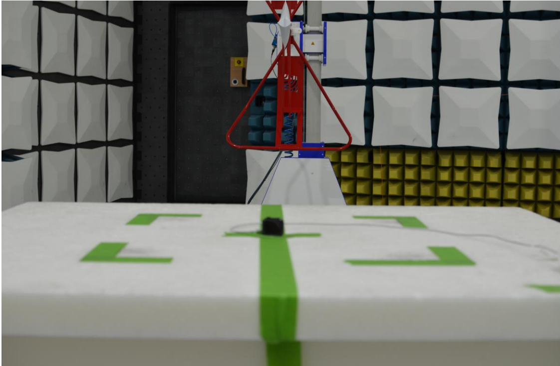
Figure 11: 30MHz-960MHz Test Setup (Rear View)
