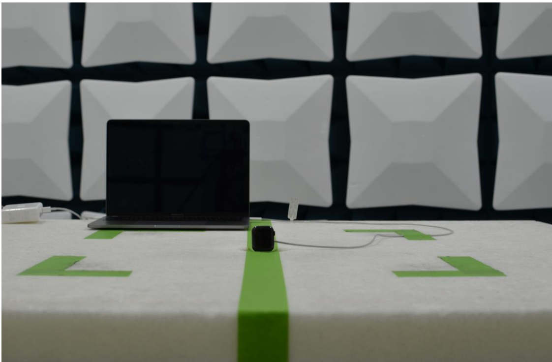
Figure 18: 30MHz-960MHz Test Setup (Front View)
