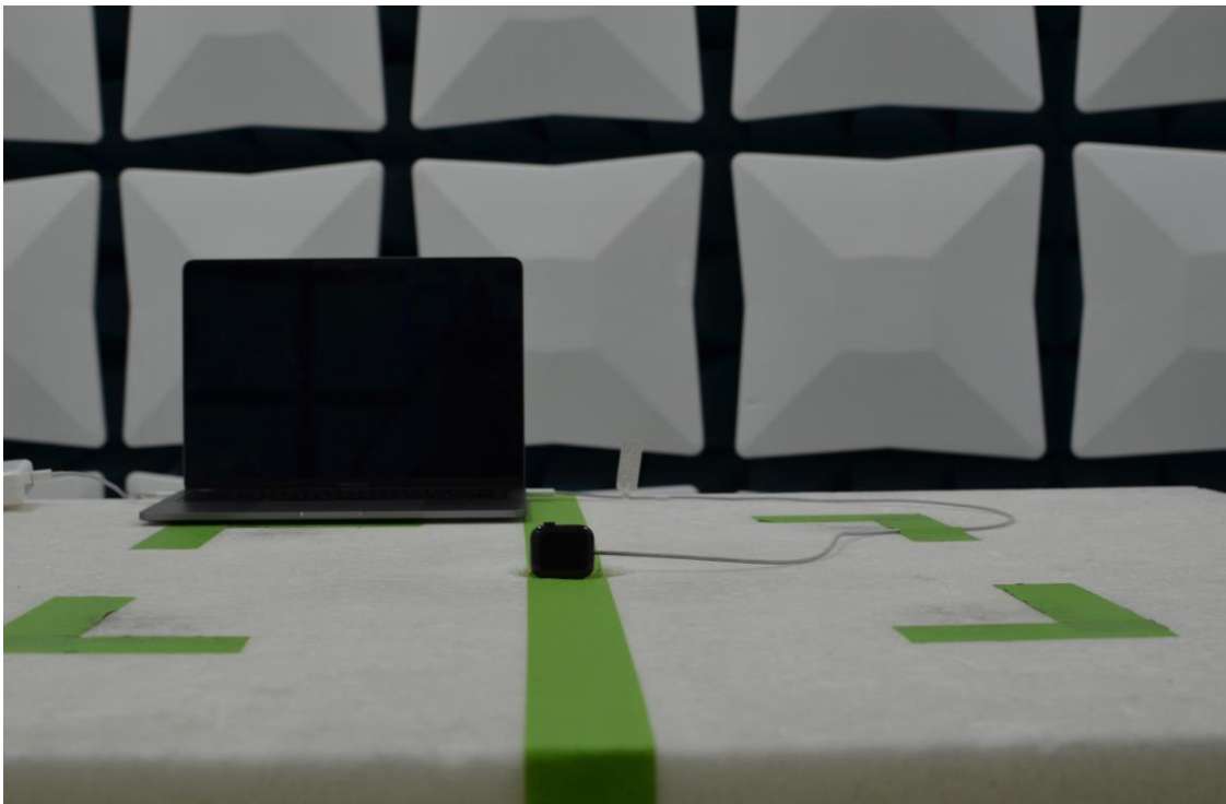
Figure 16: 30MHz-960MHz Test Setup (Front View)
