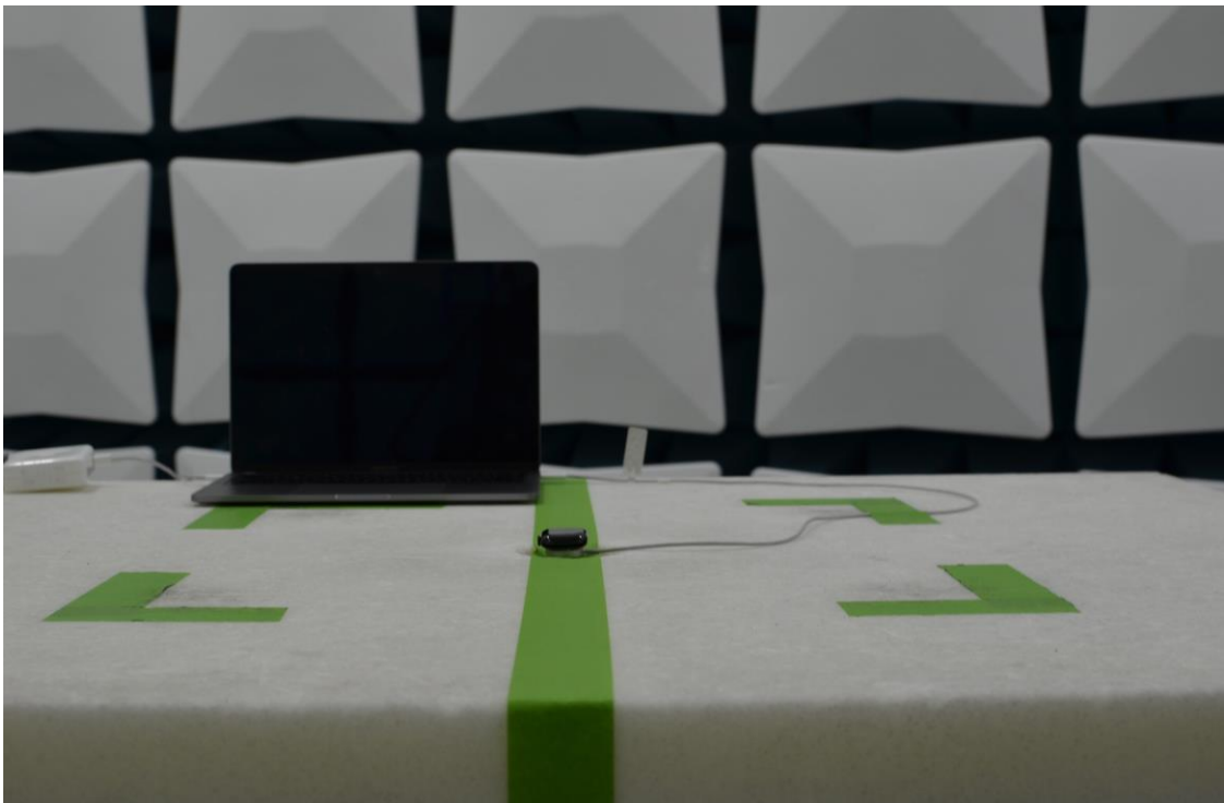
Figure 14: 30MHz-960MHz Test Setup (Front View)
