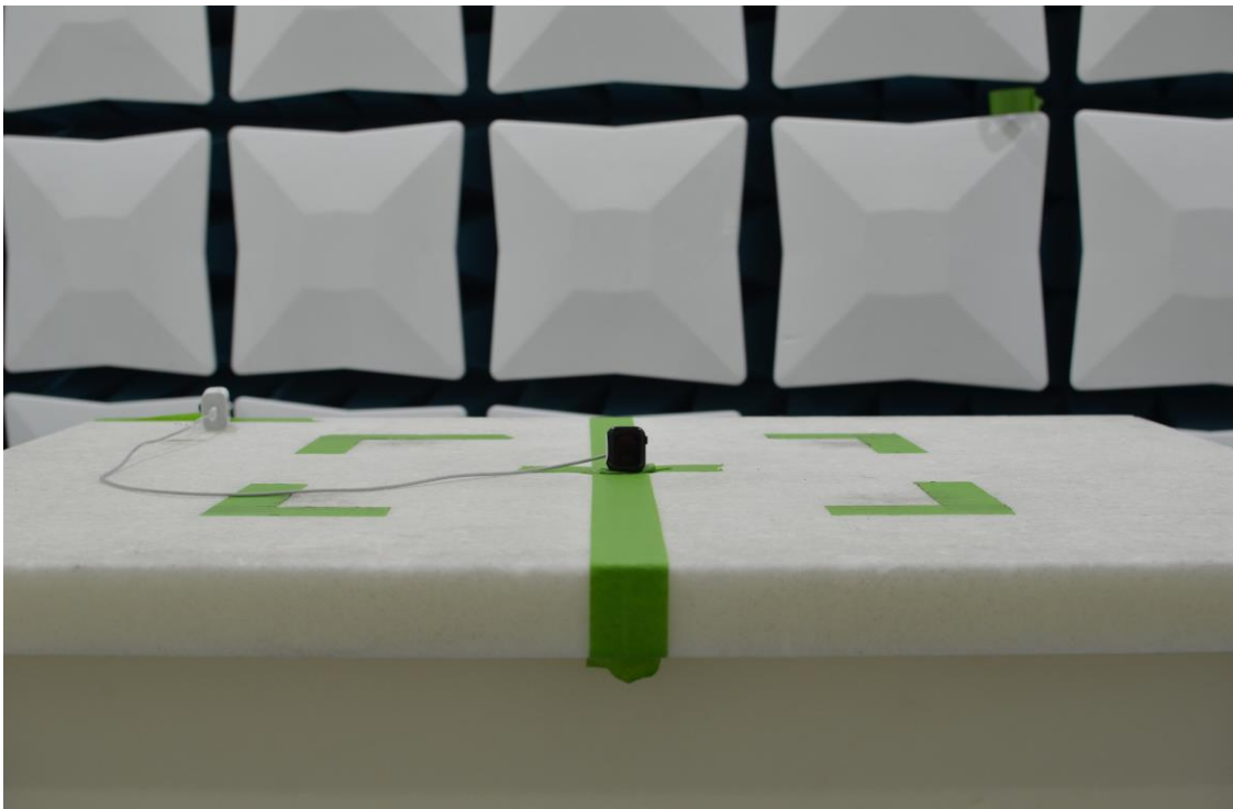
Figure 12: 30MHz-960MHz Test Setup (Front View)
