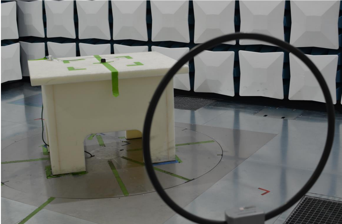
Figure 21: 9kHz-30MHz Test Setup (Front View)
