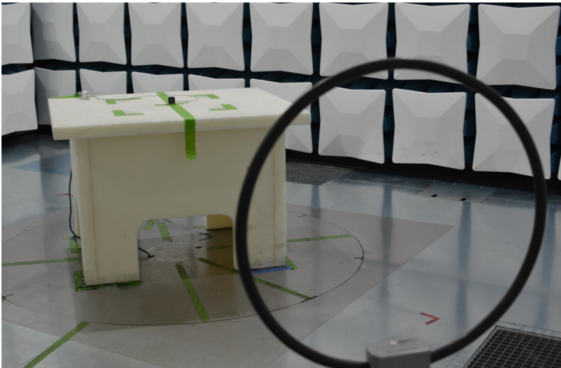
Figure 22: 9kHz-30MHz Test Setup (Front View)
