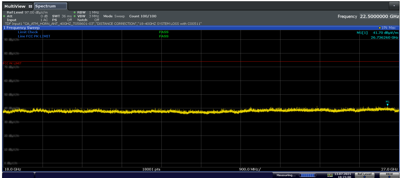
Plot 7-32. Radiated Spurious Emissions above 18GHz (GFSK ePA – Ch.0, Pol. H)
