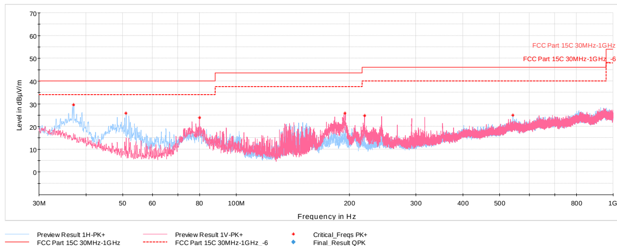
Plot 7-41. Radiated Spurious Emissions below 1GHz (GFSK ePA – Ch.0, Pol. H & V, with AC/DC Adapter + Magnetic Charger)
