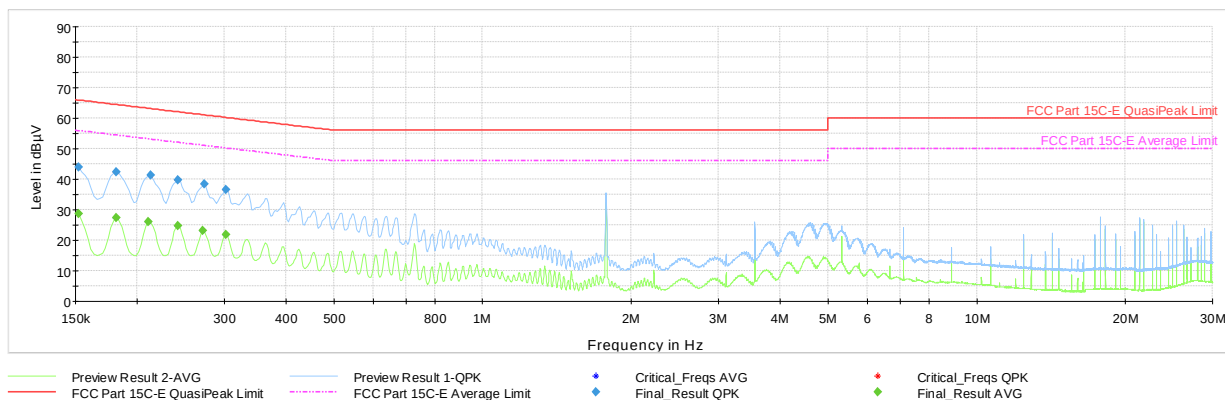
Plot 7-44. AC Line-Conducted Emissions (N, GFSK ePA – Ch.0 with AC/DC Adapter + Magnetic Charger)
