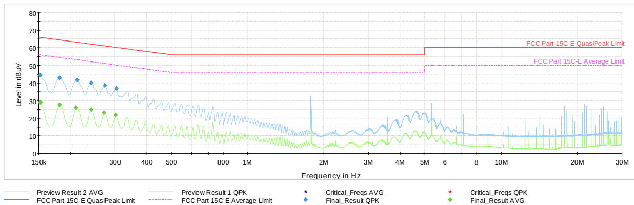
Plot 7-43. AC Line-Conducted Emissions (L1, GFSK ePA – Ch.0 with AC/DC Adapter + Magnetic Charger)
