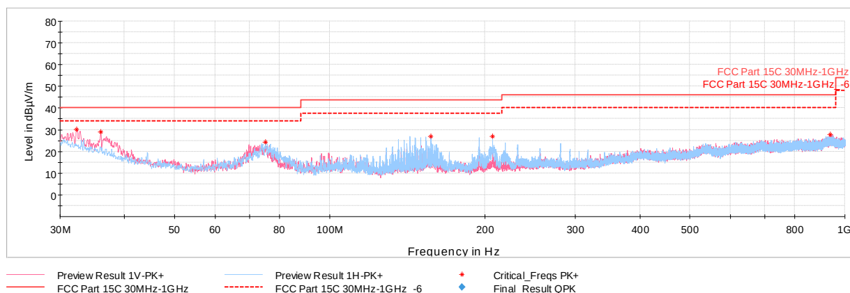
Plot 7-42. Radiated Spurious Emissions below 1GHz – Simultaneous Transmission with AC/DC Adapter + Magnetic Charger
