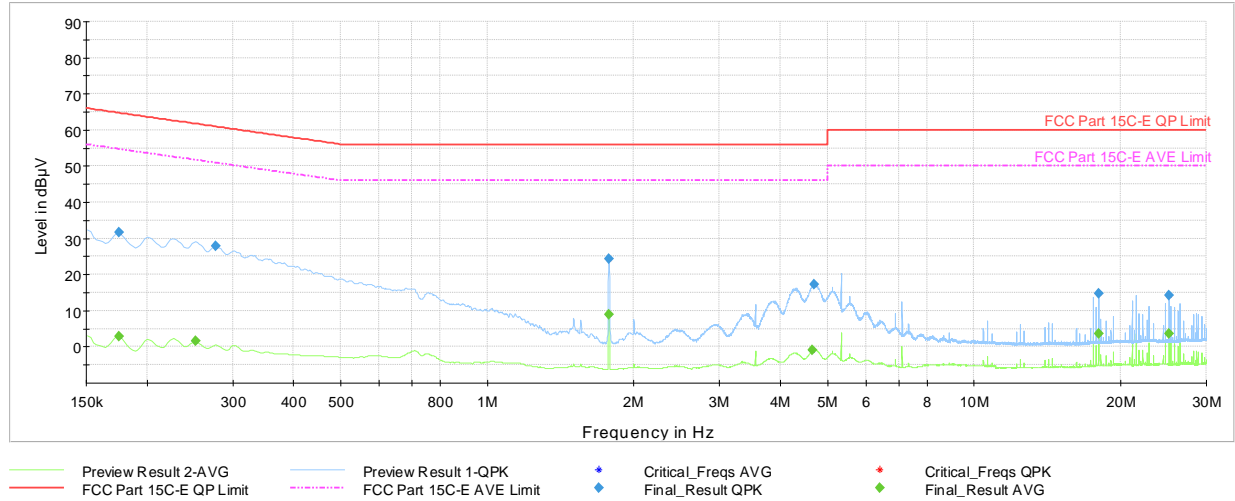
Plot 7-59. AC Line Conducted Plot with 802.11n UNII Band 3 – Ch.149 (N) with AC/DC Adaptor & Magnetic Charger
