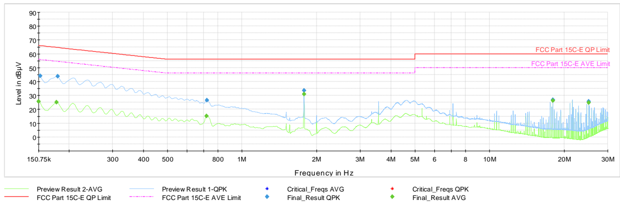
Plot 7-58. AC Line Conducted Plot with 802.11n UNII Band 3 – Ch.149 (L1) with AC/DC Adaptor & Magnetic Charger
