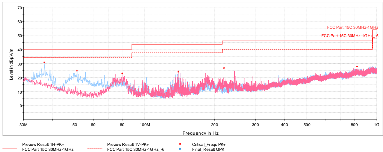
Plot 7-56. Radiated Spurious Emissions below 1GHz (802.11n – UNII 3 Ch. 149) with AC/DC Adaptor & Magnetic Charger
