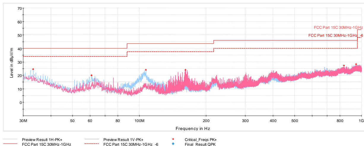
Plot 7-57. Radiated Spurious Emissions – Simultaneous Transmission below 1GHz with AC/DC Adaptor & Magnetic Charger
