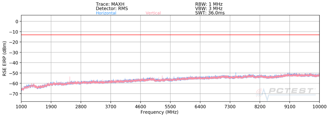
Plot 7-26. Antenna BCM Radiated Spurious Plot above 1GHz (LTE Band 26)
