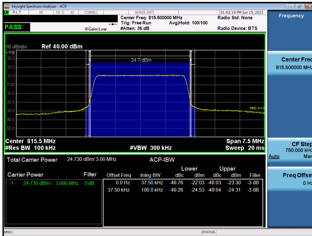
Plot 7-20. Channel Edge Plot (LTE Band 26 - 3MHz QPSK - Low Channel)
