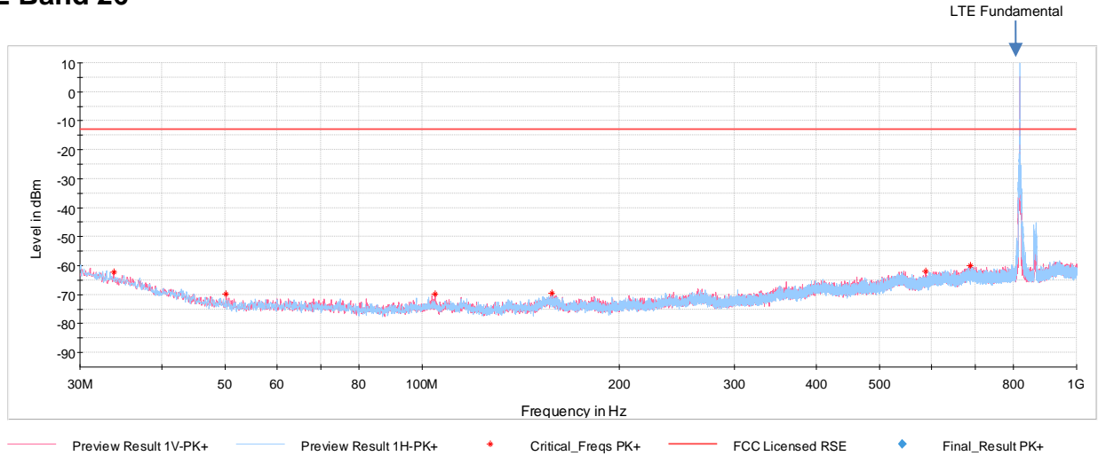
Plot 7-25. Antenna BCM Radiated Spurious Plot below 1GHz (LTE Band 26)
