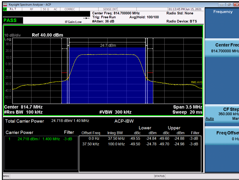
Plot 7-18. Channel Edge Plot (LTE Band 26 - 1.4MHz QPSK - Low Channel)
