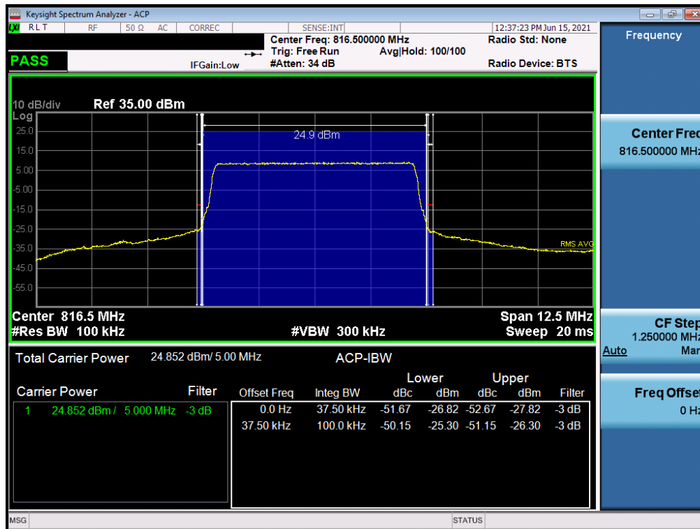
Plot 7-22. Channel Edge Plot (LTE Band 26 - 5MHz QPSK - Low Channel)
