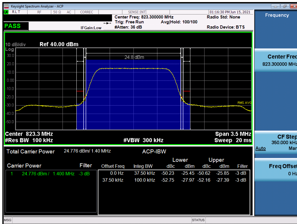
Plot 7-19. Channel Edge Plot (LTE Band 26 - 1.4MHz QPSK - High Channel)
