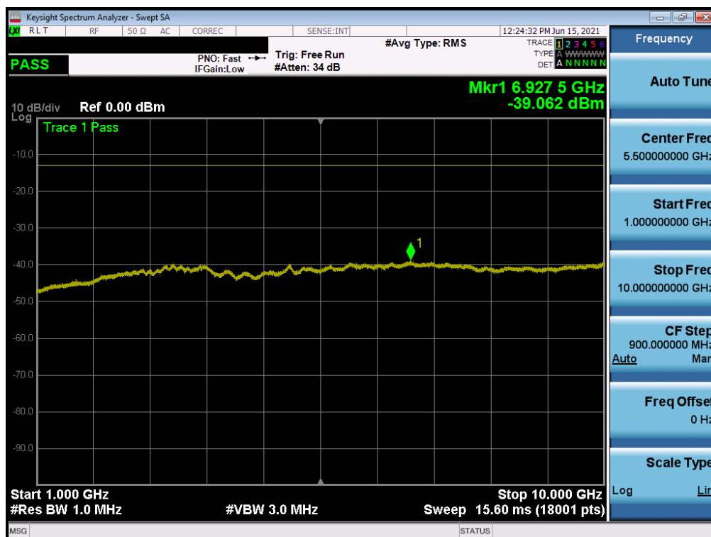
Plot 7-14. Conducted Spurious Plot (LTE Band 26 - 10MHz QPSK - RB Size 1, RB Offset 0 – Mid Channel)
