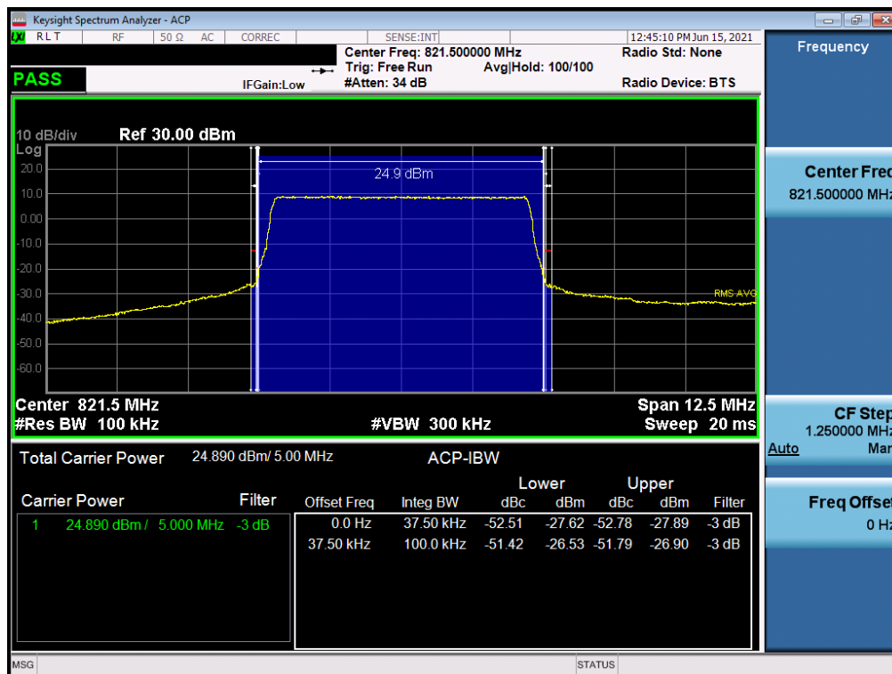
Plot 7-23. Channel Edge Plot (LTE Band 26 - 5MHz QPSK - High Channel)
