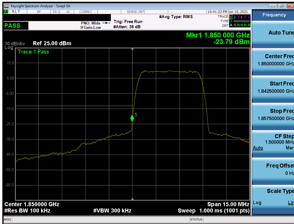
Plot 7-80. Lower Band Edge Plot (WCDMA PCS – Ch. 9262)
