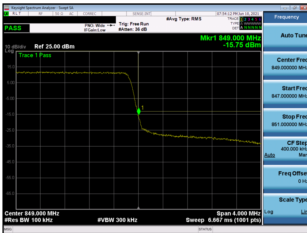
Plot 7-31. Upper BE Plot (LTE Band 5 - 3MHz QPSK – Full RB Configuration)
