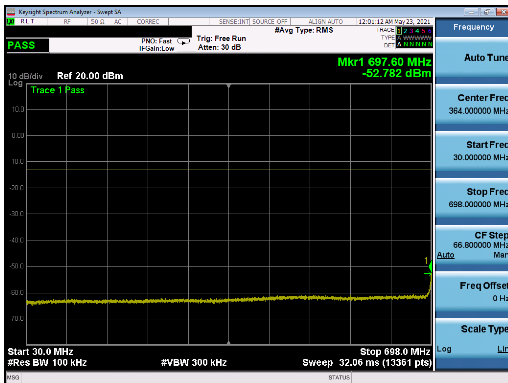
Plot 7-38. CSE (LTE Band 12/17 - 10MHz QPSK - RB Size 1, RB Offset 0 - Mid Channel)
