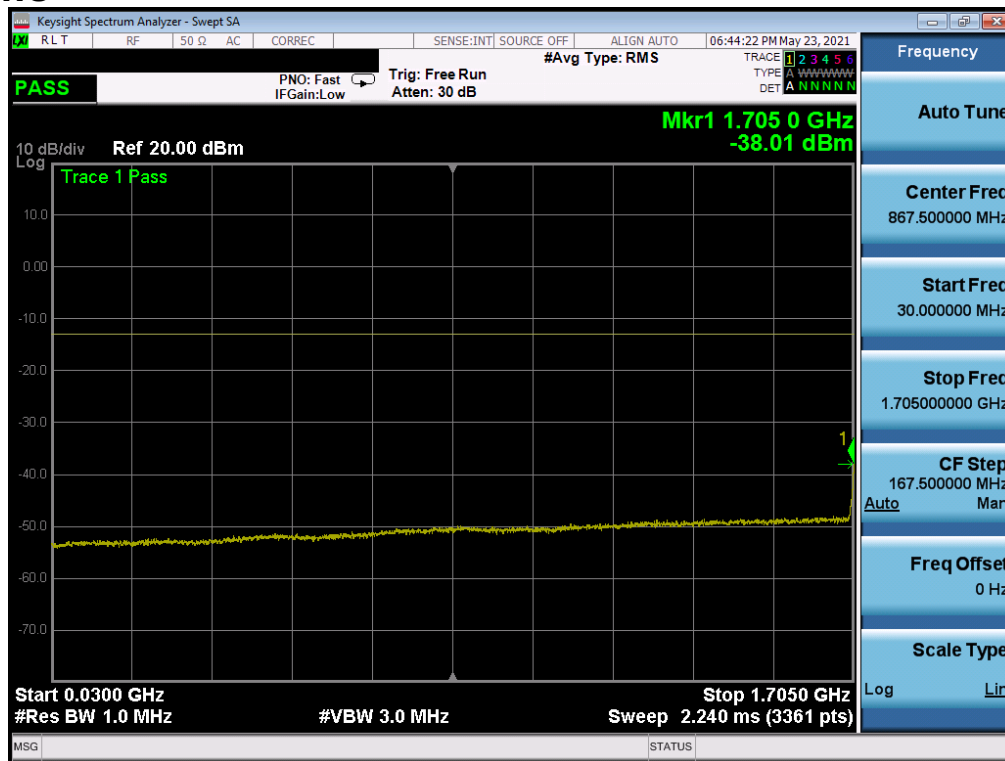
Plot 7-47. CSE WCDMA Ch. 1312- Low Channel)
