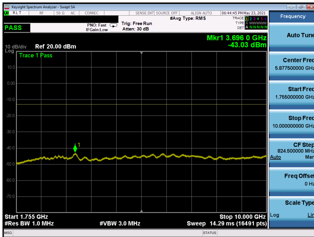
Plot 7-48. CSE (WCDMA Ch. 1312- Low Channel)
