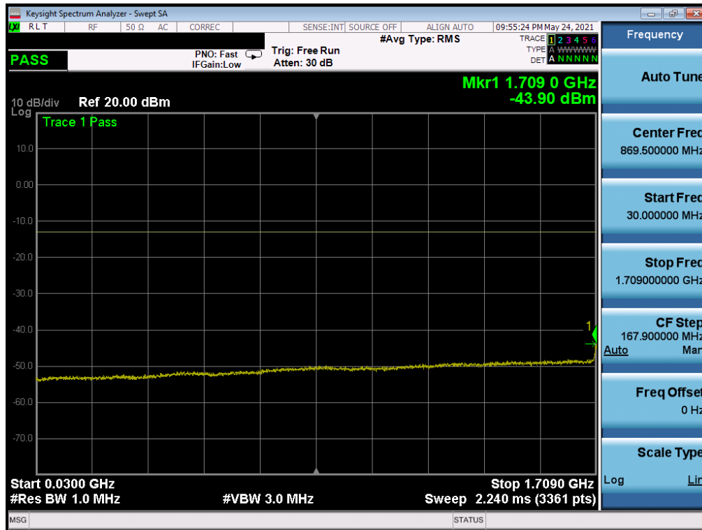
Plot 7-26. CSE (LTE Band 66/4 - 20MHz QPSK - RB Size 1, RB Offset 0 - Low Channel)
