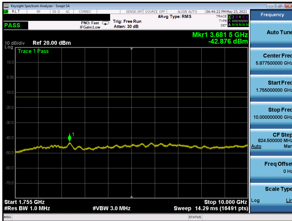
Plot 7-51. CSE (WCDMA Ch. 1413- Mid Channel)
