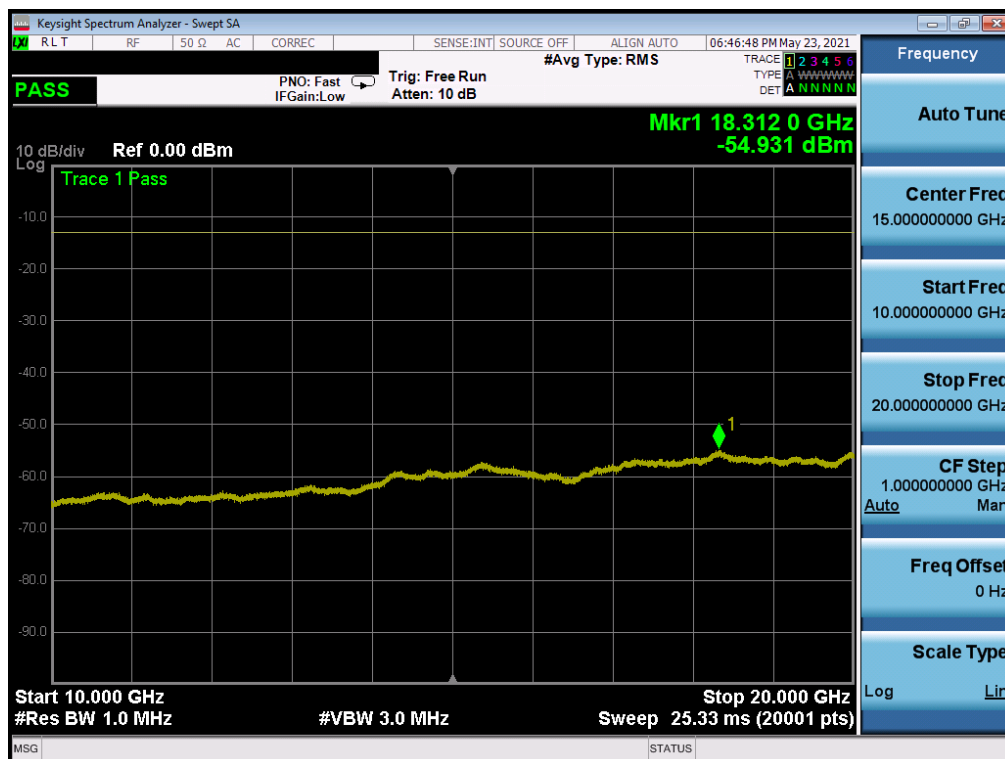
Plot 7-52. CSE (WCDMA Ch. 1413- Mid Channel)
