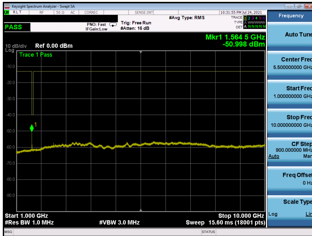
Plot 7-46. CSE (LTE Band 13 - 10MHz QPSK - RB Size 1, RB Offset 0)
