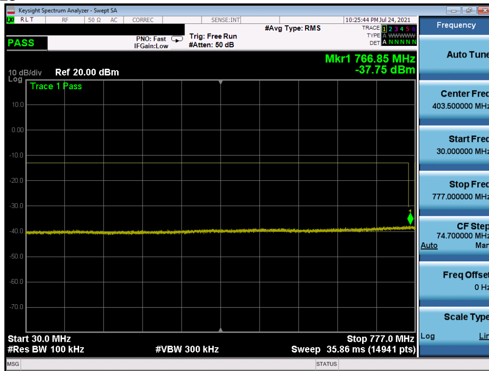
Plot 7-44. CSE (LTE Band 13 - 10MHz QPSK - RB Size 1, RB Offset 0)
