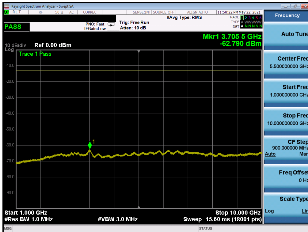
Plot 7-37. CSE (LTE Band 12/17 - 10MHz QPSK - RB Size 1, RB Offset 0 - Low Channel)
