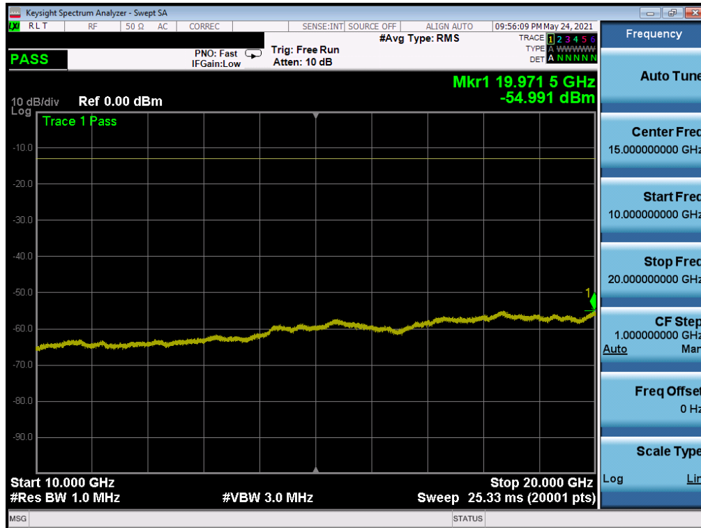
Plot 7-28. CSE (LTE Band 66/4 - 20MHz QPSK - RB Size 1, RB Offset 0 - Low Channel)
