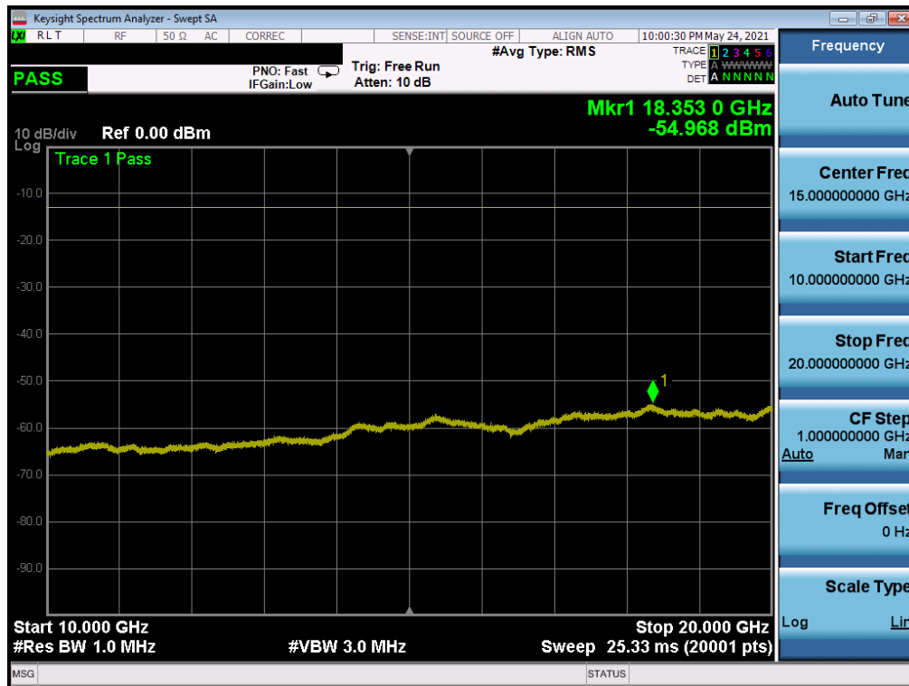
Plot 7-34. CSE (LTE Band 66/4 - 20MHz QPSK - RB Size 1, RB Offset 0 - High Channel)
