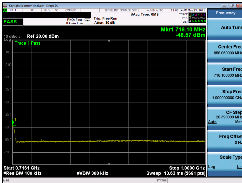
Plot 7-42. CSE (LTE Band 12/17 - 10MHz QPSK - RB Size 1, RB Offset 0 - High Channel)
