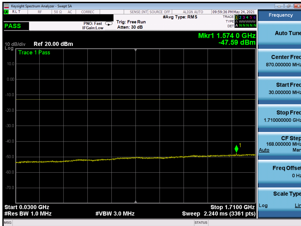
Plot 7-32. CSE (LTE Band 66/4 - 20MHz QPSK - RB Size 1, RB Offset 0 - High Channel)
