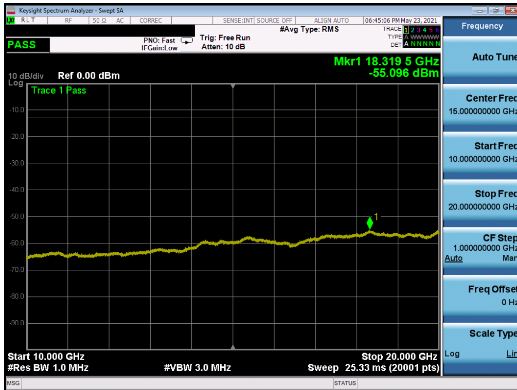
Plot 7-49. CSE (WCDMA Ch. 1312- Low Channel)
