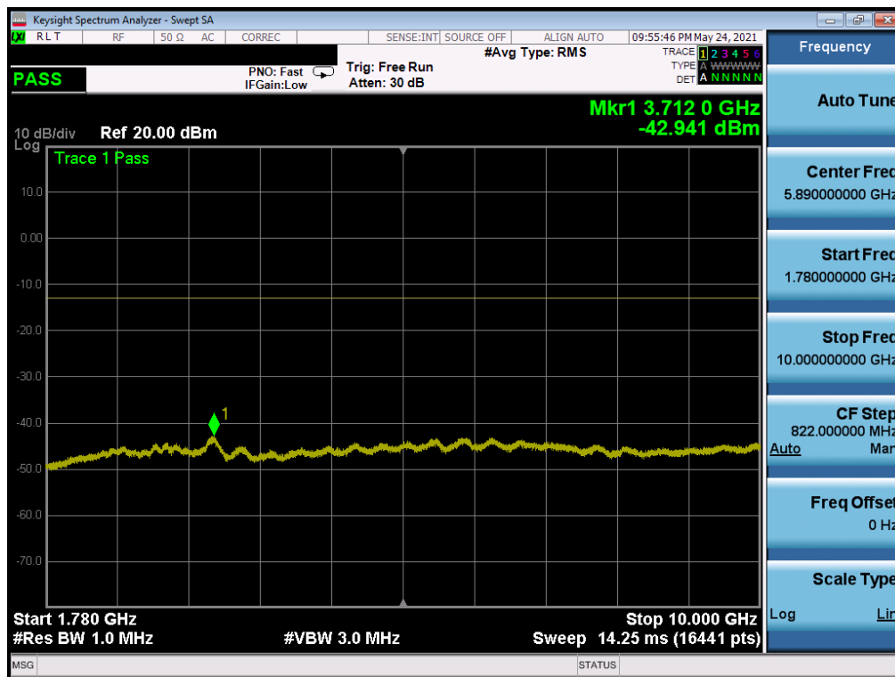
Plot 7-27. CSE (LTE Band 66/4 - 20MHz QPSK - RB Size 1, RB Offset 0 - Low Channel)
