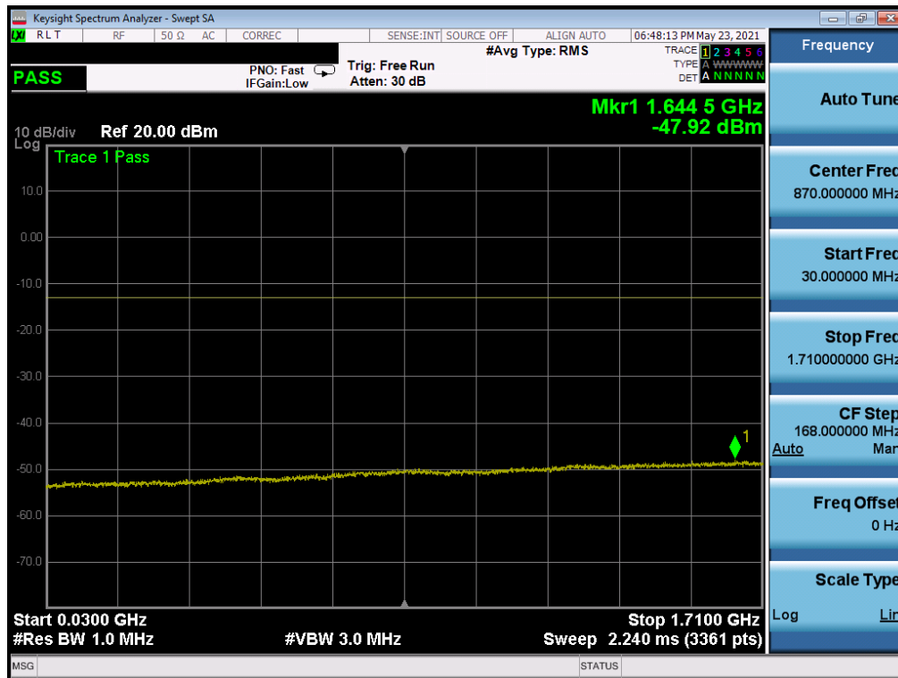
Plot 7-53. CSE (WCDMA Ch. 1513- High Channel)
