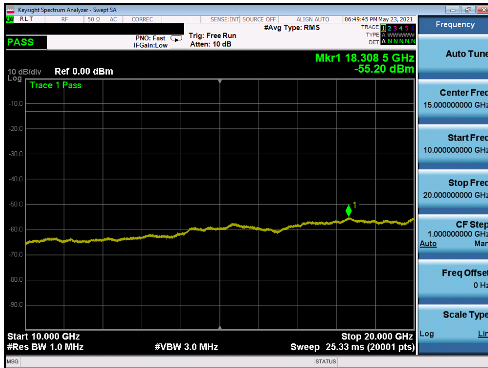
Plot 7-55. CSE (WCDMA Ch. 1513- High Channel)
