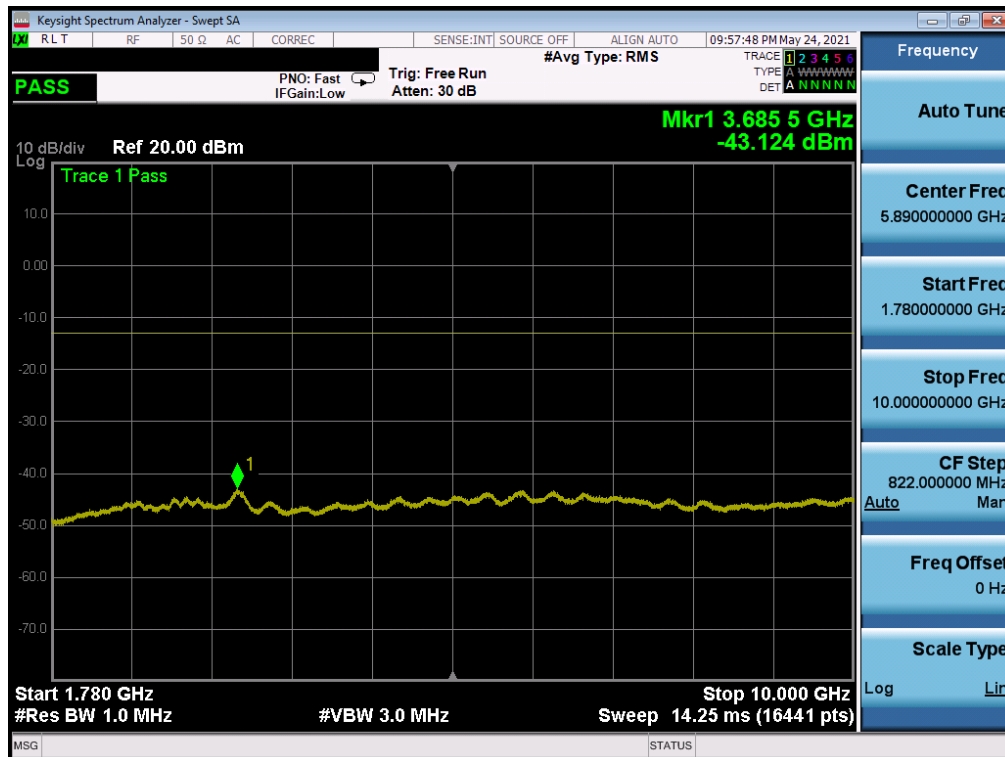
Plot 7-30. CSE (LTE Band 66/4 - 20MHz QPSK - RB Size 1, RB Offset 0 - Mid Channel)
