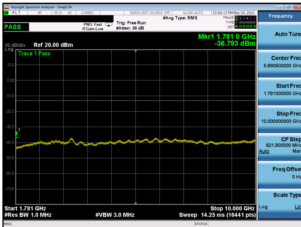
Plot 7-33. CSE (LTE Band 66/4 - 20MHz QPSK - RB Size 1, RB Offset 0 - High Channel)
