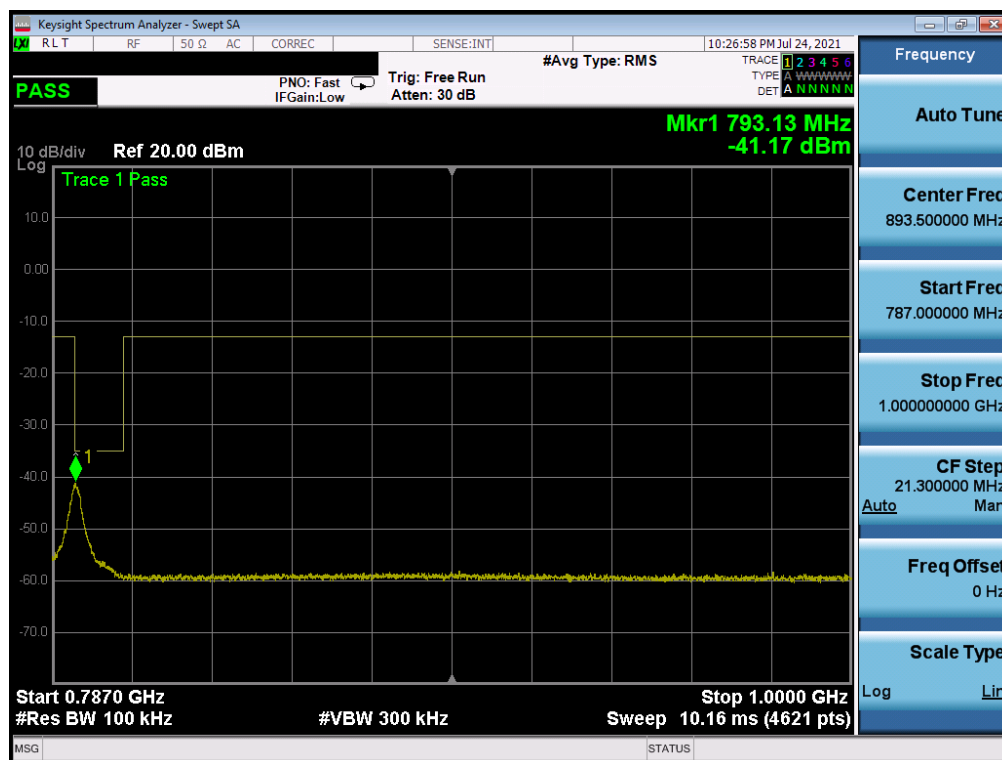
Plot 7-45. CSE (LTE Band 13 - 10MHz QPSK - RB Size 1, RB Offset 0)
