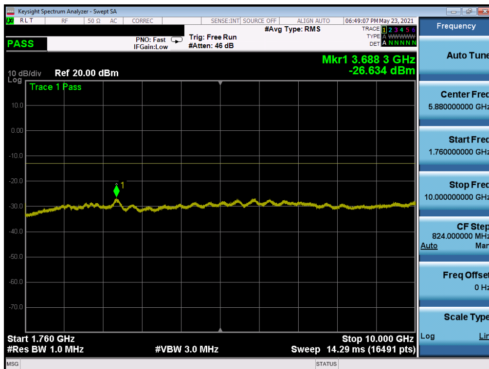
Plot 7-54. CSE (WCDMA Ch. 1513- High Channel)
