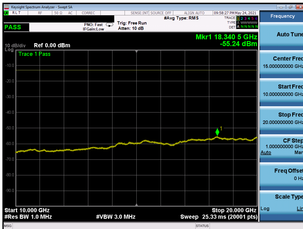
Plot 7-31. CSE (LTE Band 66/4 - 20MHz QPSK - RB Size 1, RB Offset 0 - Mid Channel)
