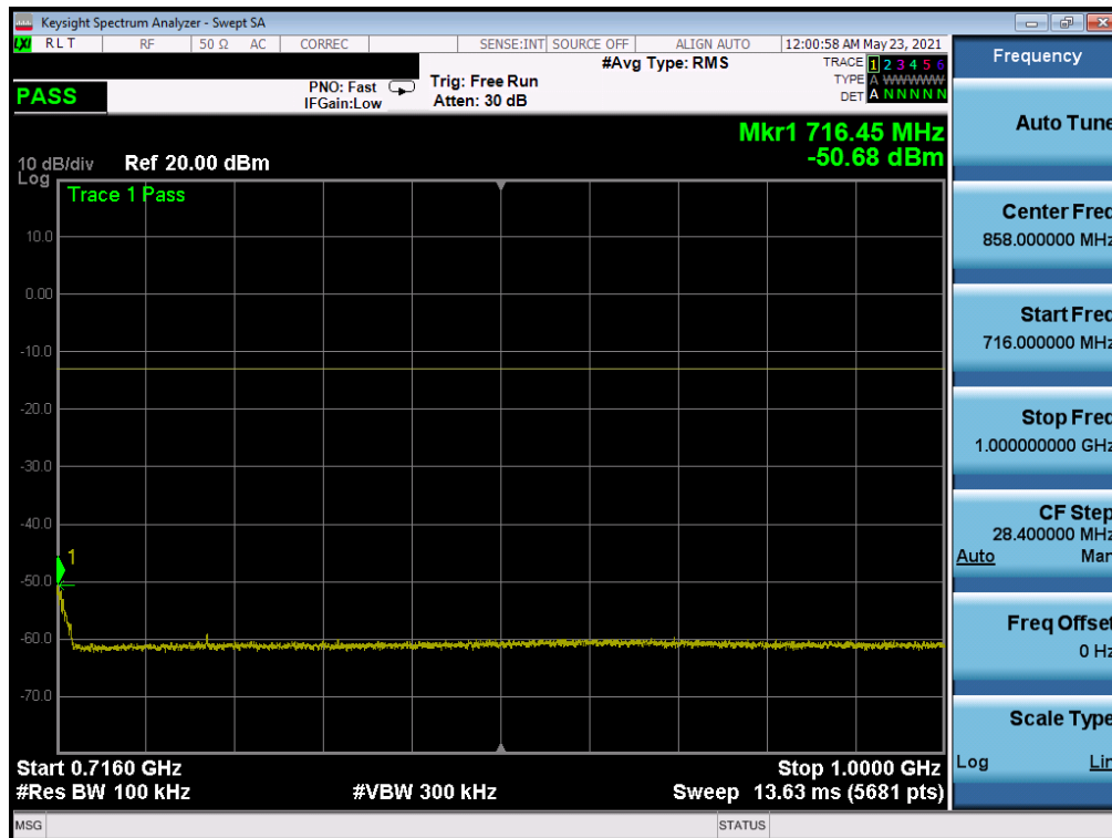
Plot 7-39. CSE Plot (LTE Band 12/17 - 10MHz QPSK - RB Size 1, RB Offset 0 - Mid Channel)
