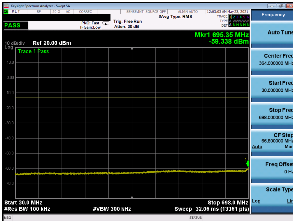
Plot 7-41. CSE (LTE Band 12/17 - 10MHz QPSK - RB Size 1, RB Offset 0 - High Channel)
