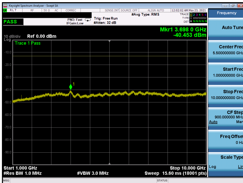
Plot 7-40. CSE (LTE Band 12/17 - 10MHz QPSK - RB Size 1, RB Offset 0 - Mid Channel)
