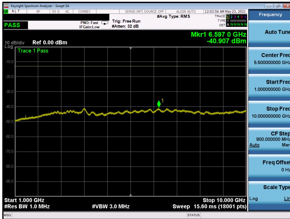
Plot 7-43. CSE (LTE Band 12/17 - 10MHz QPSK - RB Size 1, RB Offset 0 - High Channel)
