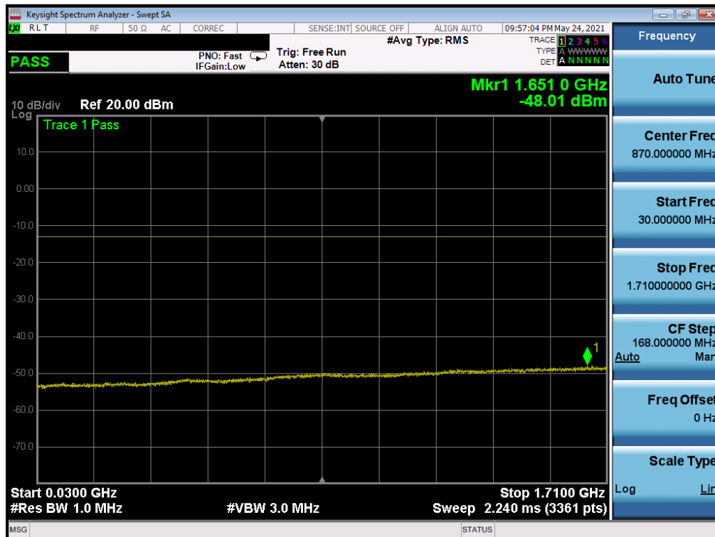
Plot 7-29. CSE (LTE Band 66/4 - 20MHz QPSK - RB Size 1, RB Offset 0 - Mid Channel)
