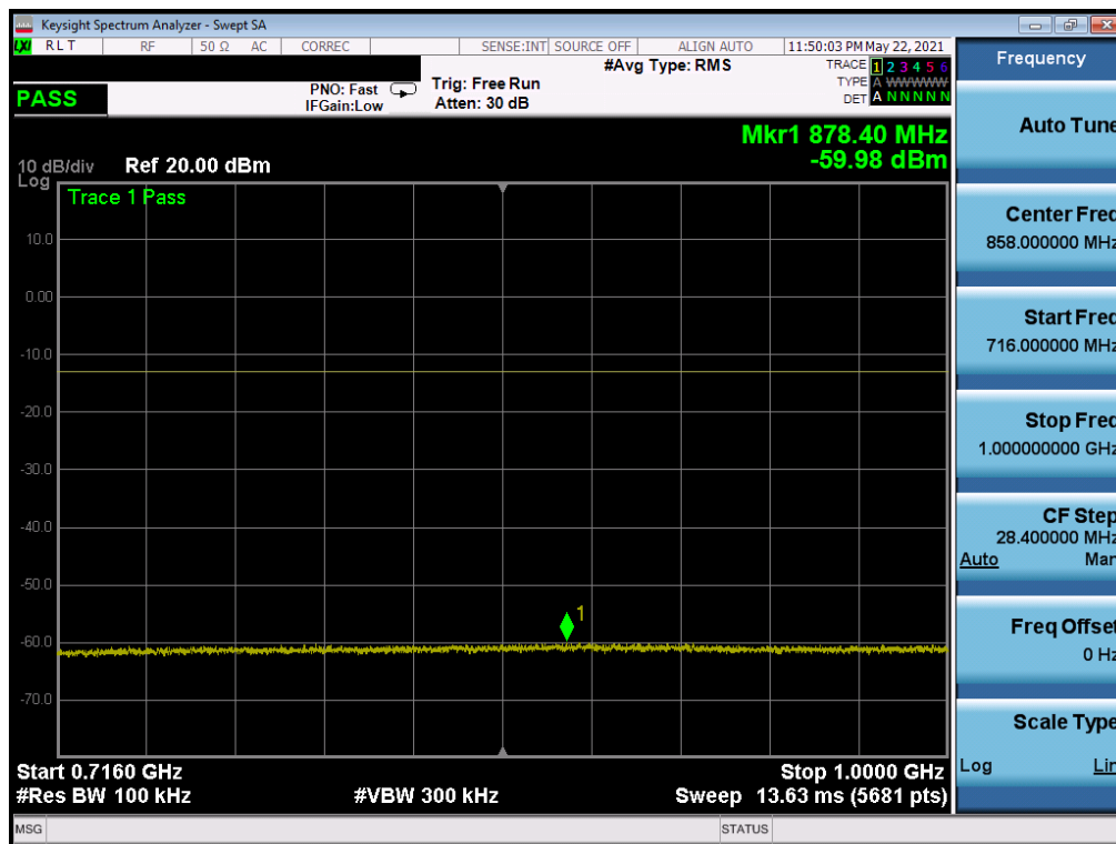
Plot 7-36. CSE (LTE Band 12/17 - 10MHz QPSK - RB Size 1, RB Offset 0 - Low Channel)
