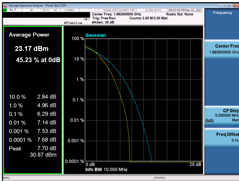
Plot 7-103. PAR Plot (LTE Band 25 - 10MHz 16-QAM - Full RB Configuration)
