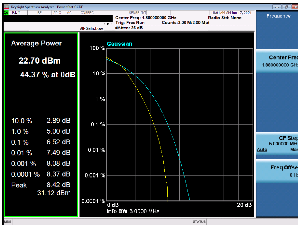
Plot 7-87. PAR Plot (LTE Band 2 - 3MHz 16-QAM - Full RB Configuration)
