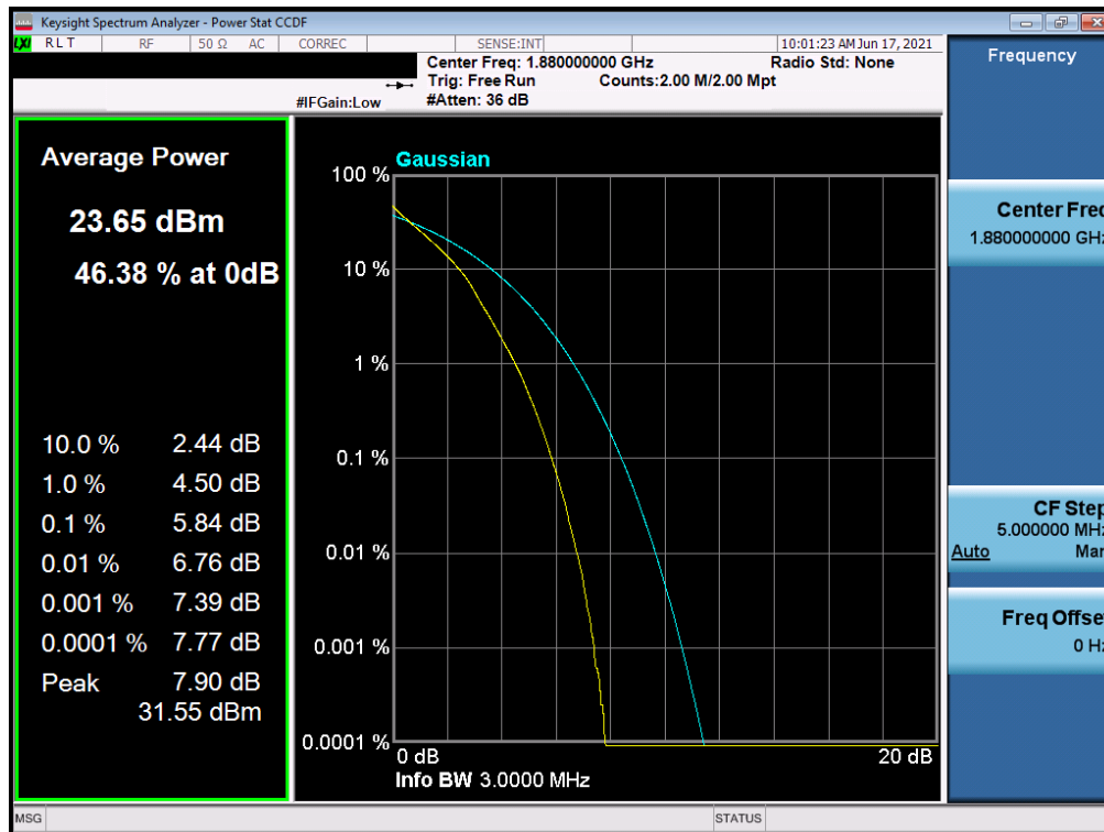
Plot 7-86. PAR Plot (LTE Band 2 - 3MHz QPSK - Full RB Configuration)
