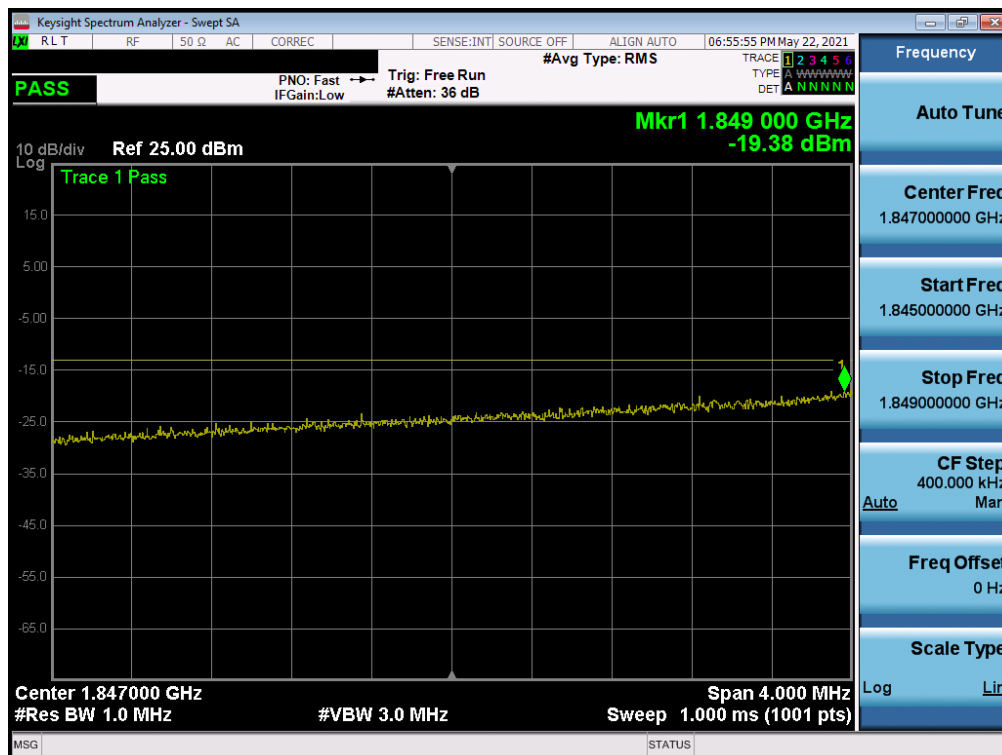
Plot 7-69. Extended Lower Band Edge Plot (LTE Band 25 – 10MHz QPSK – Full RB Configuration)
