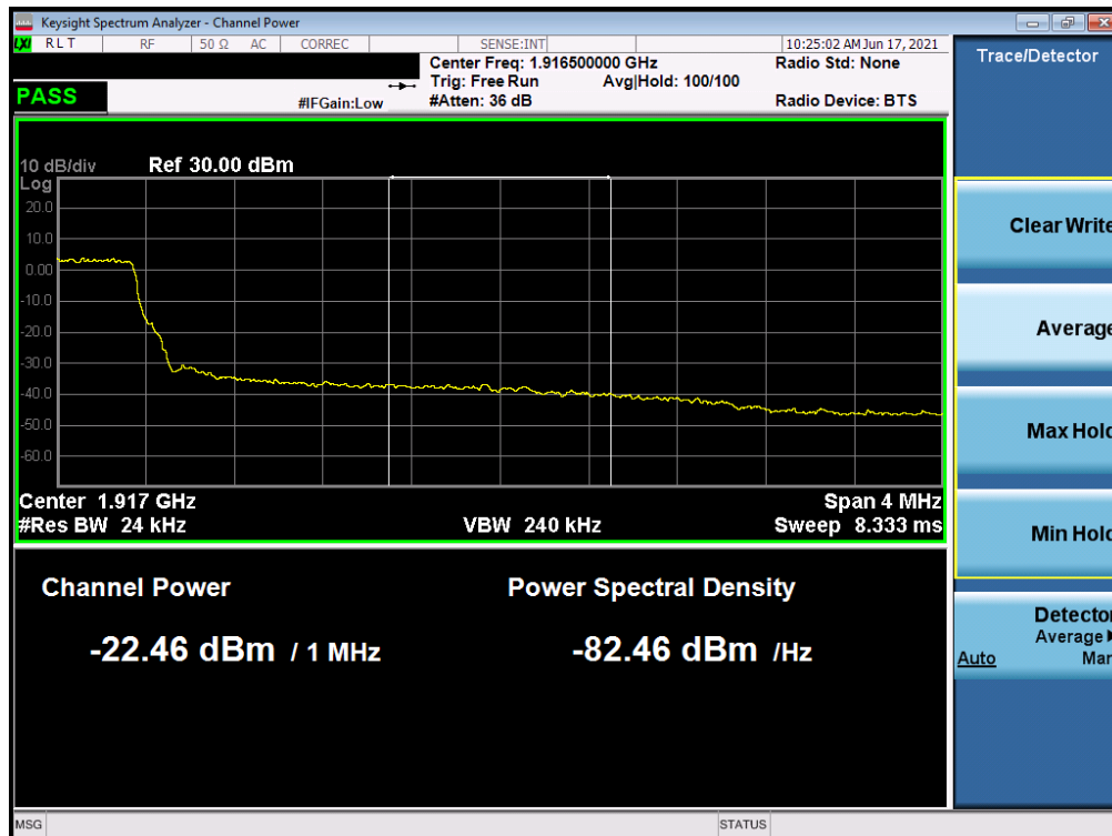
Plot 7-63. Extended Upper Band Edge Plot (LTE Band 25 – 3MHz QPSK – Full RB Configuration)
