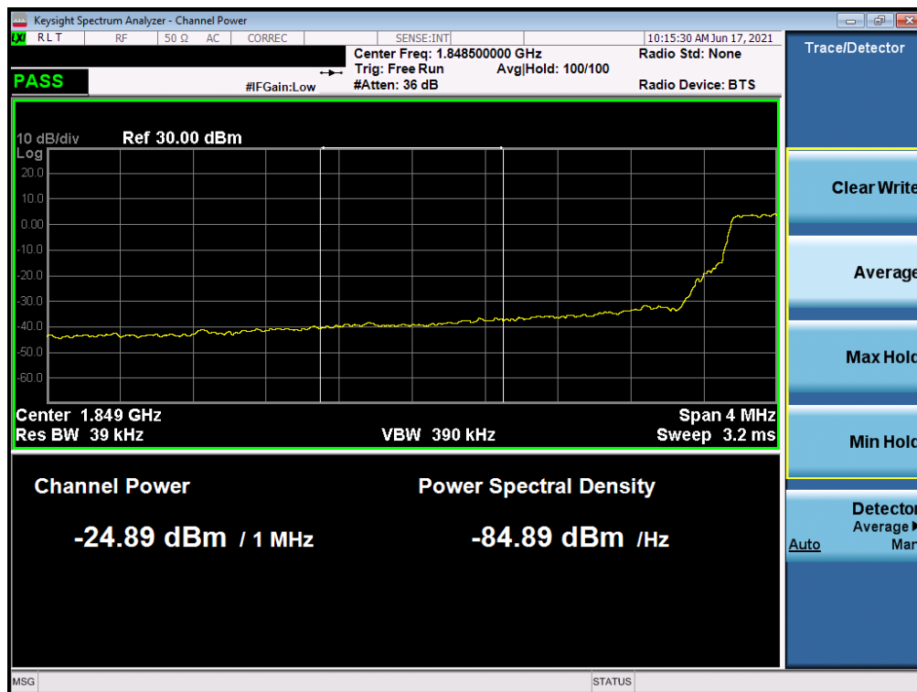
Plot 7-65. Extended Lower Band Edge Plot (LTE Band 25 – 5MHz QPSK – Full RB Configuration)
