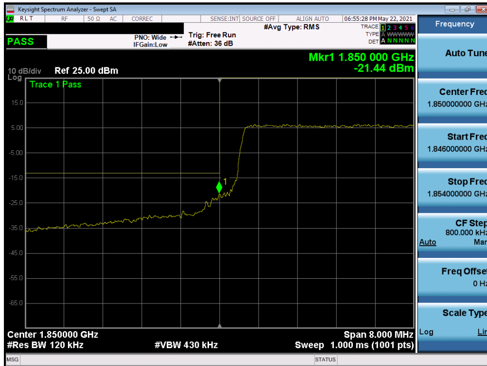
Plot 7-68. Lower Band Edge Plot (LTE Band 25 – 10MHz QPSK – Full RB Configuration)
