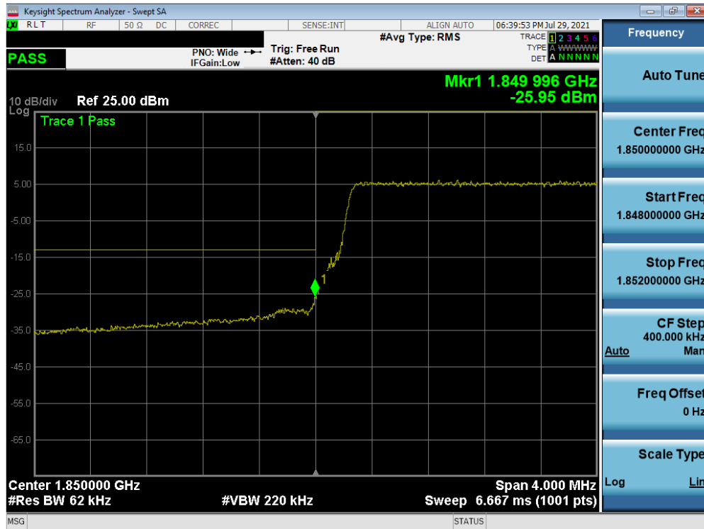
Plot 7-64. Lower Band Edge Plot (LTE Band 25 – 5MHz QPSK – Full RB Configuration)
