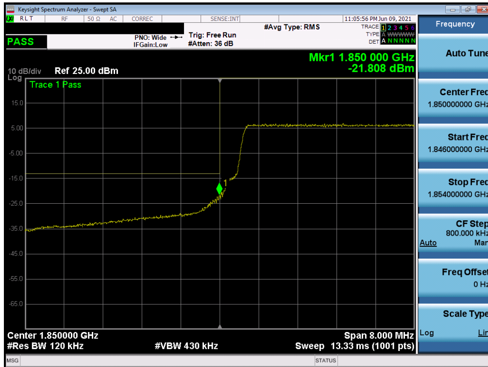
Plot 7-44. Lower Band Edge Plot (LTE Band 2 – 10MHz QPSK – Full RB Configuration)
