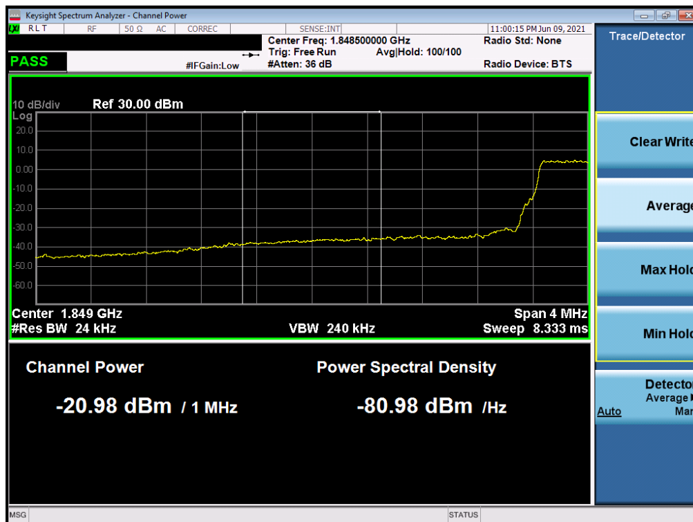
Plot 7-37. Extended Lower Band Edge Plot (LTE Band 2 – 3MHz QPSK – Full RB Configuration)
