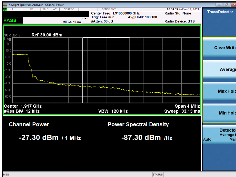
Plot 7-59. Extended Upper Band Edge Plot (LTE Band 25 – 1.4MHz QPSK – Full RB Configuration)
