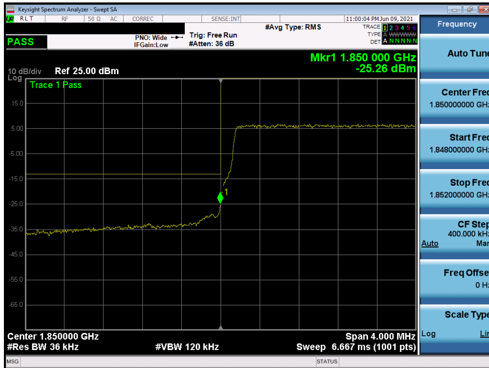
Plot 7-36. Lower Band Edge Plot (LTE Band 2 – 3MHz QPSK – Full RB Configuration)
