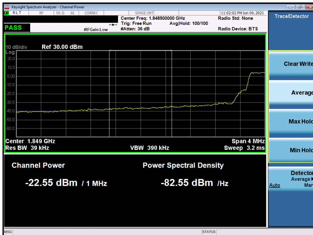
Plot 7-41. Extended Lower Band Edge Plot (LTE Band 2 – 5MHz QPSK – Full RB Configuration)
