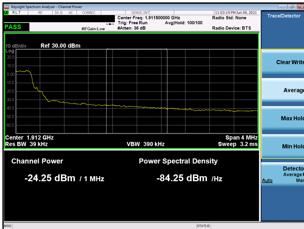
Plot 7-43. Extended Upper Band Edge Plot (LTE Band 2 – 5MHz QPSK – Full RB Configuration)
