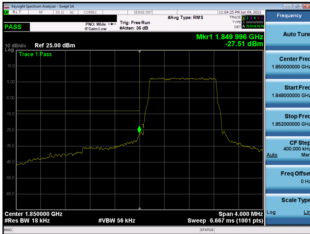
Plot 7-32. Lower Band Edge Plot (LTE Band 2 – 1.4MHz QPSK – Full RB Configuration)
