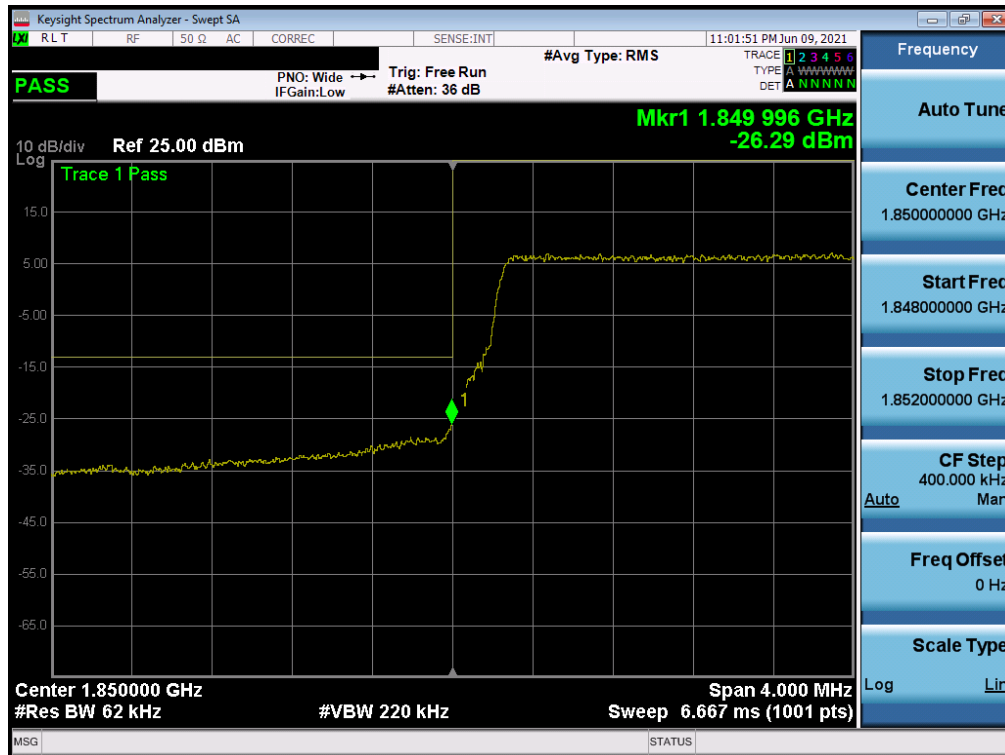
Plot 7-40. Lower Band Edge Plot (LTE Band 2 – 5MHz QPSK – Full RB Configuration)
