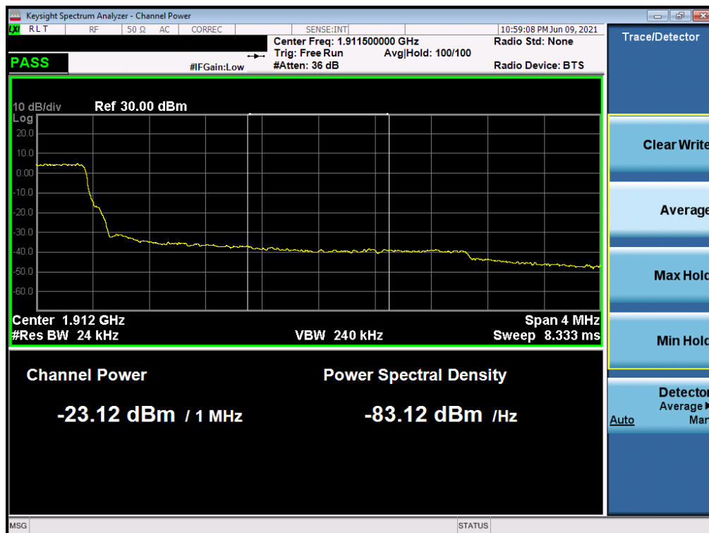
Plot 7-39. Extended Upper Band Edge Plot (LTE Band 2 – 3MHz QPSK – Full RB Configuration)
