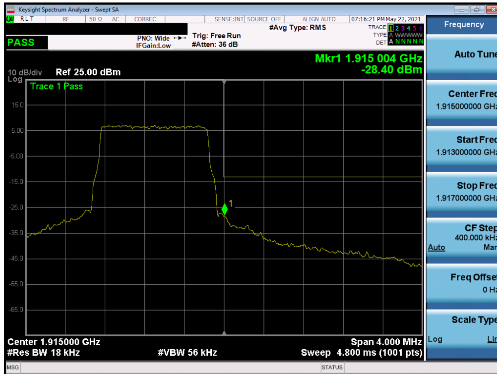
Plot 7-58. Upper Band Edge Plot (LTE Band 25 – 1.4MHz QPSK – Full RB Configuration)
