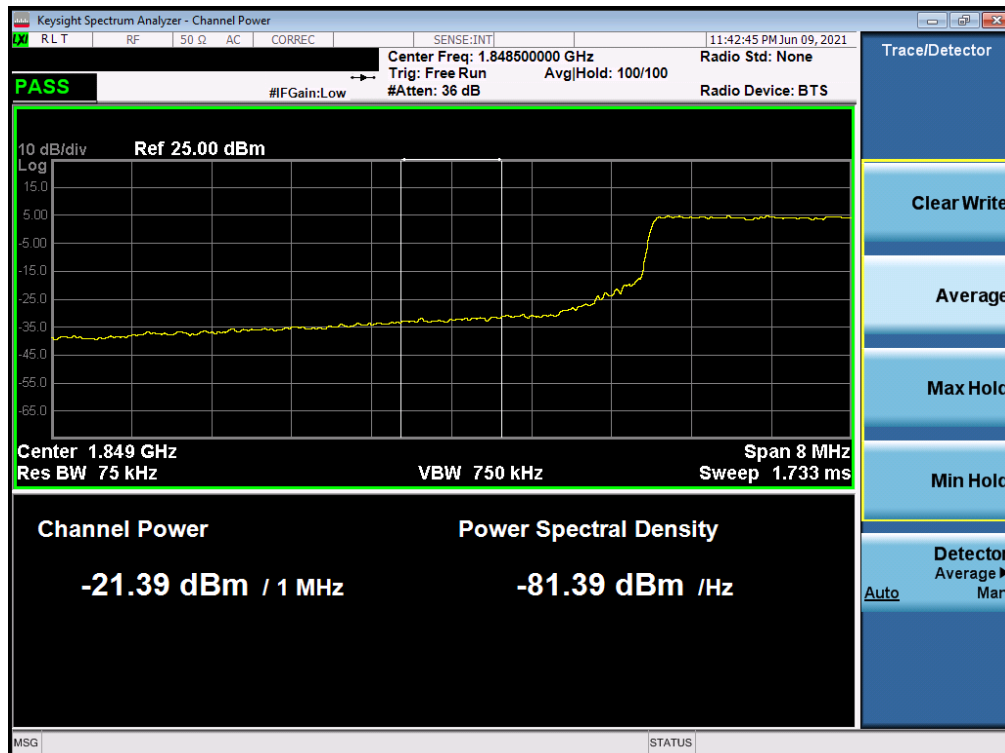
Plot 7-45. Extended Lower Band Edge Plot (LTE Band 2 – 10MHz QPSK – Full RB Configuration)
