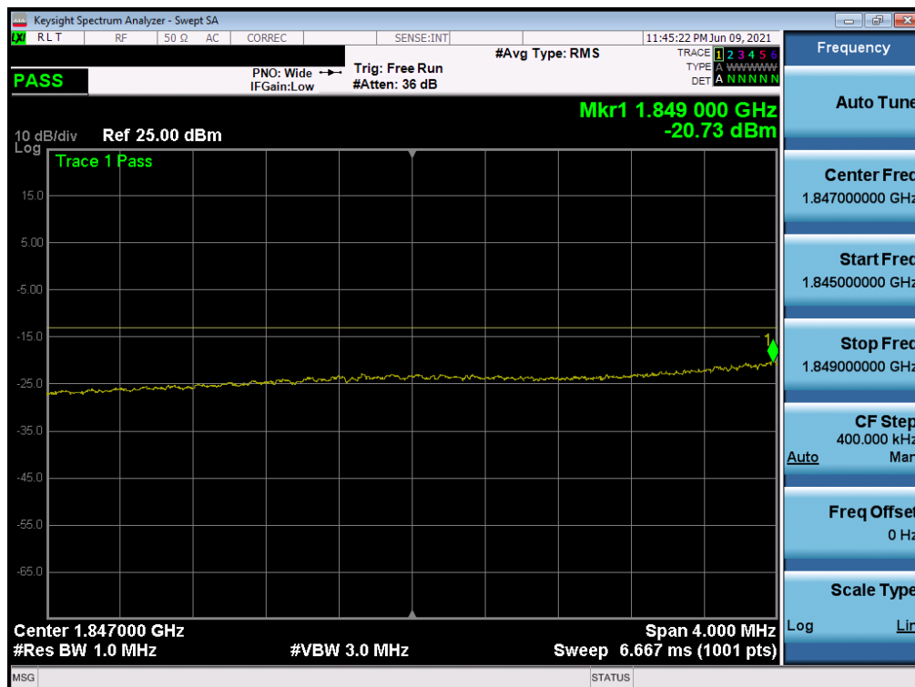
Plot 7-49. Extended Lower Band Edge Plot (LTE Band 2 – 15MHz QPSK – Full RB Configuration)
