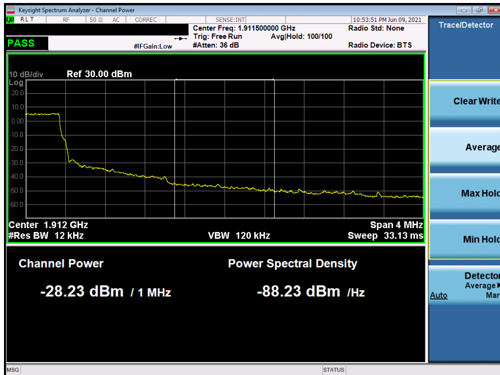
Plot 7-35. Extended Upper Band Edge Plot (LTE Band 2 – 1.4MHz QPSK – Full RB Configuration)
