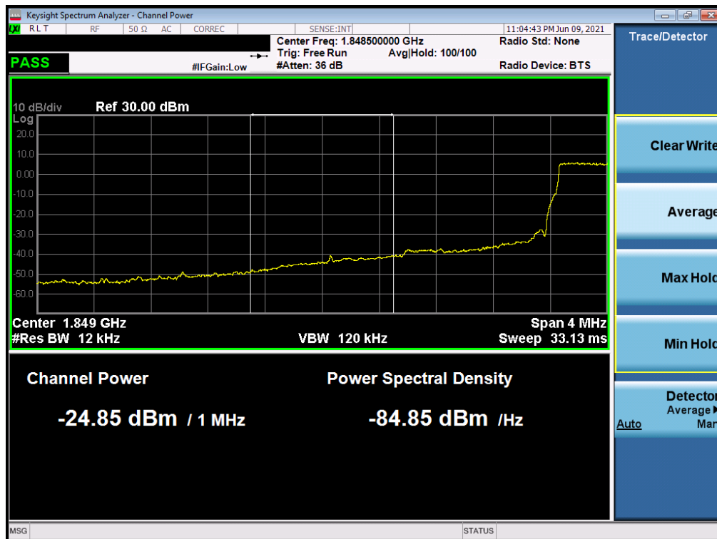
Plot 7-33. Extended Lower Band Edge Plot (LTE Band 2 – 1.4MHz QPSK – Full RB Configuration)
