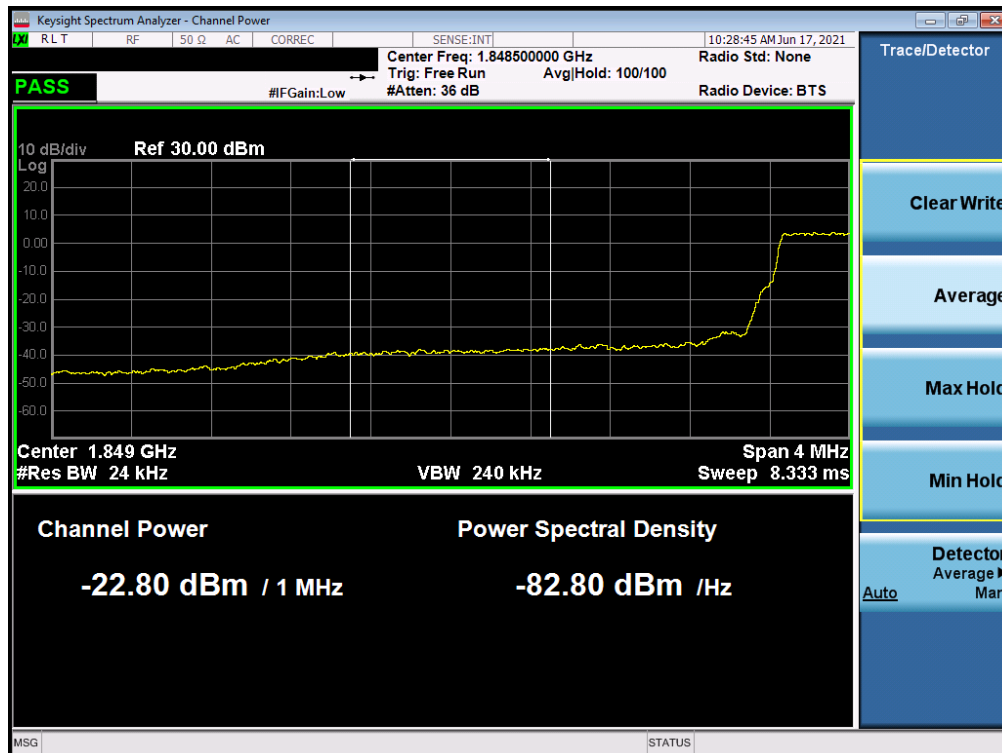
Plot 7-61. Extended Lower Band Edge Plot (LTE Band 25 – 3MHz QPSK – Full RB Configuration)
