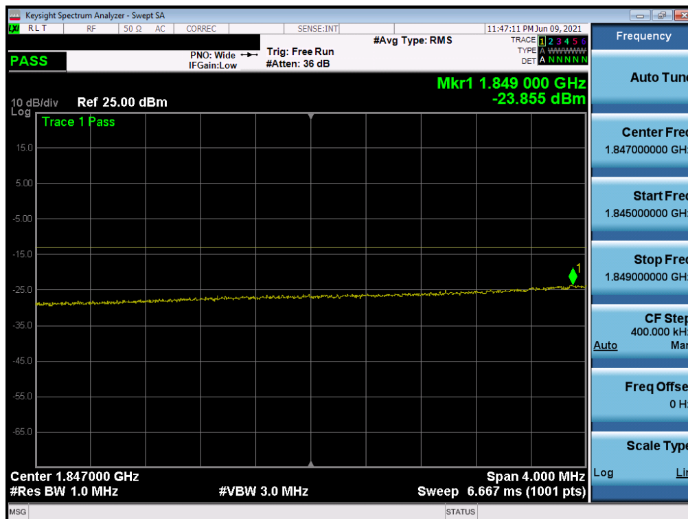
Plot 7-53. Extended Lower Band Edge Plot (LTE Band 2 – 20MHz QPSK – Full RB Configuration)
