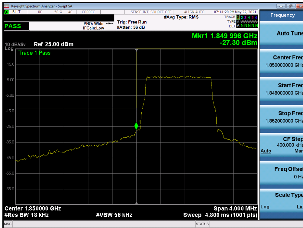
Plot 7-56. Lower Band Edge Plot (LTE Band 25 – 1.4MHz QPSK – Full RB Configuration)
