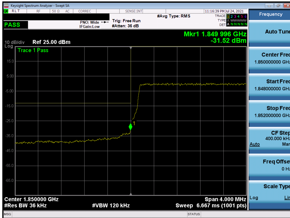
Plot 7-60. Lower Band Edge Plot (LTE Band 25 – 3MHz QPSK – Full RB Configuration)
