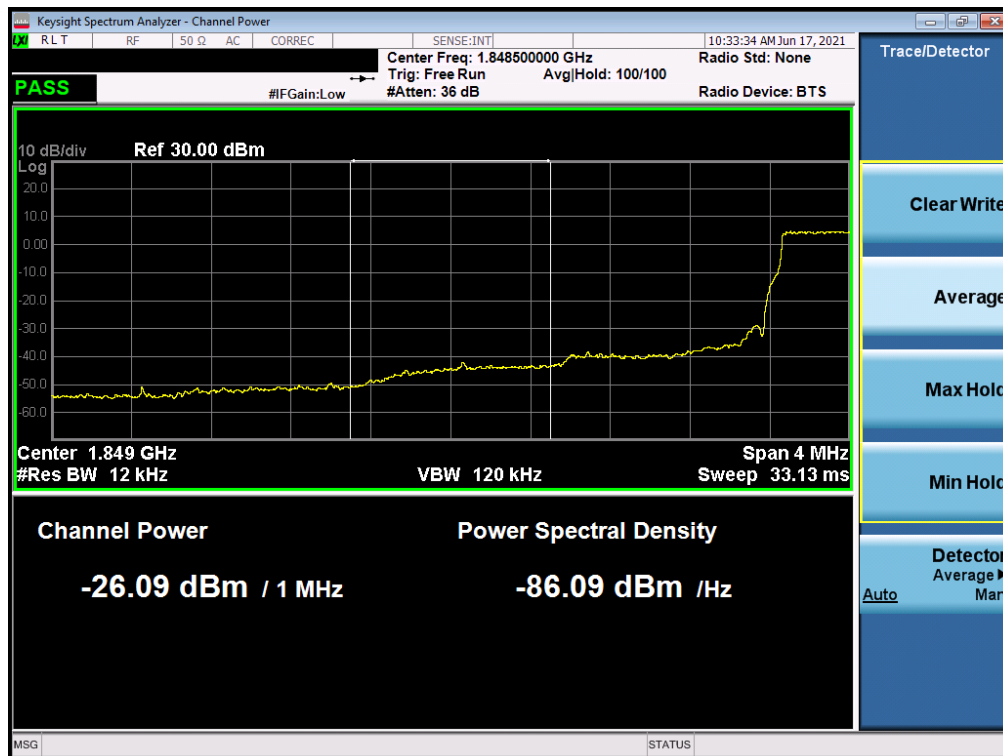
Plot 7-57. Extended Lower Band Edge Plot (LTE Band 25 – 1.4MHz QPSK – Full RB Configuration)
