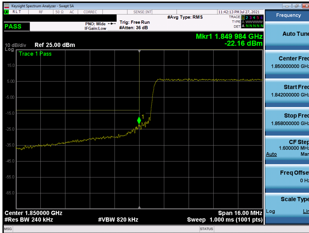
Plot 7-52. Lower Band Edge Plot (LTE Band 2 – 20MHz QPSK – Full RB Configuration)
