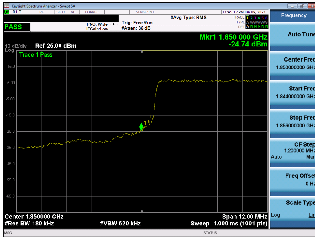
Plot 7-48. Lower Band Edge Plot (LTE Band 2 – 15MHz QPSK – Full RB Configuration)
