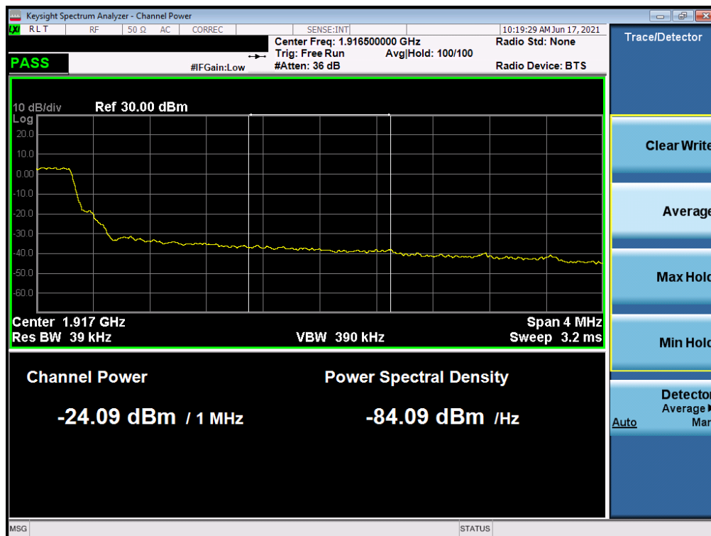
Plot 7-67. Extended Upper Band Edge Plot (LTE Band 25 – 5MHz QPSK – Full RB Configuration)
