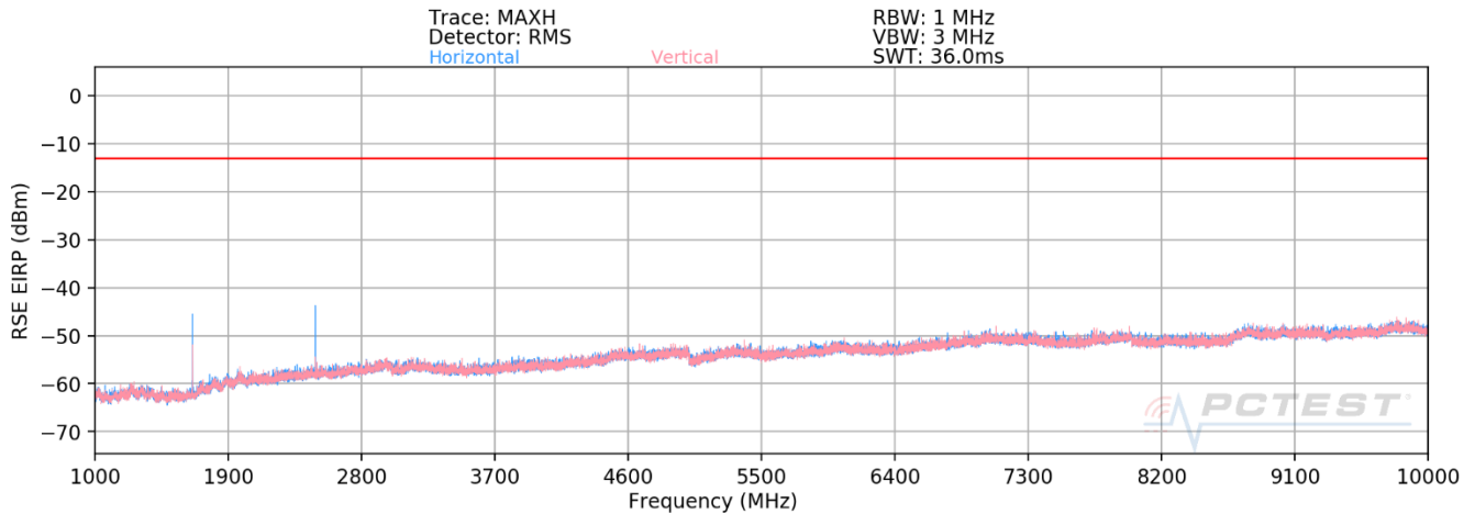
Plot 7-47. Antenna BCM Radiated Spurious Emission Above 1GHz (LTE Band 26/5)
