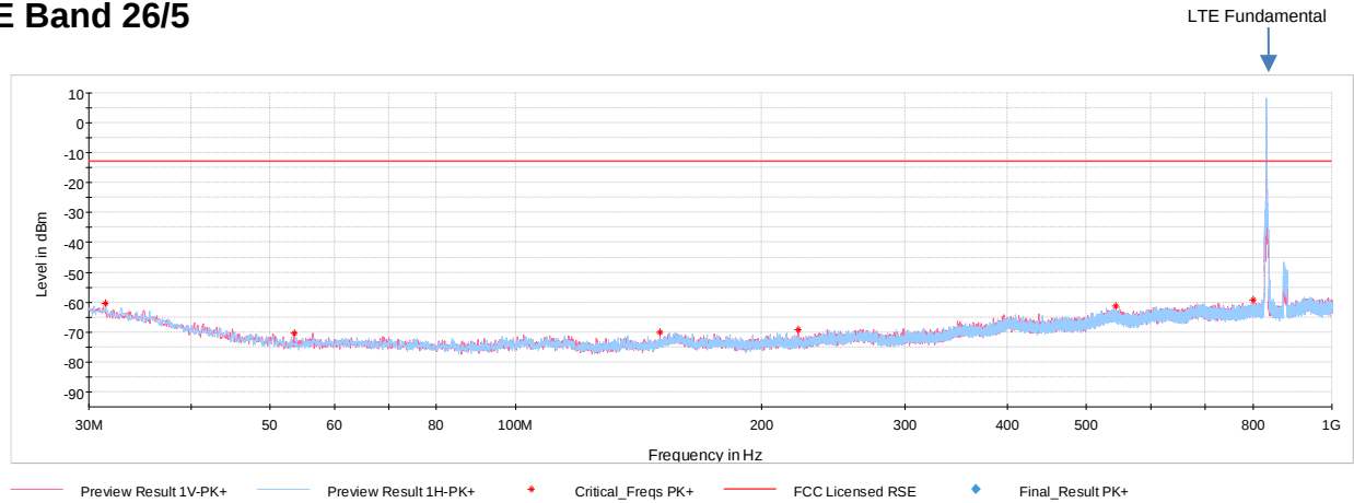
Plot 7-46. Antenna BCM Radiated Spurious Emission Below 1GHz (LTE Band 26/5)
