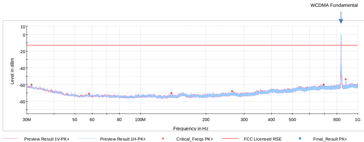
Plot 7-48. Antenna BCM Radiated Spurious Emission below 1GHz (WCDMA Cell)
