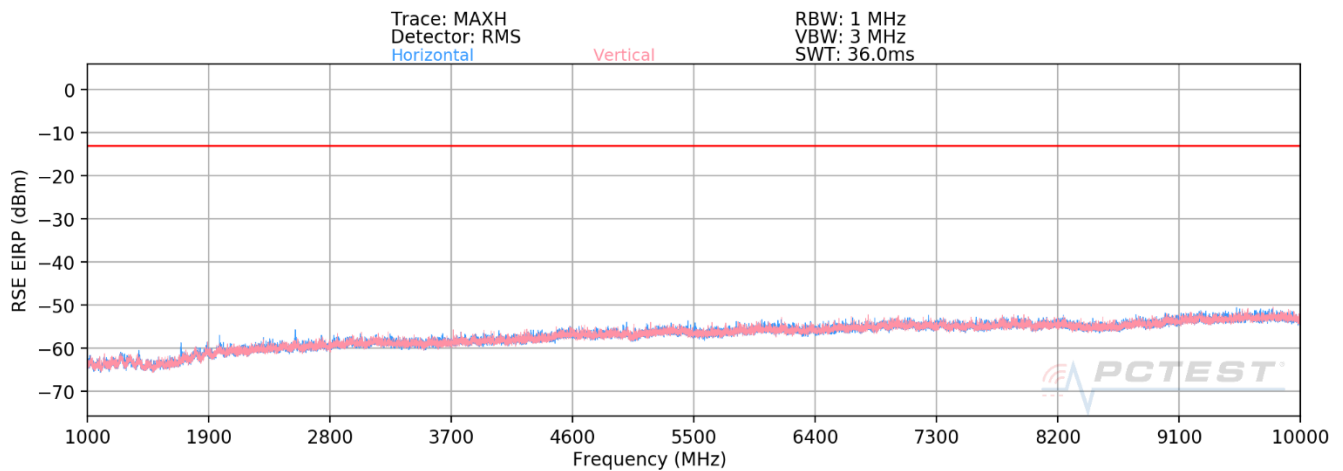
Plot 7-49. Antenna BCM Radiated Spurious Emission above 1GHz (WCDMA Cell)
