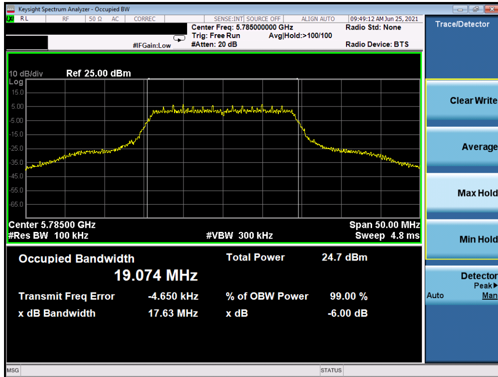
Plot 7-11. 99% OBW and 6dB Bandwidth Plot (20MHz BW 802.11n (UNII Band 3) – Ch. 157)
