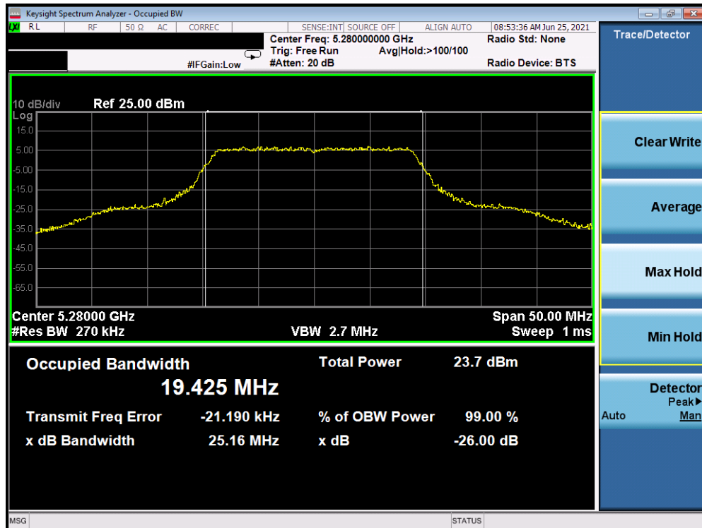
Plot 7-5. 99% OBW and 26dB Bandwidth (20MHz BW 802.11n (UNII Band 2A) – Ch. 56)
