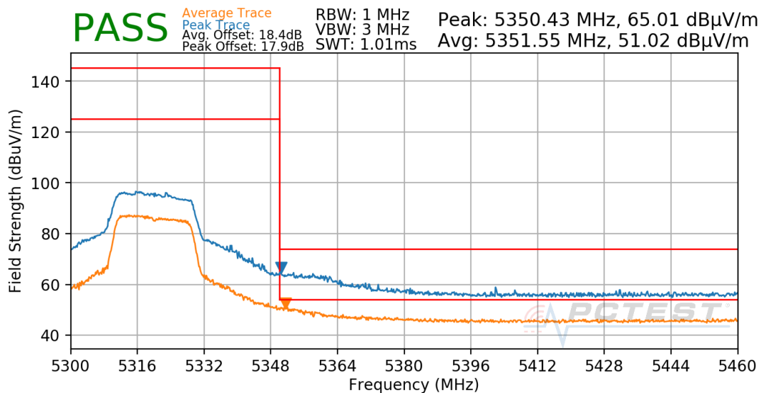
Plot 7-45. Radiated Upper Band Edge Plot (UNII Band 2A)
