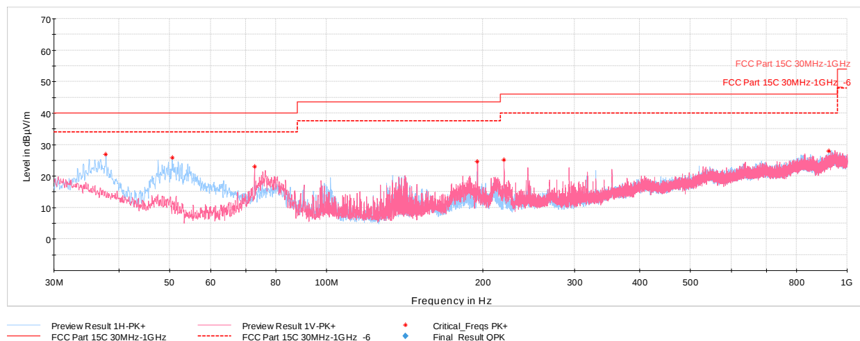
Plot 7-56. Radiated Spurious Emissions below 1GHz (802.11n – UNII 2C Ch. 149) with AC/DC Adaptor & Magnetic Charger
