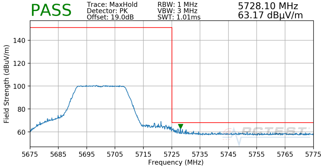
Plot 7-50. Radiated Upper Band Edge Plot (Peak – UNII Band 2C)
