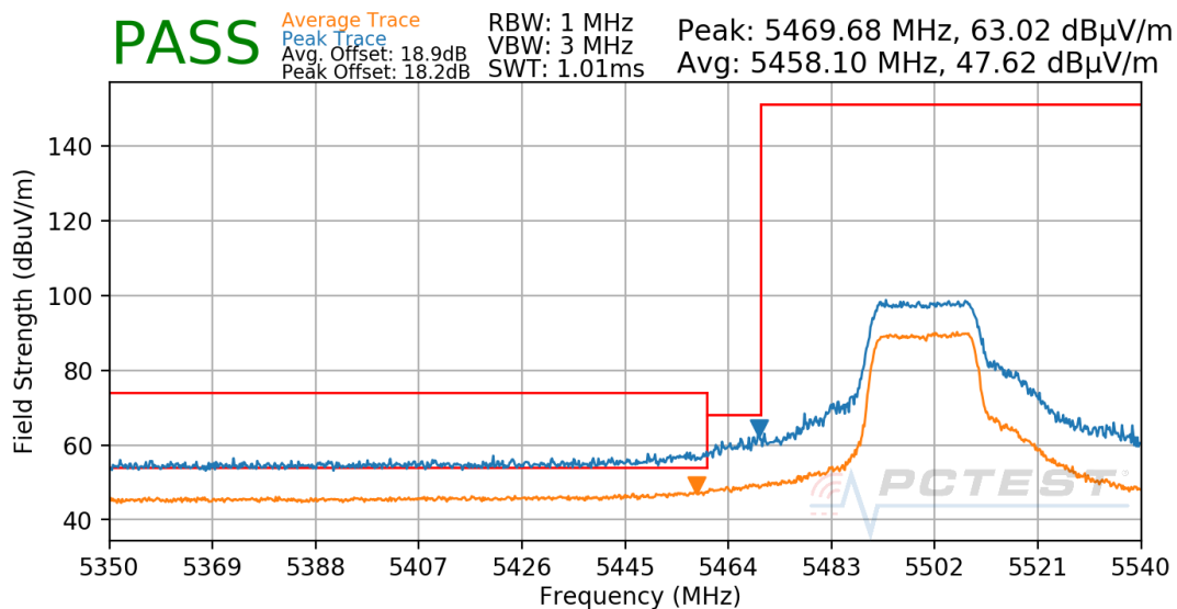
Plot 7-47. Radiated Lower Band Edge Plot (UNII Band 2C)
