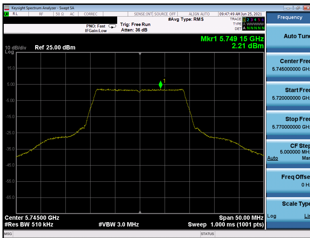
Plot 7-22. Power Spectral Density Plot (20MHz BW 802.11n (UNII Band 3) – Ch. 149)
