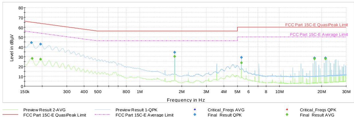
Plot 7-58. AC Line Conducted Plot with 802.11n UNII Band 2C – Ch.149 (L1) with AC/DC Adaptor & Magnetic Charger
