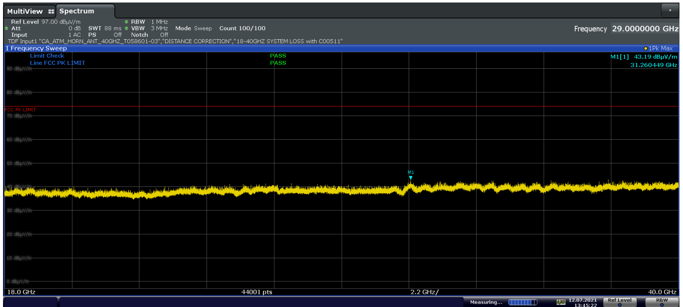
Plot 7-36. Radiated Spurious Emissions 18GHz - 40GHz – V Polarity (802.11n Ch 149)
