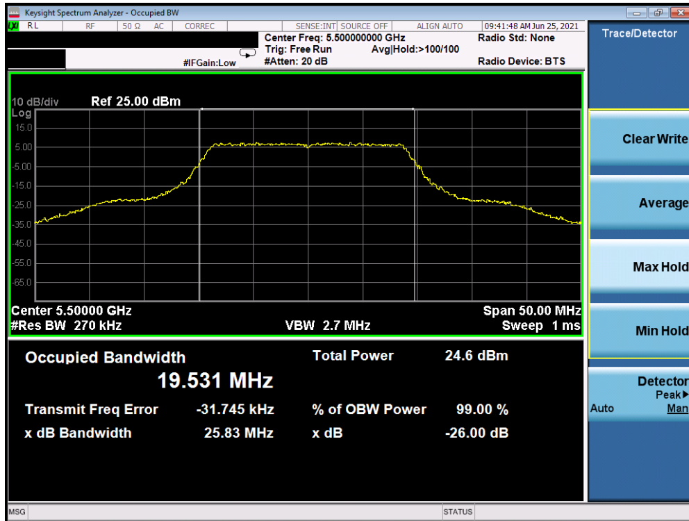
Plot 7-7. 99% OBW and 26dB Bandwidth (20MHz BW 802.11n (UNII Band 2C) – Ch. 100)
