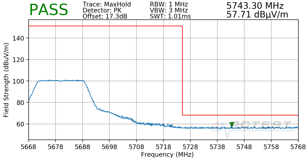
Plot 7-48. Radiated Upper Band Edge Plot (Peak – UNII Band 2C)
