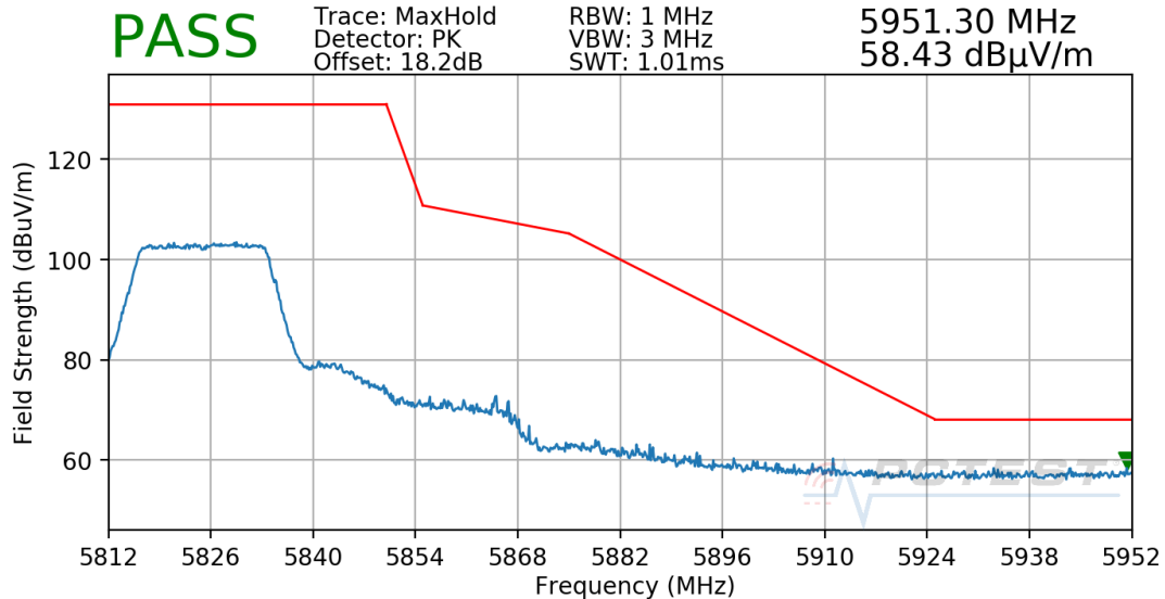
Plot 7-54. Radiated Upper Band Edge Plot (Peak – UNII Band 3)
