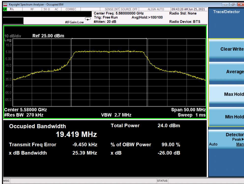
Plot 7-8. 99% OBW and 26dB Bandwidth (20MHz BW 802.11n (UNII Band 2C) – Ch. 116)
