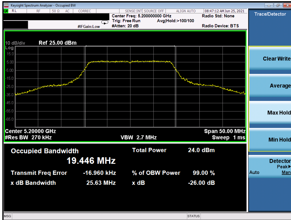
Plot 7-2. 99% OBW and 26dB Bandwidth (20MHz BW 802.11n (UNII Band 1) – Ch. 40)
