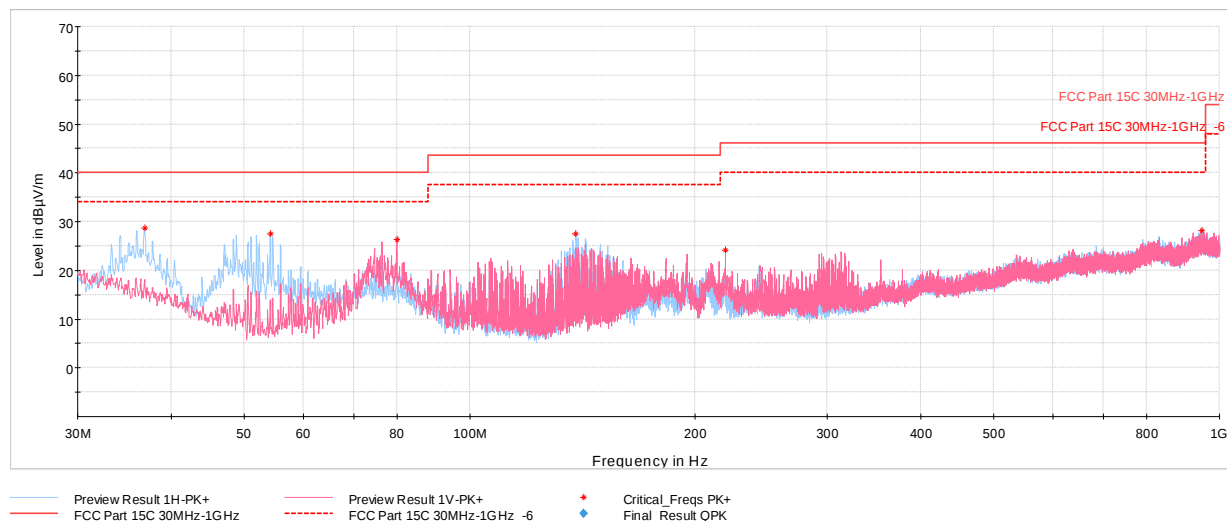
Plot 7-57. Radiated Spurious Emissions – Simultaneous Transmission below 1GHz with AC/DC Adaptor & Magnetic Charger
