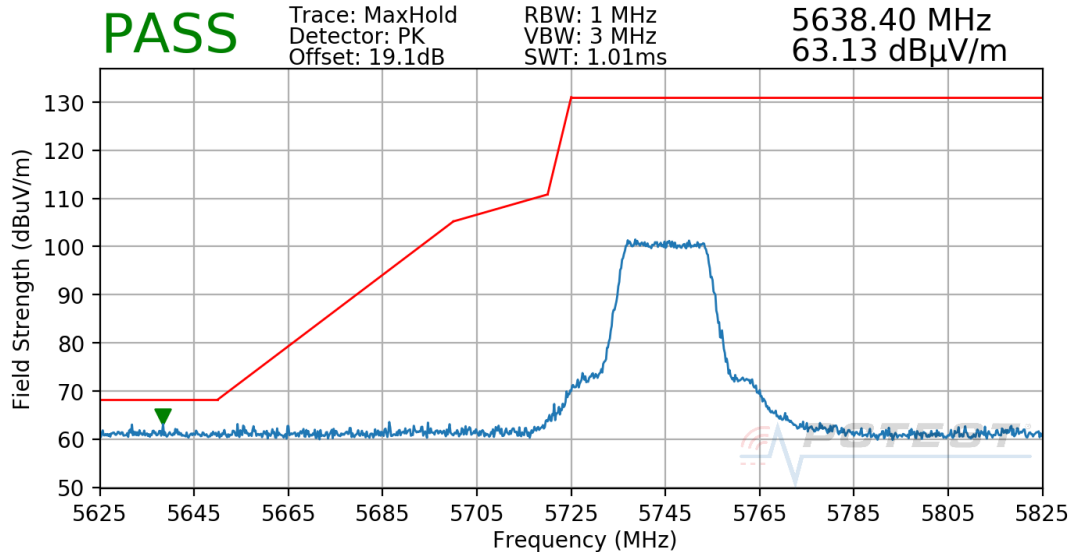
Plot 7-52. Radiated Lower Band Edge Plot (Peak – UNII Band 3)
