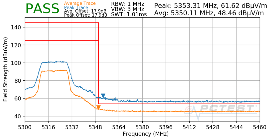
Plot 7-44. Radiated Upper Band Edge Plot (UNII Band 2A)
