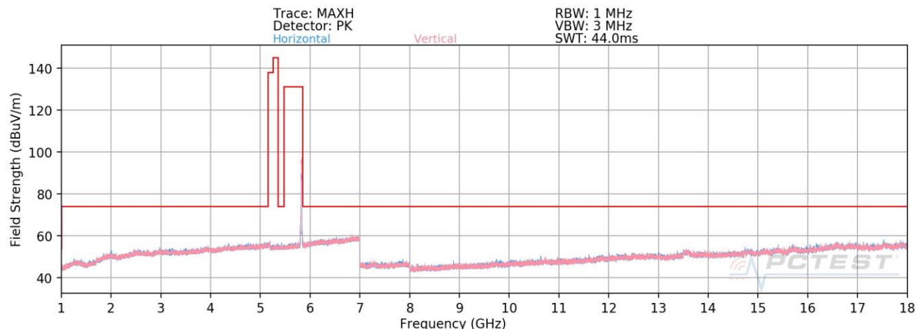
Plot 7-38. Radiated Spurious Emissions above 1GHz (802.11n – UNII 3 Ch. 165)
