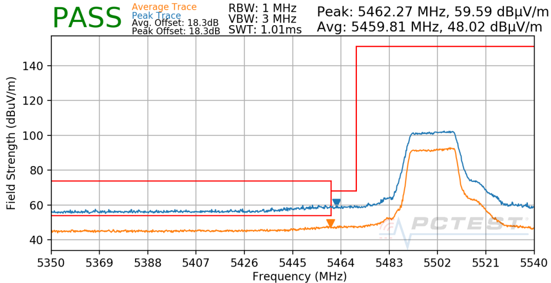
Plot 7-46. Radiated Lower Band Edge Plot (UNII Band 2C)
