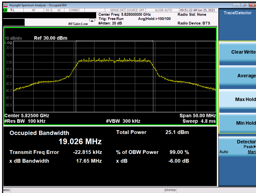
Plot 7-12. 99% OBW and 6dB Bandwidth Plot (20MHz BW 802.11n (UNII Band 3) – Ch. 165)
