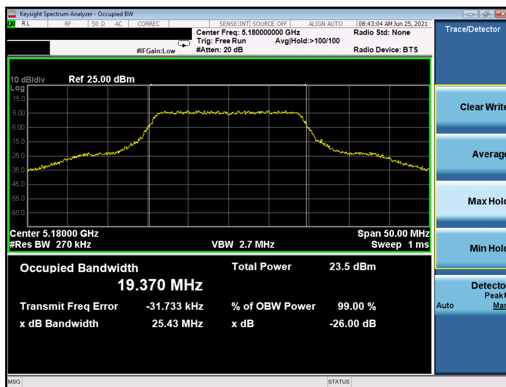
Plot 7-1. 99% OBW and 26dB Bandwidth (20MHz BW 802.11n (UNII Band 1) – Ch. 36)
