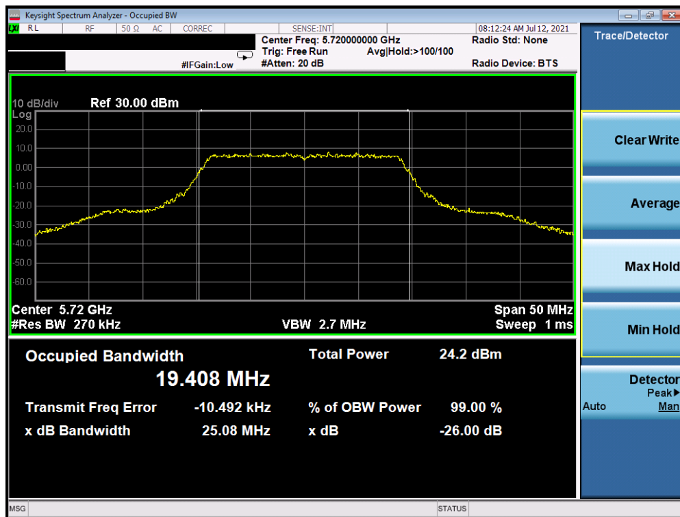
Plot 7-9. 99% OBW and 26dB Bandwidth (20MHz BW 802.11n (UNII Band 2C) – Ch. 144)
