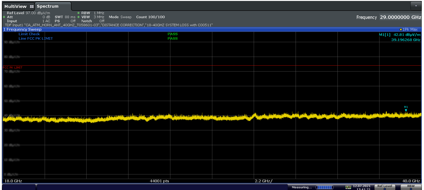
Plot 7-35. Radiated Spurious Emissions 18GHz - 40GHz – H Polarity (802.11n Ch 149)
