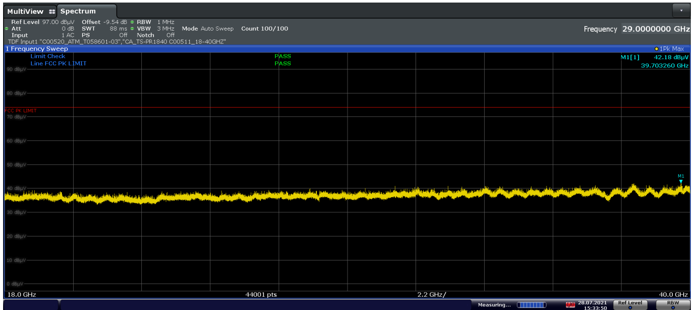
Plot 7-40. Radiated Spurious Emissions – Simultaneous Transmission 18GHz – 40GHz Pol H
