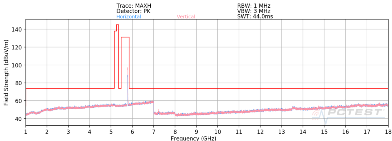
Plot 7-37. Radiated Spurious Emissions above 1GHz (802.11n – UNII 3 Ch. 157)
