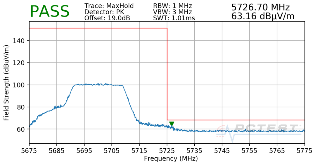
Plot 7-51. Radiated Upper Band Edge Plot (Peak – UNII Band 2C)
