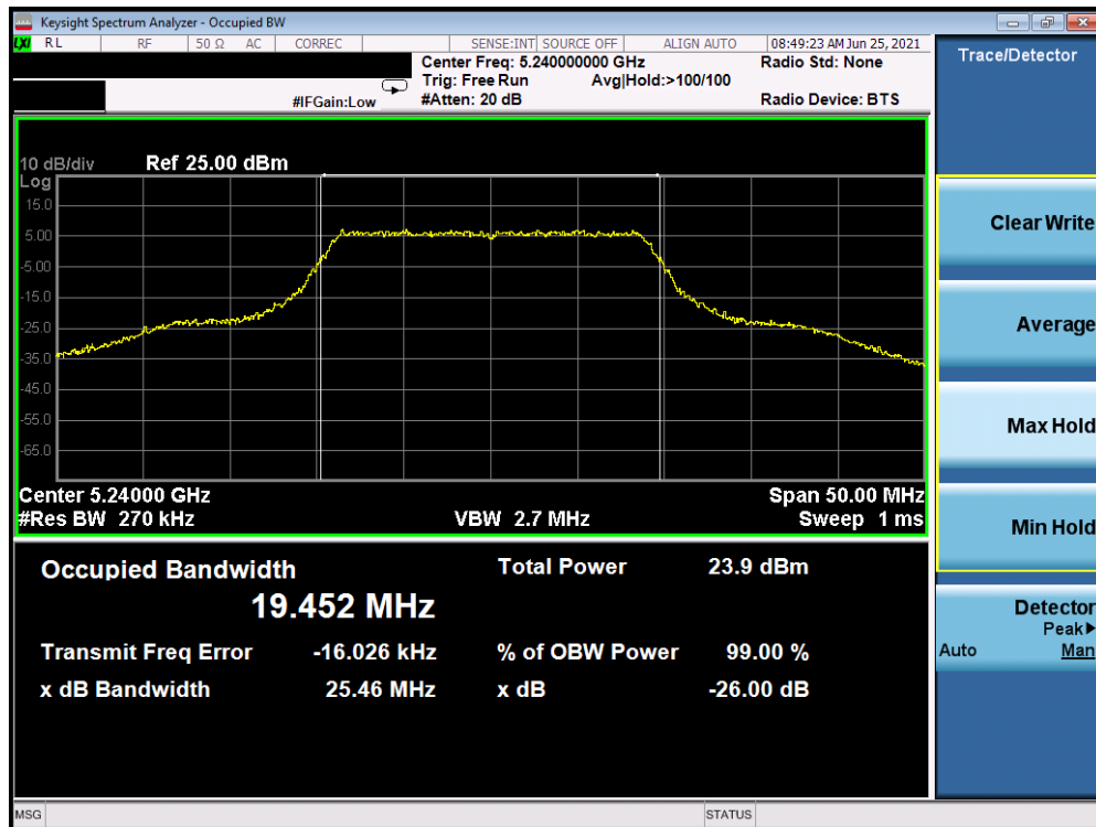
Plot 7-3. 99% OBW and 26dB Bandwidth (20MHz BW 802.11n (UNII Band 1) – Ch. 48)
