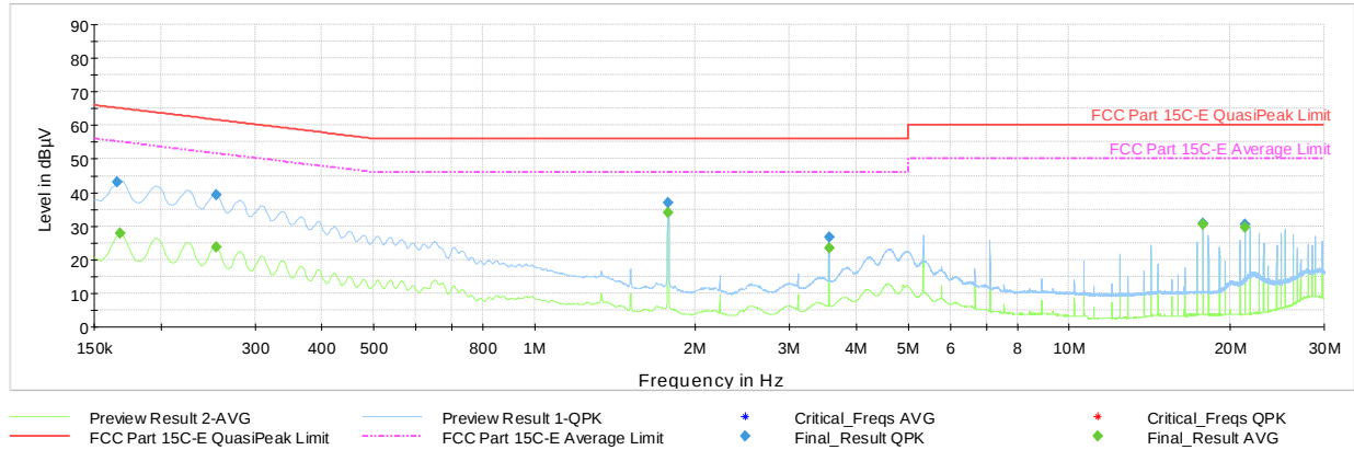
Plot 7-59. AC Line Conducted Plot with 802.11n UNII Band 2C – Ch.149 (N) with AC/DC Adaptor & Magnetic Charger
