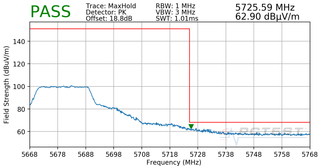
Plot 7-49. Radiated Upper Band Edge Plot (Peak – UNII Band 2C)
