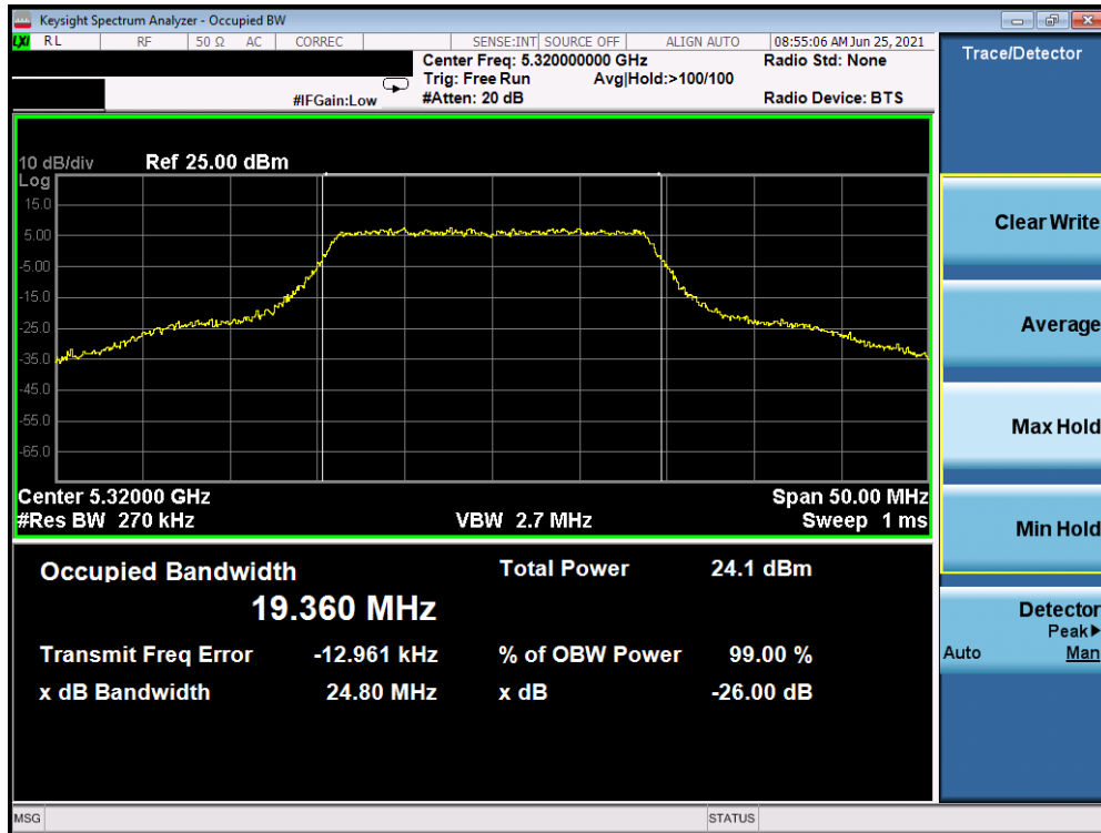
Plot 7-6. 99% OBW and 26dB Bandwidth (20MHz BW 802.11n (UNII Band 2A) – Ch. 64)
