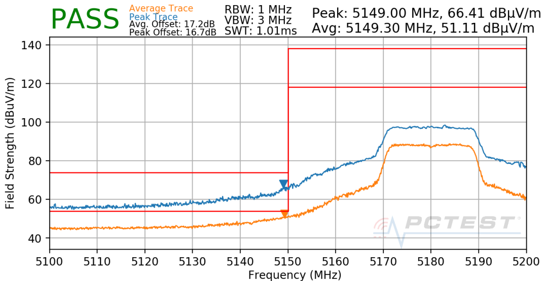
Plot 7-43. Radiated Lower Band Edge Plot (UNII Band 1)
