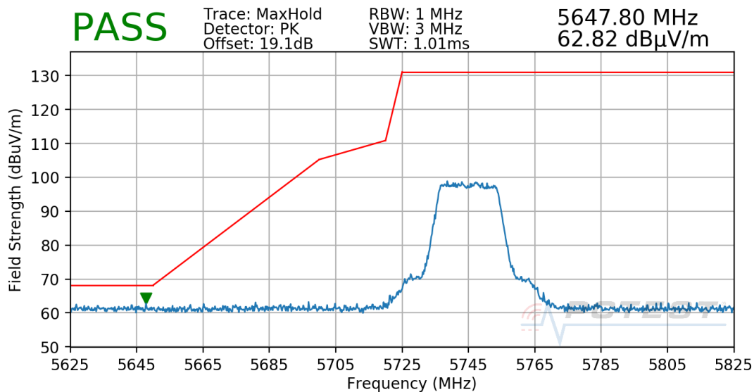
Plot 7-53. Radiated Lower Band Edge Plot (Peak – UNII Band 3)
