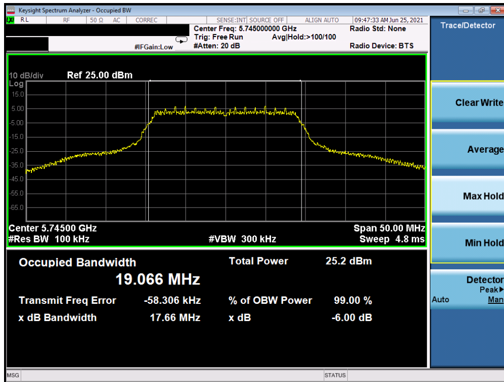
Plot 7-10. 99% OBW and 6dB Bandwidth Plot (20MHz BW 802.11n (UNII Band 3) – Ch. 149)
