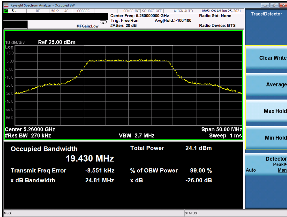
Plot 7-4. 99% OBW and 26dB Bandwidth (20MHz BW 802.11n (UNII Band 2A) – Ch. 52)
