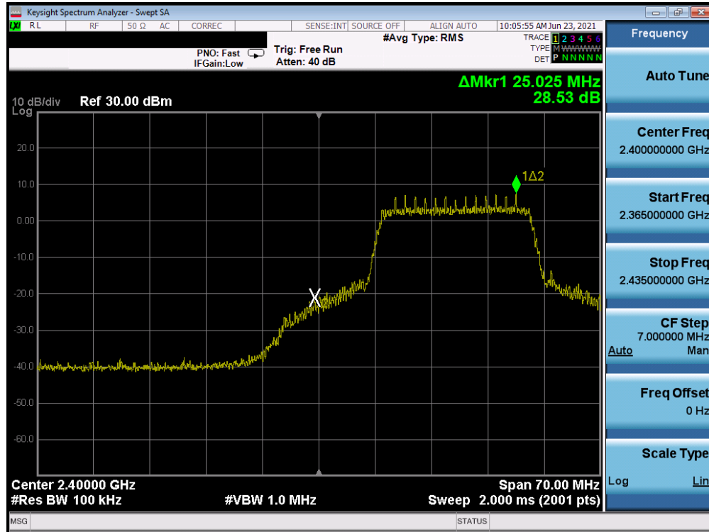
Plot 7-37. Band Edge Plot (802.11n MCS0 – Ch. 2)
