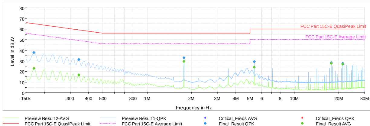
Plot 7-74.AC Line Conducted Plot 802.11b – Ch.6 (L1), with AC/DC Adapter and Magnetic Charger
