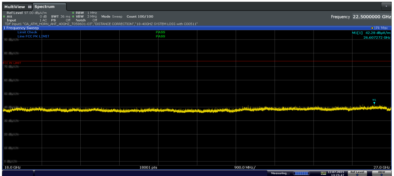
Plot 7-57. Radiated Spurious Plot above 18GHz (802.11b – Ch. 6 Pol V)
