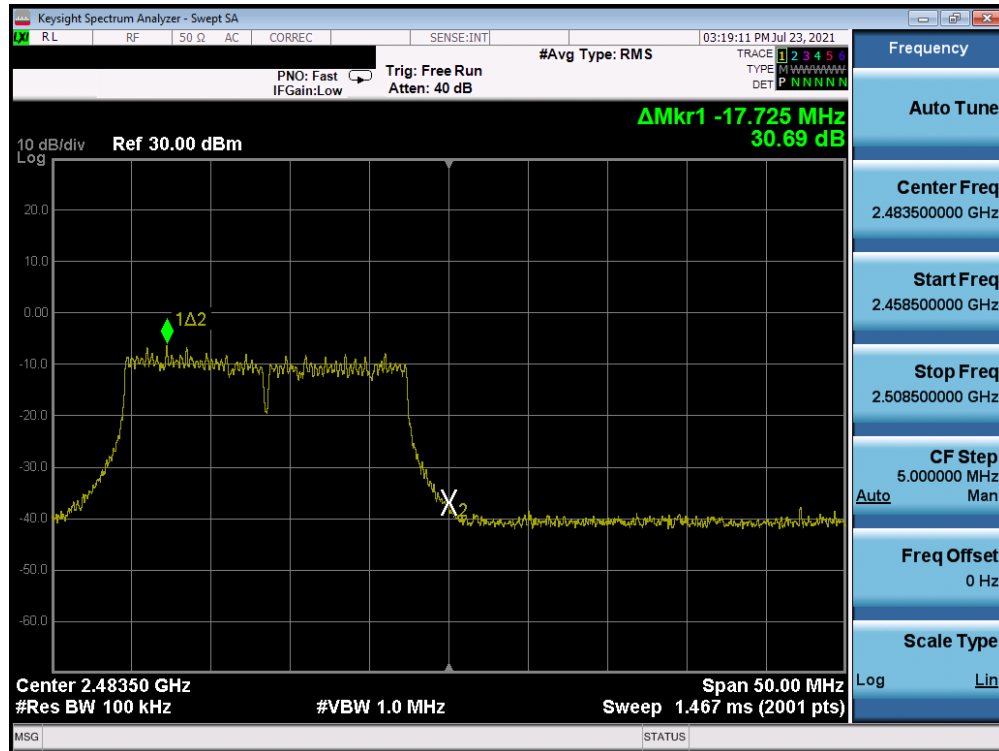
Plot 7-46. Band Edge Plot (802.11n MCS7 – Ch. 13)
