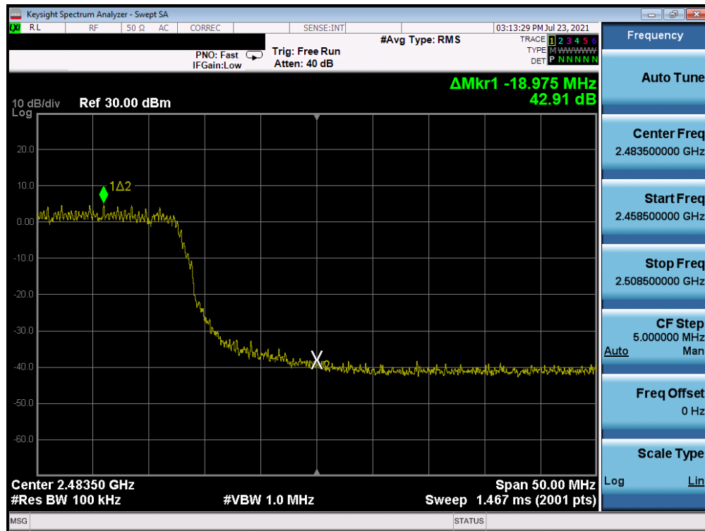
Plot 7-44. Band Edge Plot (802.11n MCS7 – Ch. 11)
