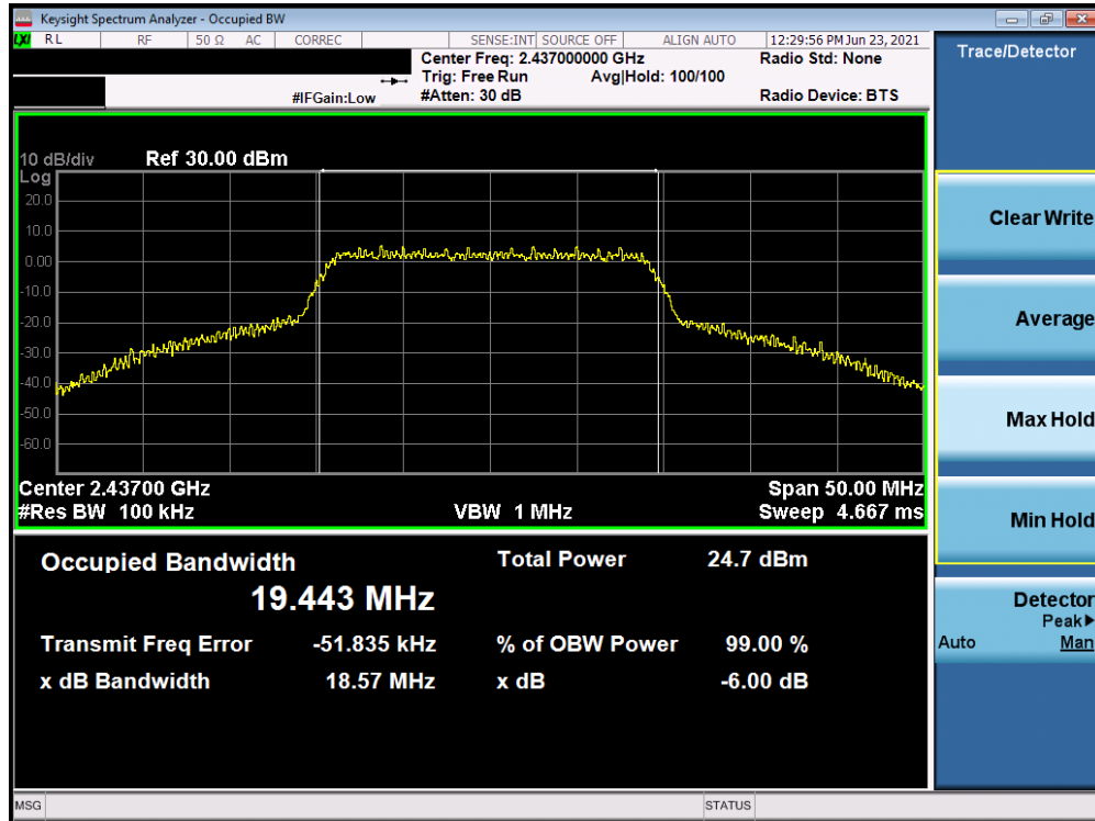
Plot 7-11. 6dB BW and 99% OBW Plot (802.11n MCS7 – Ch. 6)
