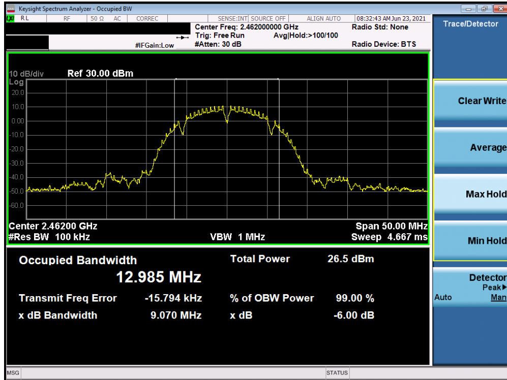
Plot 7-3. 6dB BW and 99% OBW Plot (802.11b – Ch. 11)
