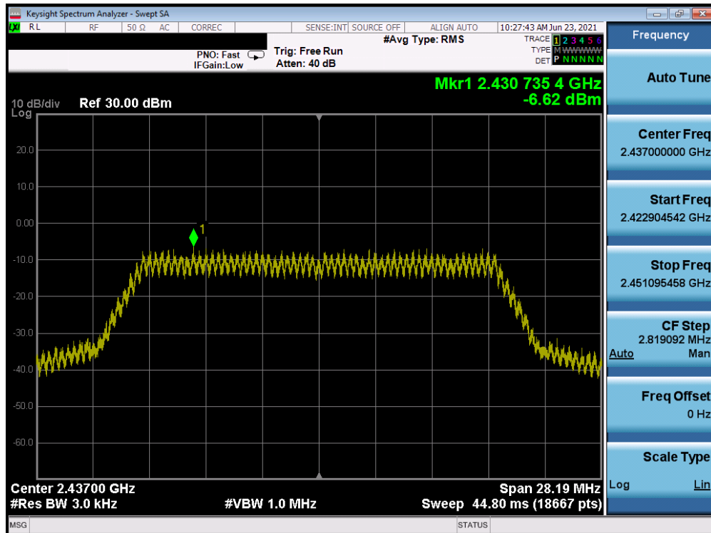
Plot 7-20. Power Spectral Density Plot (802.11n MCS0 – Ch. 6)
