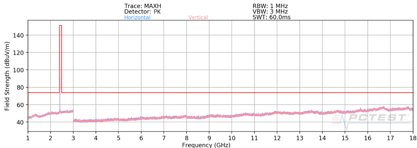
Plot 7-53. Radiated Spurious Emissions above 1GHz (802.11b – Ch. 1)
