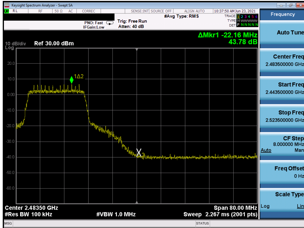
Plot 7-39. Band Edge Plot (802.11n MCS0 – Ch. 10)
