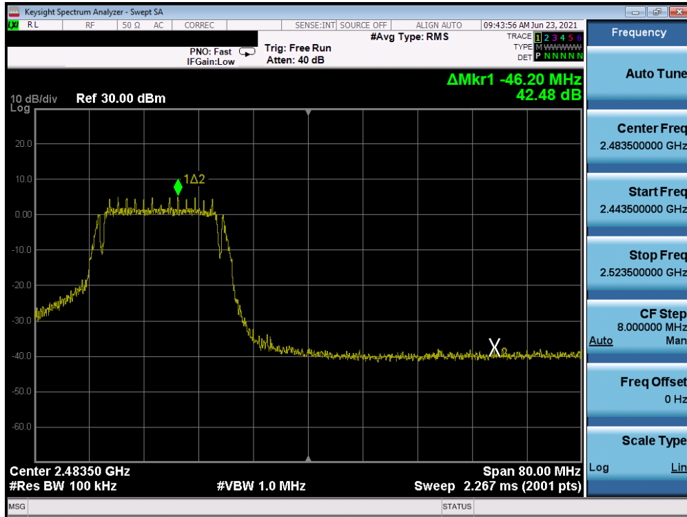
Plot 7-33. Band Edge Plot (802.11g – Ch. 11)
