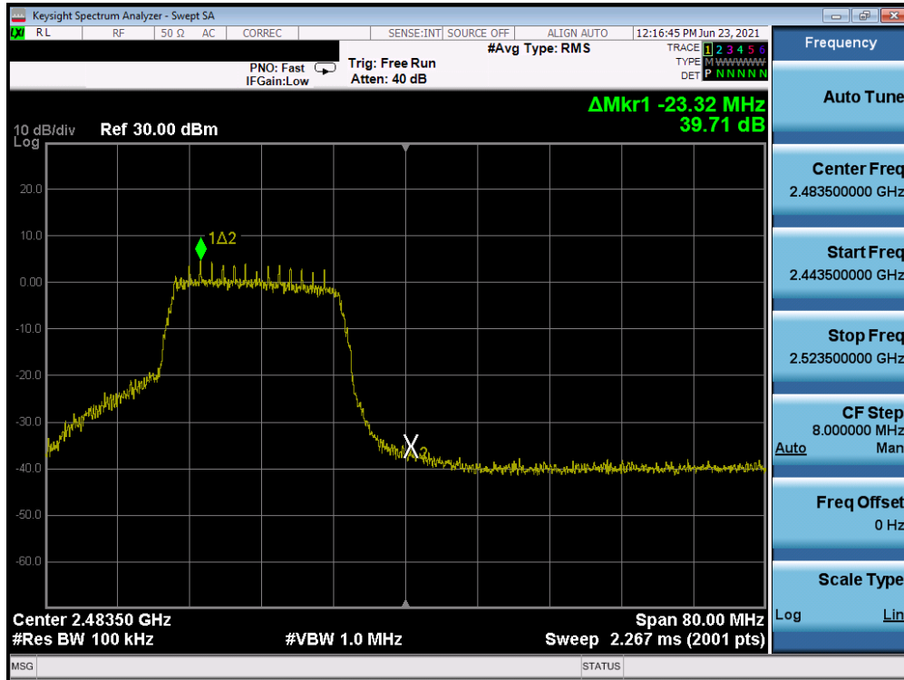
Plot 7-41. Band Edge Plot (802.11n MCS0 – Ch. 12)
