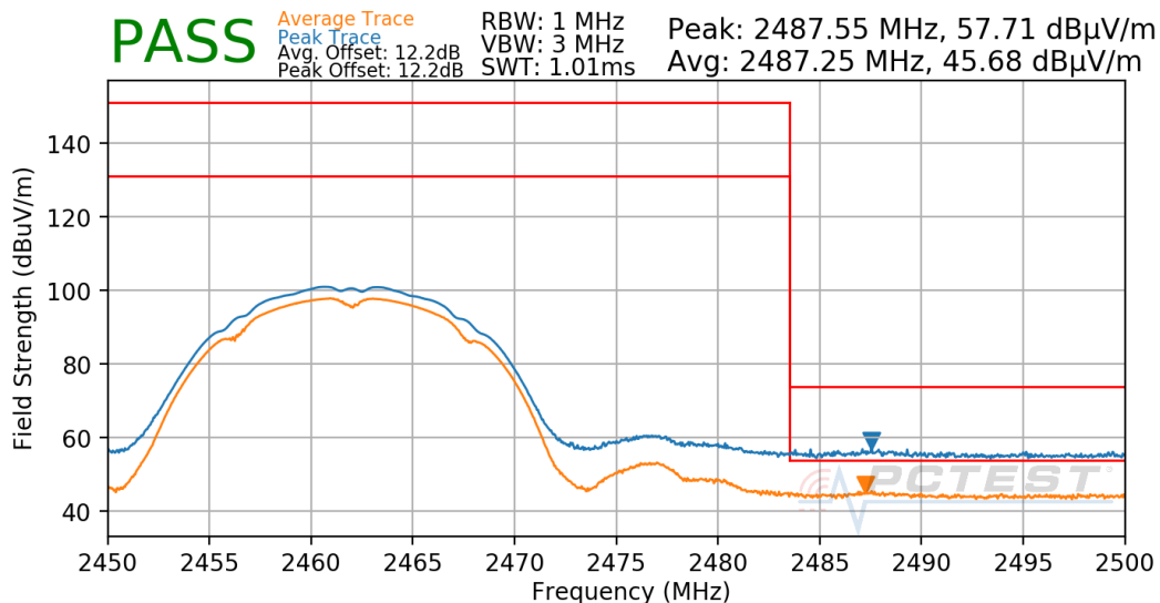
Plot 7-59. Radiated Restricted Upper Band Edge Measurement
