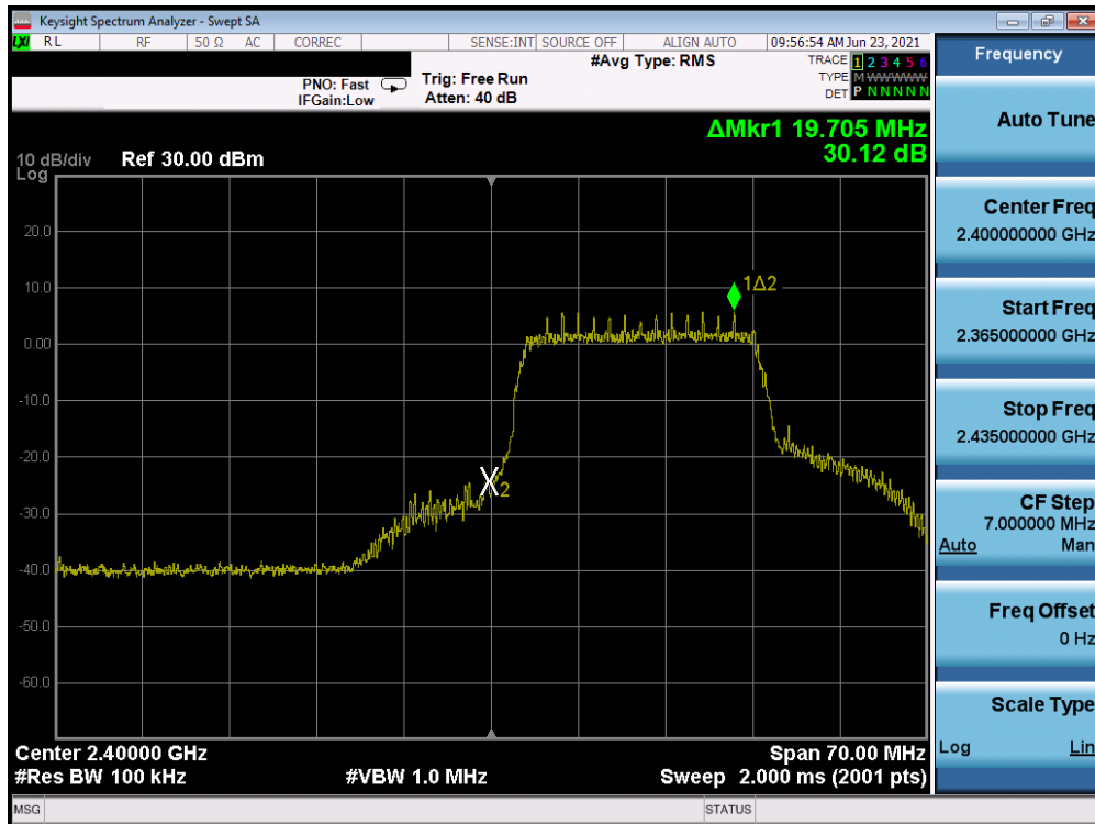
Plot 7-36. Band Edge Plot (802.11n MCS0 – Ch. 1)
