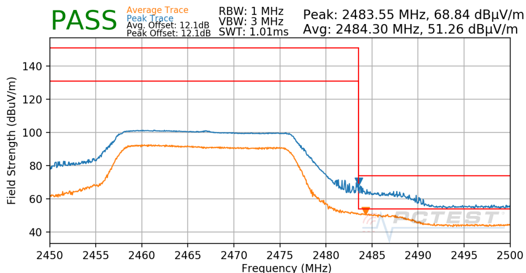
Plot 7-67. Radiated Restricted Upper Band Edge Measurement
