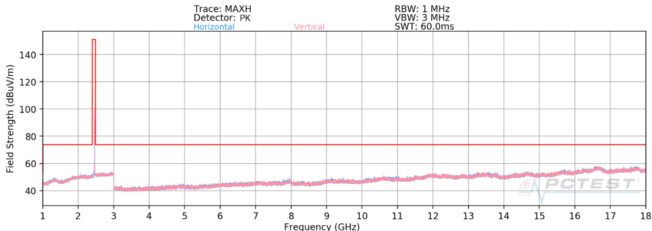
Plot 7-55. Radiated Spurious Emissions above 1GHz (802.11b – Ch. 11)
