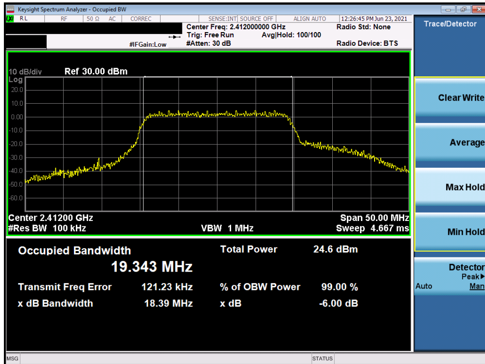
Plot 7-10. 6dB BW and 99% OBW Plot (802.11n MCS7 – Ch. 1)
