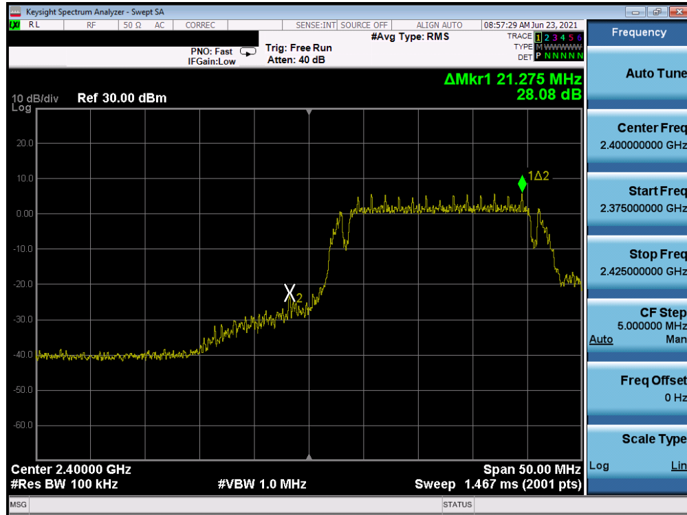
Plot 7-29. Band Edge Plot (802.11g – Ch. 1)
