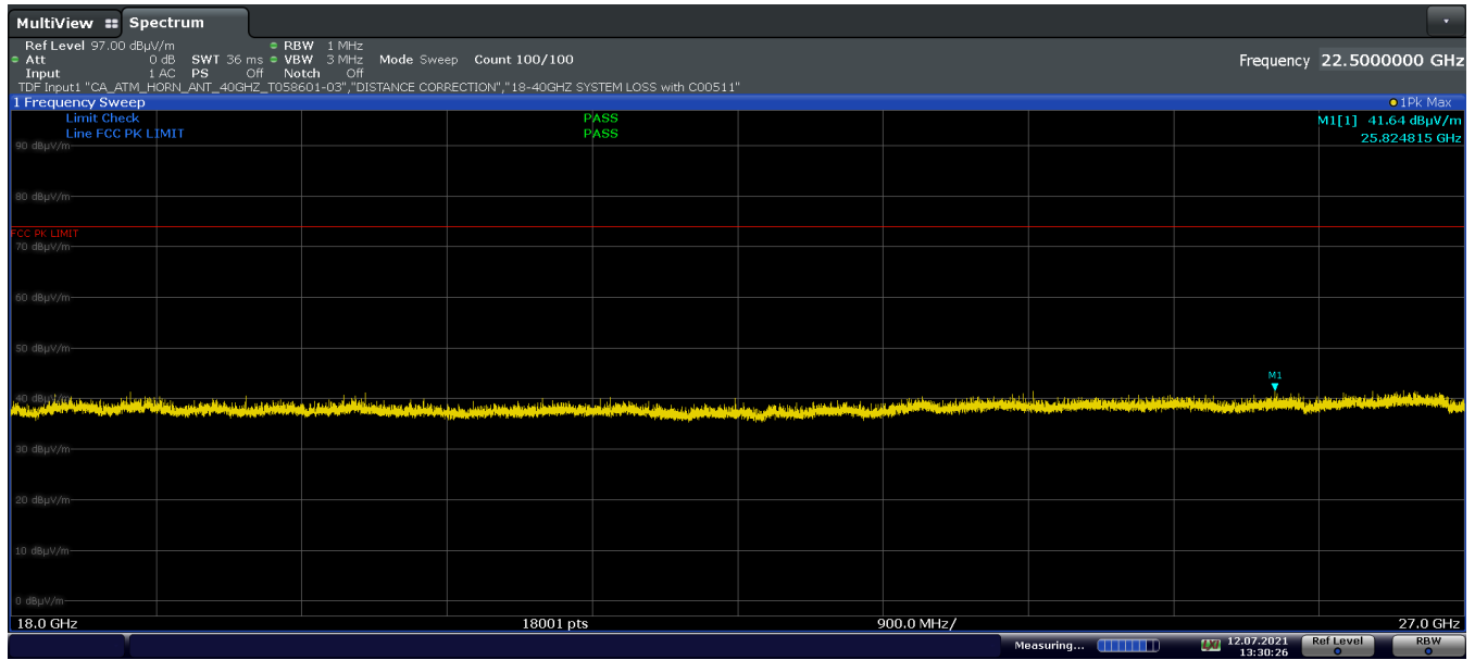
Plot 7-56. Radiated Spurious Plot above 18GHz (802.11b – Ch. 6 Pol H)
