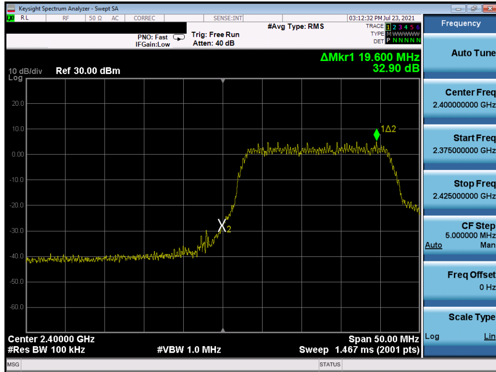
Plot 7-43. Band Edge Plot (802.11n MCS7 – Ch. 1)
