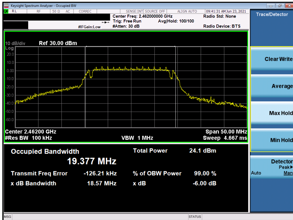
Plot 7-6. 6dB BW and 99% OBW Plot (802.11g – Ch. 11)
