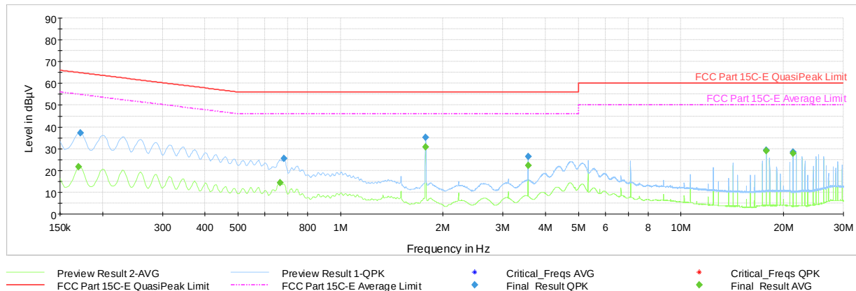
Plot 7-75.AC Line Conducted Plot 802.11b – Ch.6 (N), with AC/DC Adapter and Magnetic Charger
