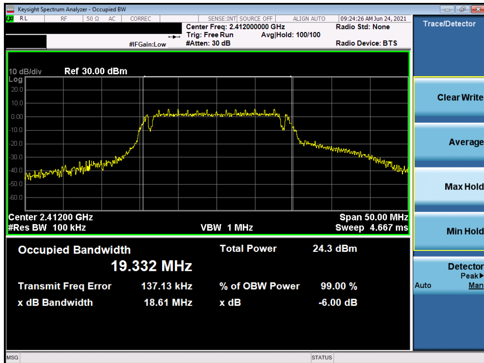
Plot 7-4. 6dB BW and 99% OBW Plot (802.11g – Ch. 1)
