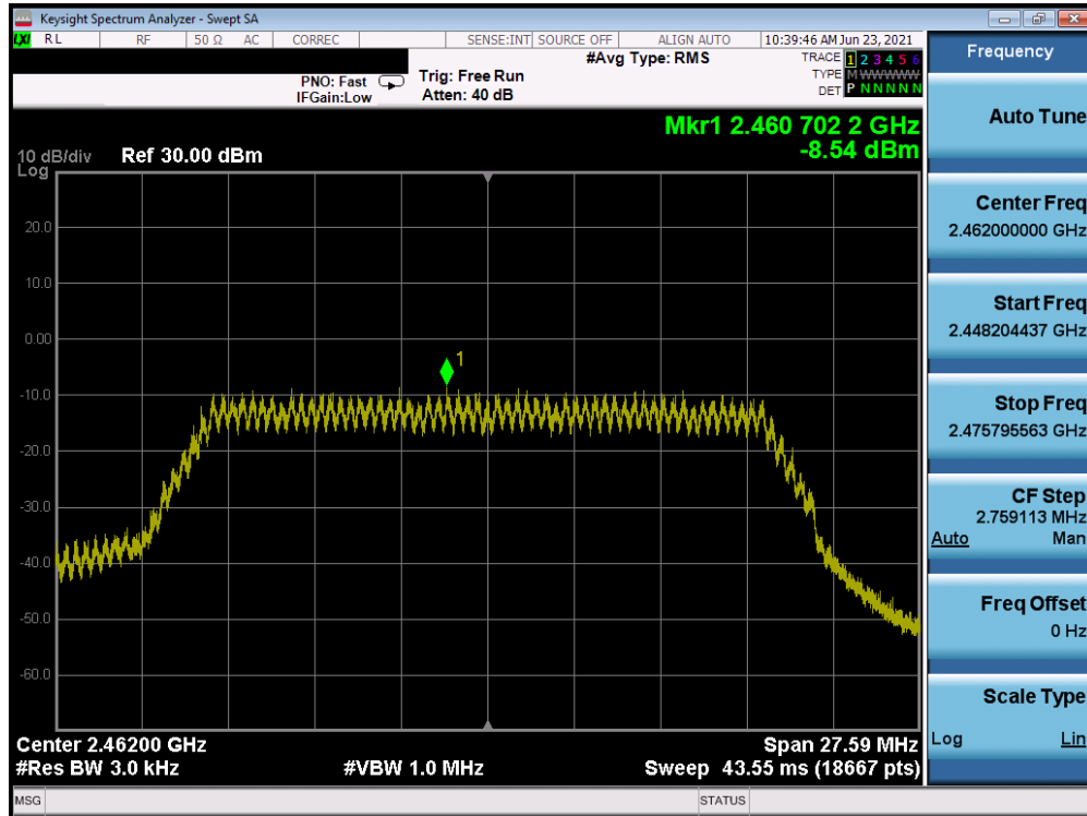
Plot 7-21. Power Spectral Density Plot (802.11n MCS0– Ch. 11)
