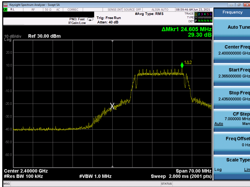
Plot 7-30. Band Edge Plot (802.11g – Ch. 2)
