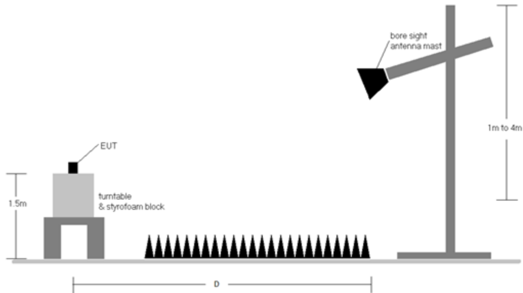
Figure 7-6. Radiated Measurement Setup
