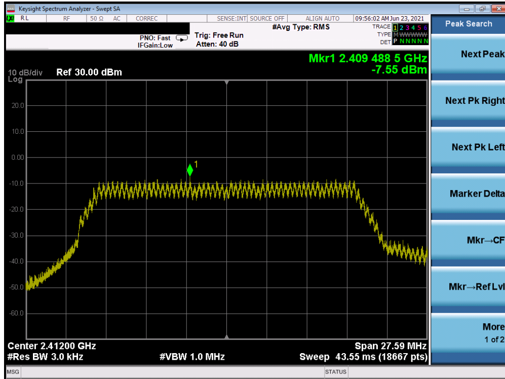
Plot 7-19. Power Spectral Density Plot (802.11n MCS0 – Ch. 1)
