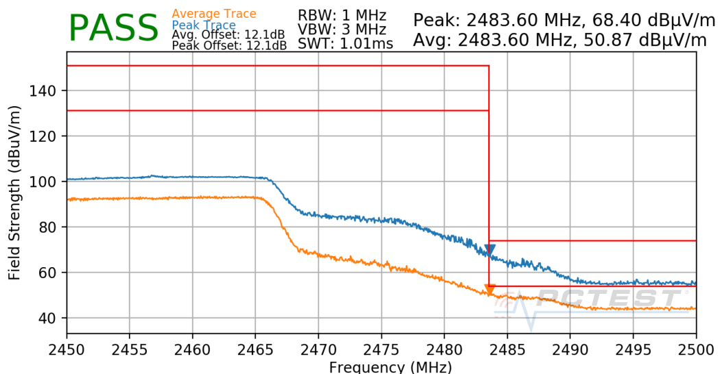
Plot 7-65. Radiated Restricted Upper Band Edge Measurement
