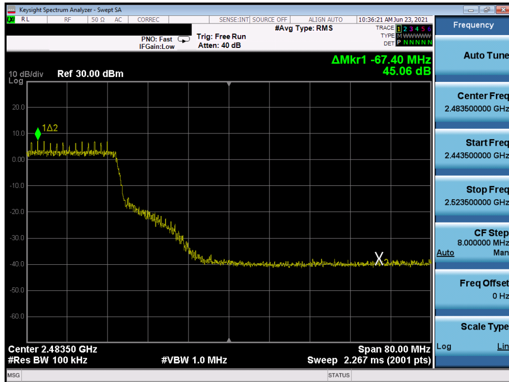
Plot 7-38. Band Edge Plot (802.11n MCS0 – Ch. 9)
