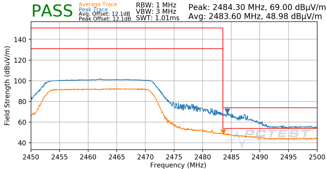
Plot 7-66. Radiated Restricted Upper Band Edge Measurement
