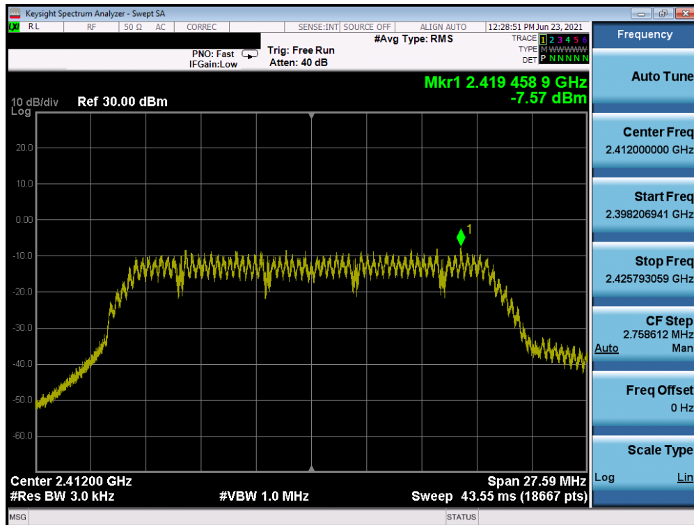
Plot 7-22. Power Spectral Density Plot (802.11n MCS7 – Ch. 1)
