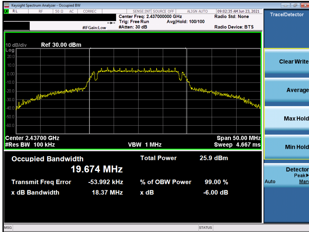
Plot 7-5. 6dB BW and 99% OBW Plot (802.11g – Ch. 6)
