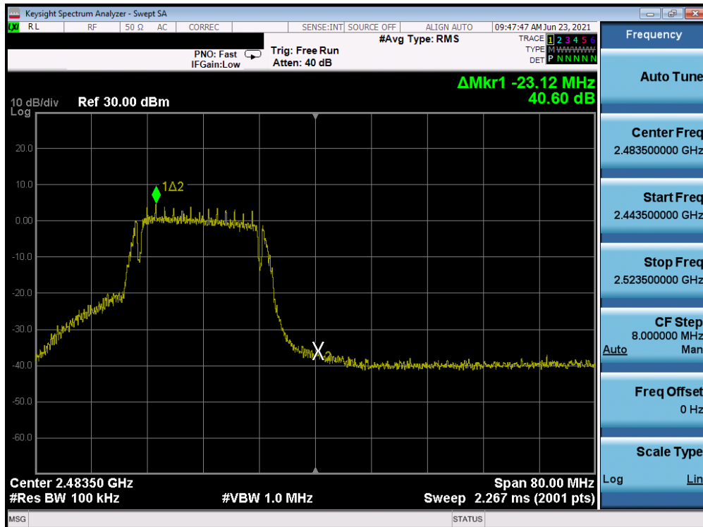
Plot 7-34. Band Edge Plot (802.11g – Ch. 12)
