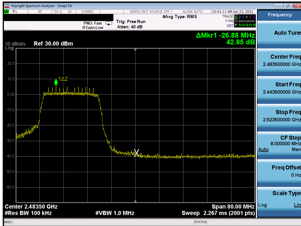
Plot 7-40. Band Edge Plot (802.11n MCS0 – Ch. 11)
