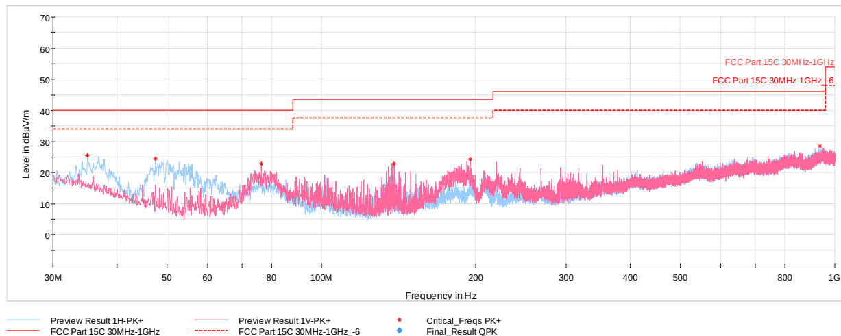
Plot 7-73. Radiated Spurious Emissions 30MHz-1GHz 802.11b – Ch.6, with AC/DC Adapter and Magnetic Charger
