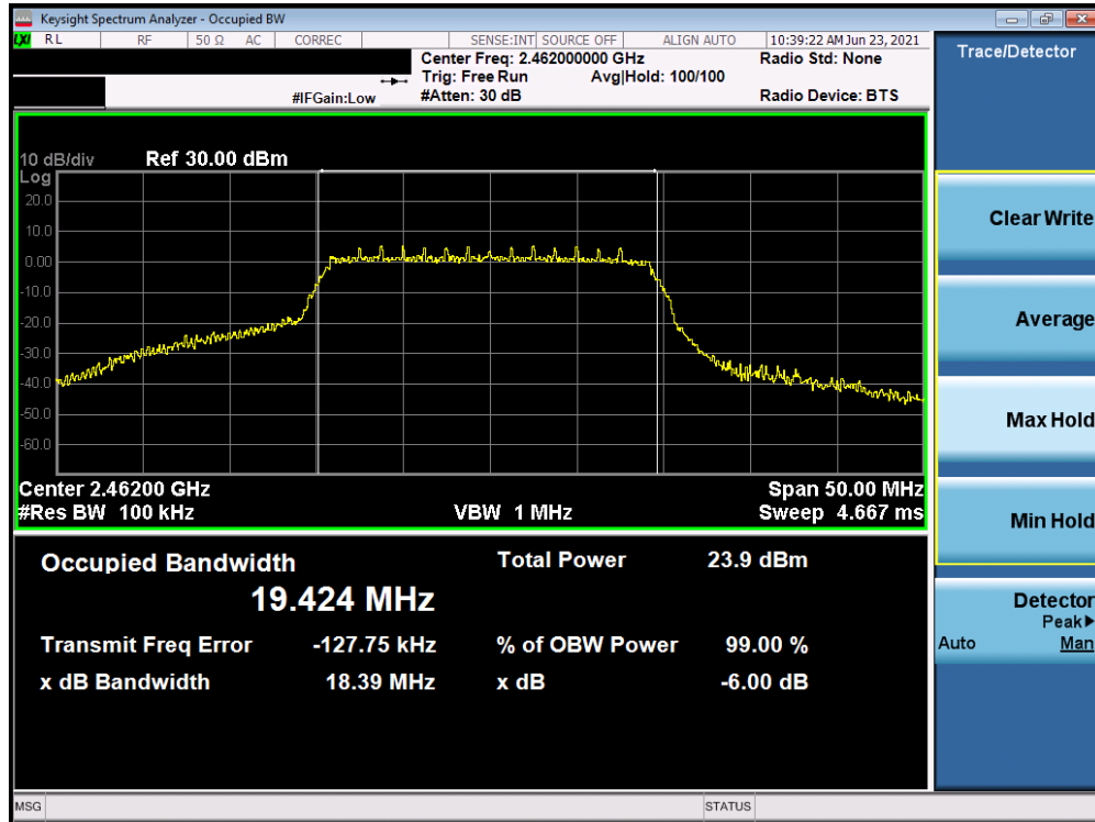
Plot 7-9. 6dB BW and 99% OBW Plot (802.11n MCS0 – Ch. 11)
