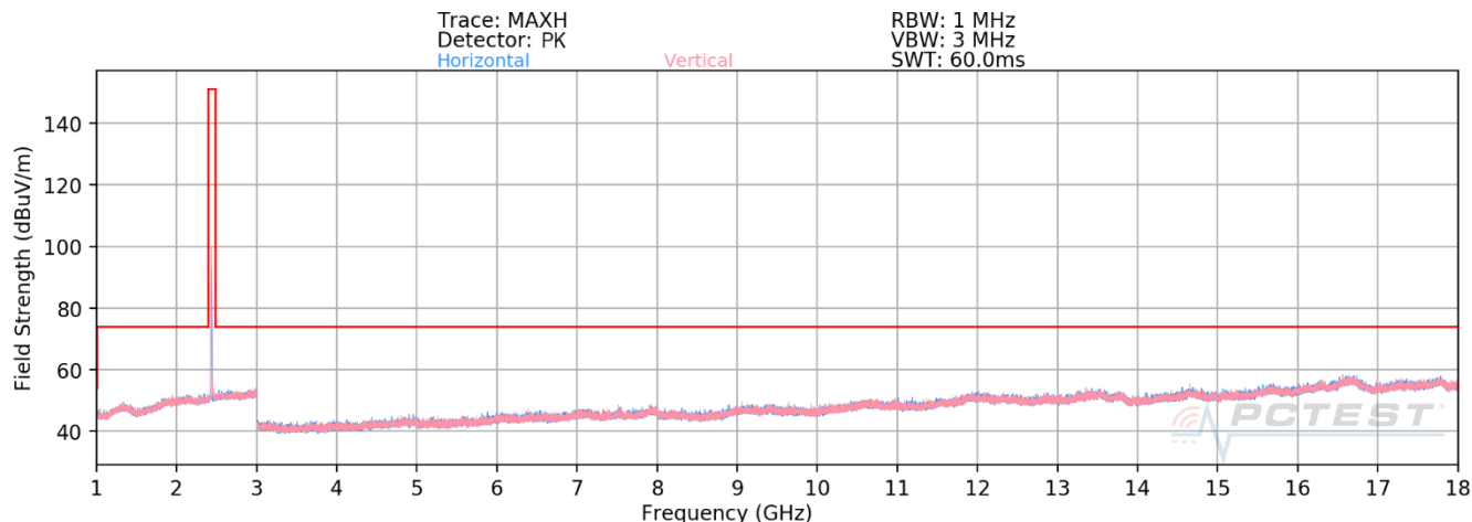
Plot 7-54. Radiated Spurious Emissions above 1GHz (802.11b – Ch. 6)
