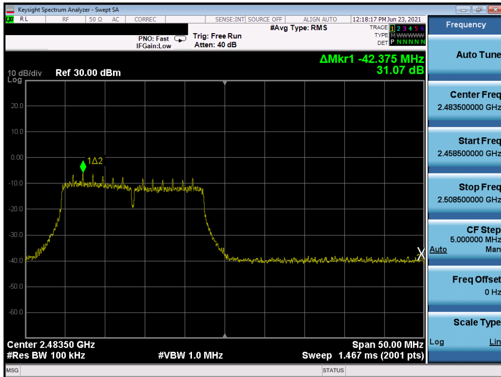
Plot 7-42. Band Edge Plot (802.11n MCS0 – Ch. 13)
