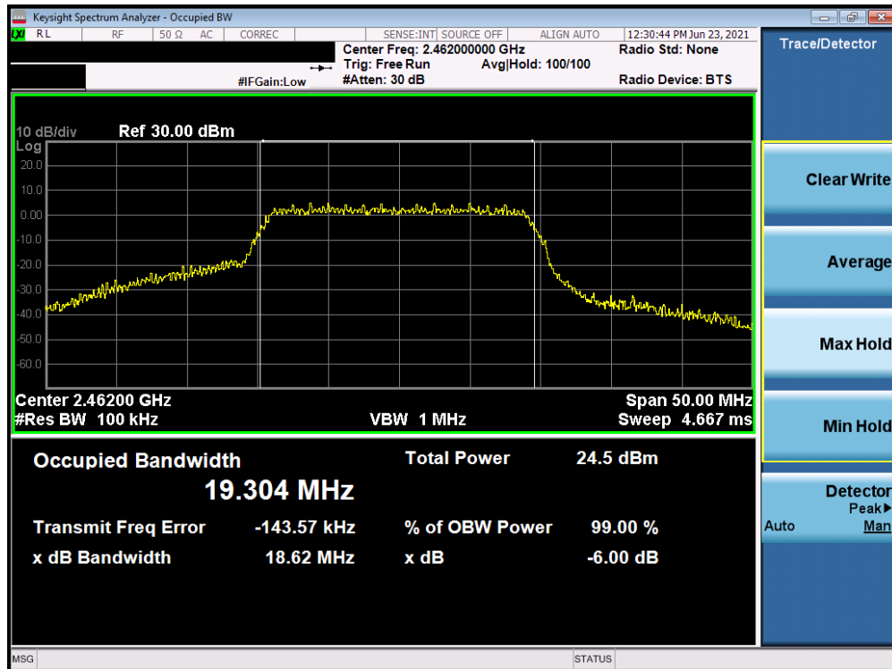
Plot 7-12. 6dB BW and 99% OBW Plot (802.11n MCS7 – Ch. 11)
