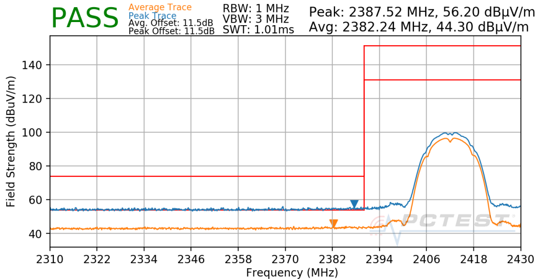
Plot 7-58. Radiated Restricted Lower Band Edge Measurement
