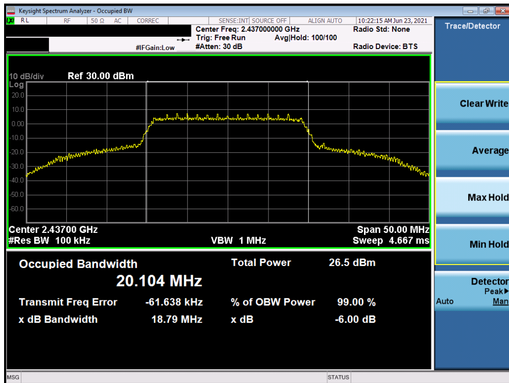
Plot 7-8. 6dB BW and 99% OBW Plot (802.11n MCS0 – Ch. 6)
