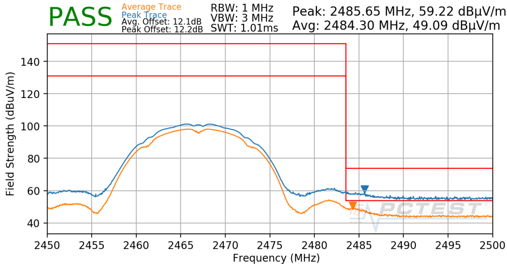
Plot 7-60. Radiated Restricted Upper Band Edge Measurement
