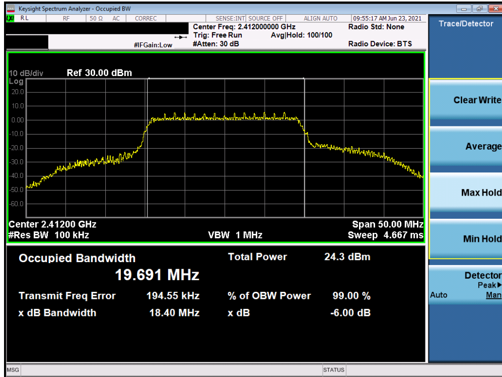
Plot 7-7. 6dB BW and 99% OBW Plot (802.11n MCS0 – Ch. 1)
