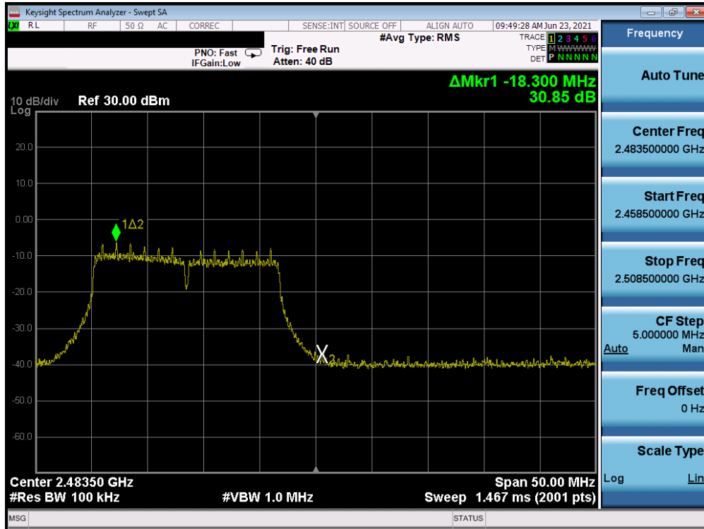
Plot 7-35. Band Edge Plot (802.11g – Ch. 13)
