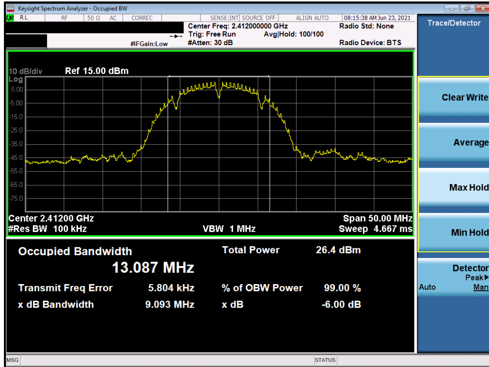
Plot 7-1. 6dB BW and 99% OBW Plot (802.11b – Ch. 1)
