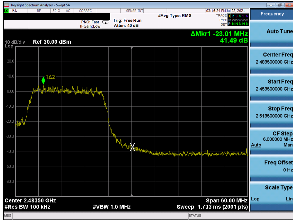
Plot 7-45. Band Edge Plot (802.11n MCS7 – Ch. 12)
