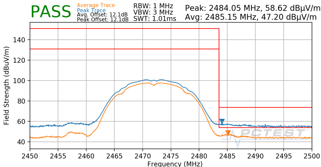
Plot 7-61. Radiated Restricted Upper Band Edge Measurement
