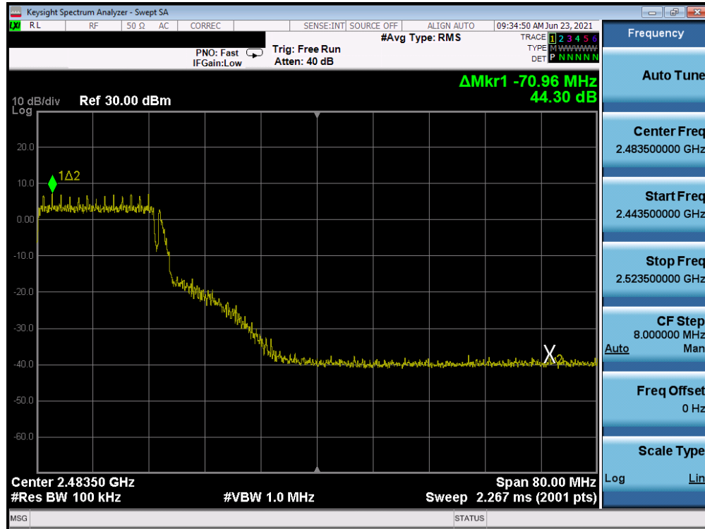
Plot 7-31. Band Edge Plot (802.11g – Ch. 9)
