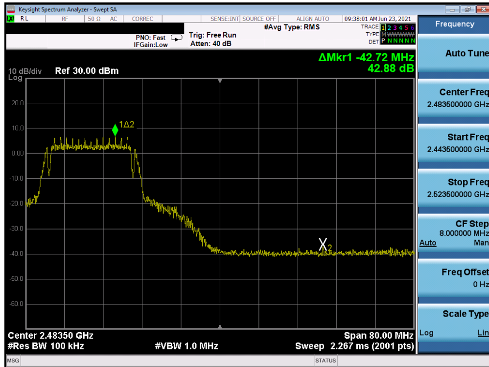
Plot 7-32. Band Edge Plot (802.11g – Ch. 10)
