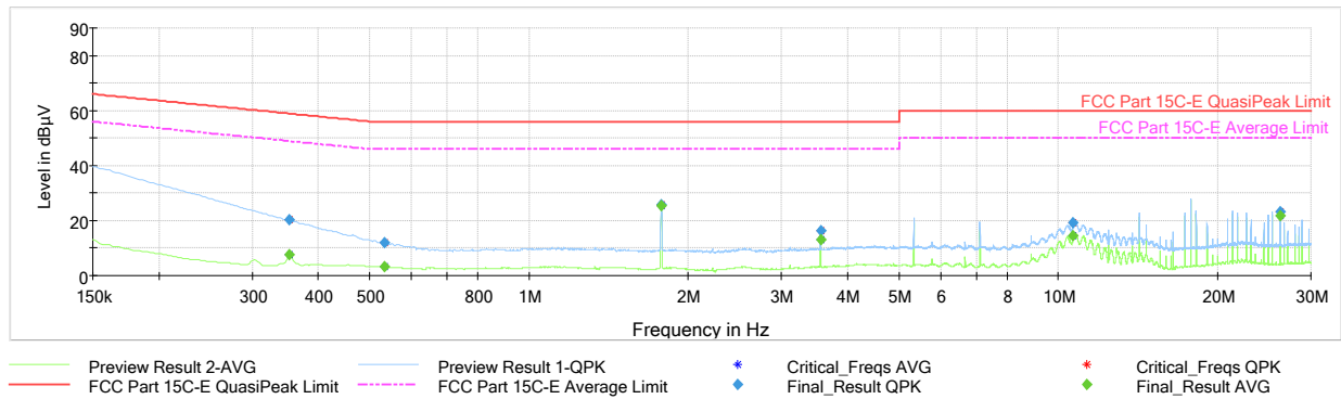
Plot 7-40. AC Line Conducted Plot with Bluetooth LE (1Mbps, ePA – Ch.19, N, with AC/DC Adapter + Magnetic Charger)
