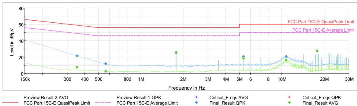
Plot 7-39. AC Line Conducted Plot with Bluetooth LE (1Mbps, ePA – Ch.19, L1, with AC/DC Adapter + Magnetic Charger)
