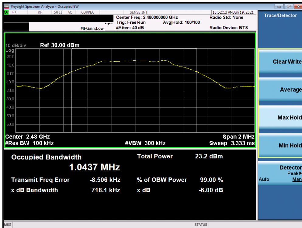
Plot 7-3. 6dB Bandwidth & 99% OBW Plot (Bluetooth (LE), 2Mbps, ePA – Ch.39)
