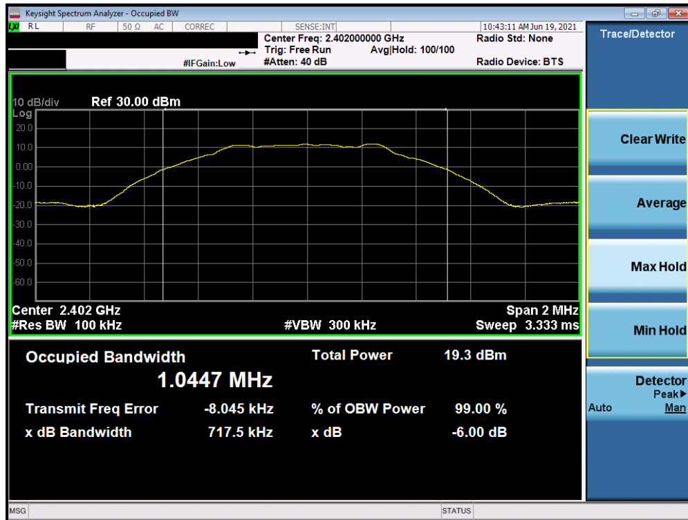
Plot 7-1. 6dB Bandwidth & 99% OBW Plot (Bluetooth (LE), 1Mbps, ePA – Ch. 0)
