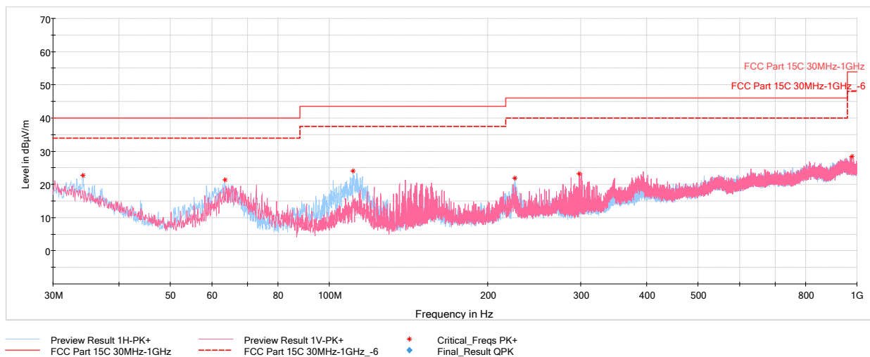
Plot 7-38. Radiated Spurious Plot Below 1GHz 1Mbps, ePA – Ch.19, Pol. H & V, with AC/DC Adapter + Magnetic Charger)
