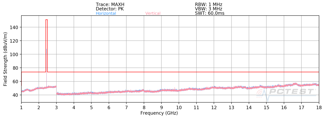
Plot 7-30. Radiated Spurious Plot Above 1GHz (1Mbps, ePA – Ch. 19, Ant. Pol. H & V)
