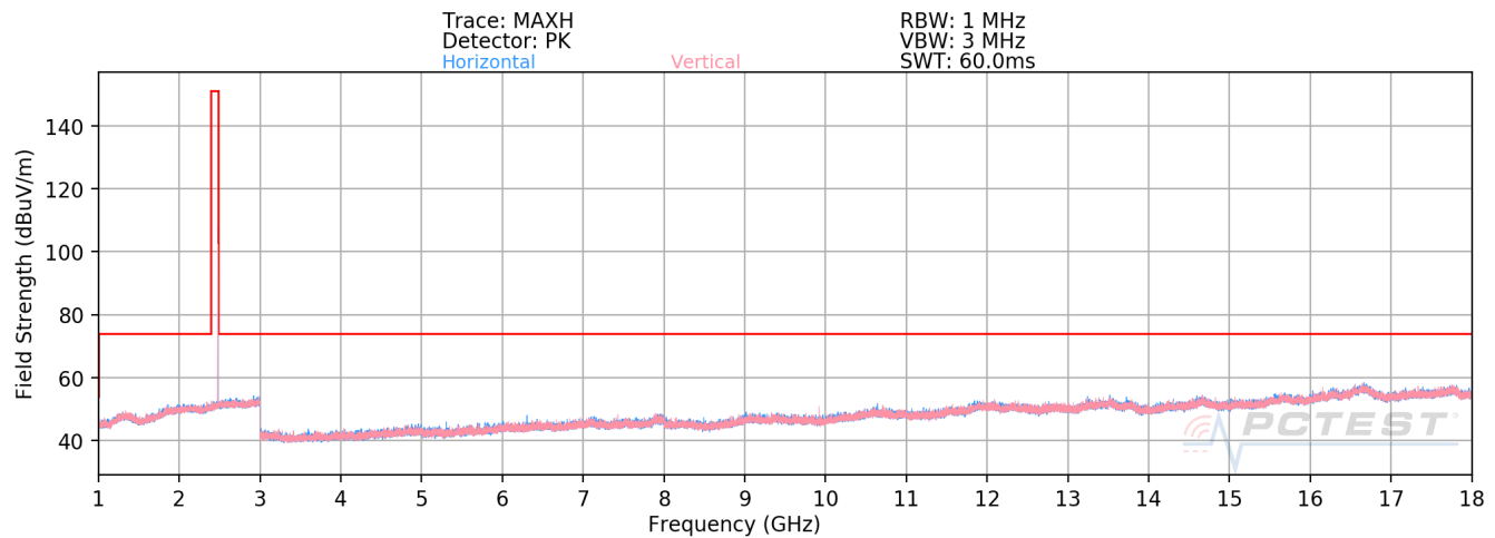
Plot 7-31. Radiated Spurious Plot Above 1GHz (1Mbps ePA – Ch. 39, Ant. Pol. H & V)
