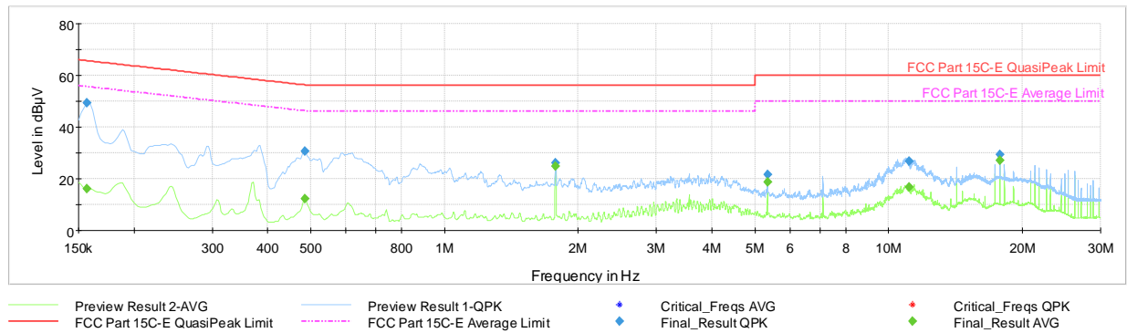
Plot 7-39. AC Line Conducted Plot with Bluetooth HDR (4Mbps, ePA – Ch.38, L1, with AC/DC Adapter + Magnetic Charger)
