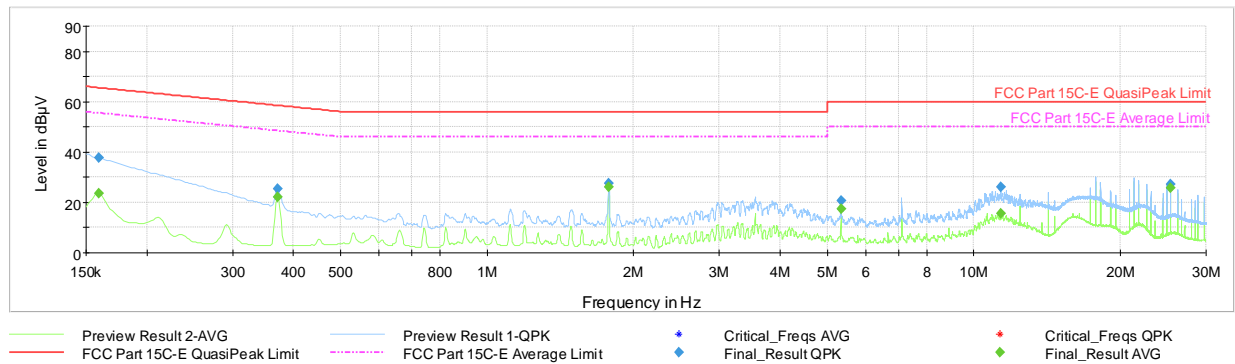
Plot 7-40. AC Line Conducted Plot with Bluetooth HDR (4Mbps, ePA – Ch.38, N, with AC/DC Adapter + Magnetic Charger)
