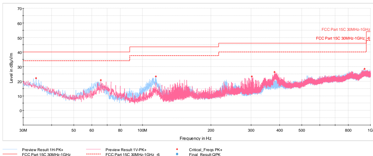
Plot 7-38. Radiated Spurious Plot Below 1GHz (4Mbps, ePA – Ch. 38, Pol. H & V, with (AC/DC Adapter + Magnetic Charger)
