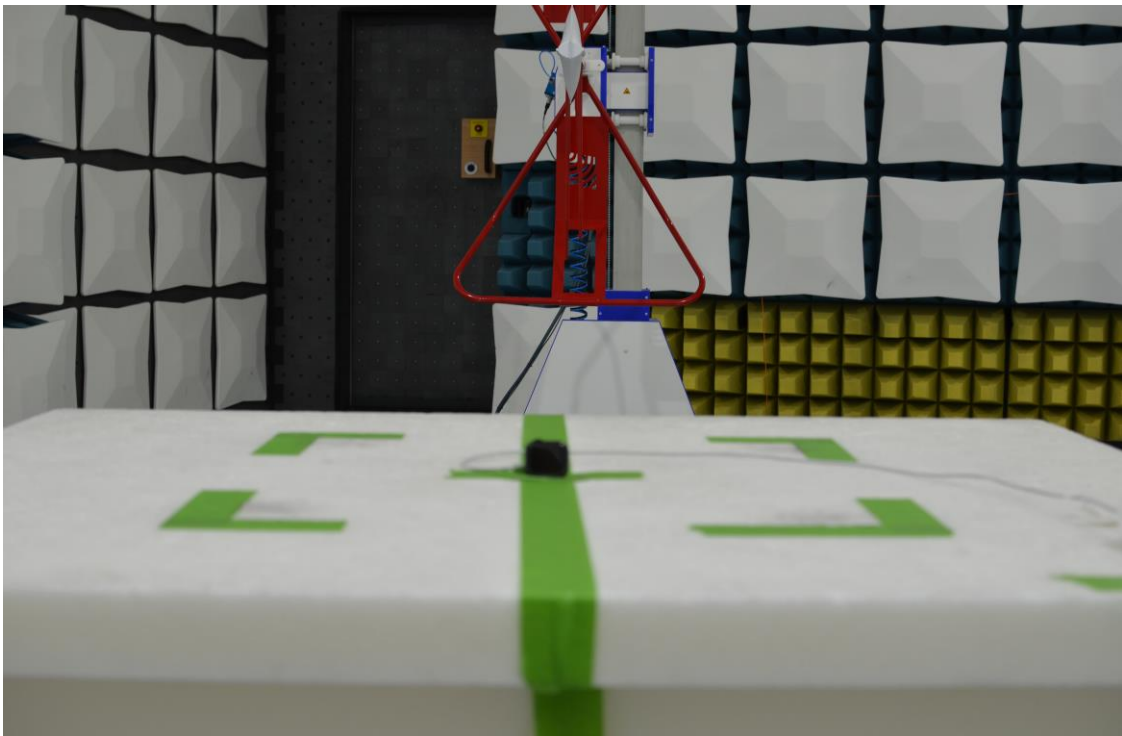
Figure 10: 30MHz-1GHz Test Setup (Rear View)
