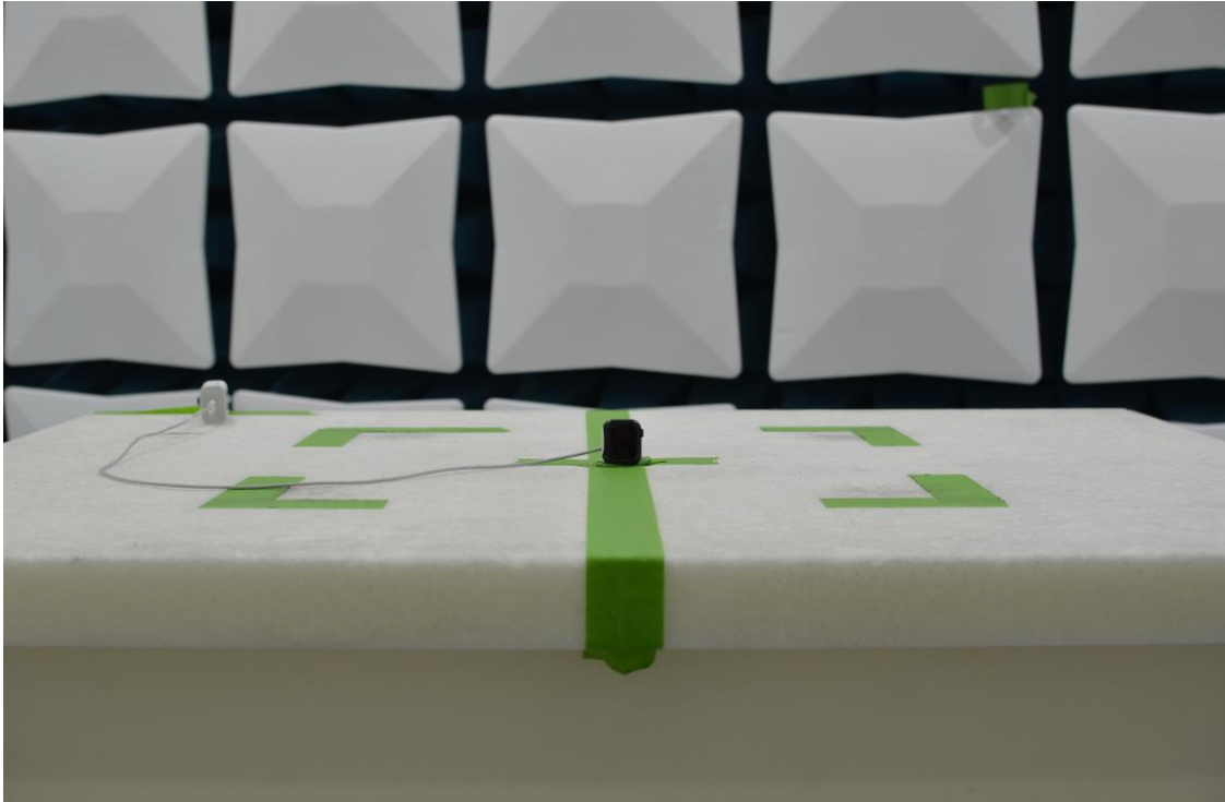
Figure 11: 30MHz-1GHz Test Setup (Front View)
