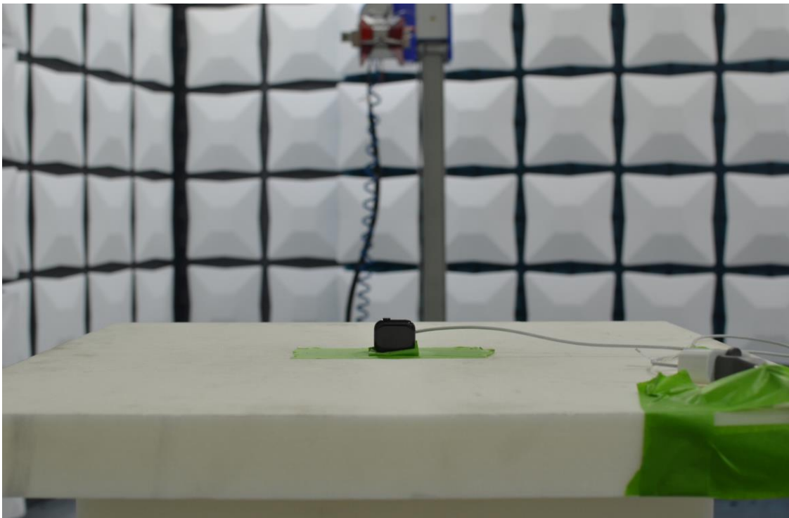
Figure 4: 1-18GHz Test Setup (Rear View)
