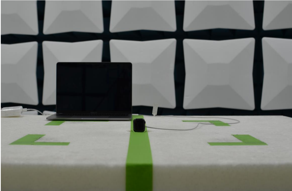
Figure 17: 30MHz-1GHz Test Setup (Front View)
