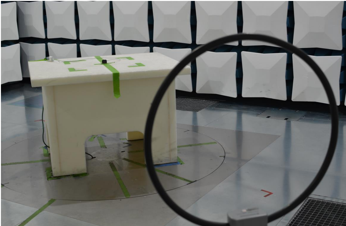
Figure 20: 9kHz-30MHz Test Setup (Front View)
