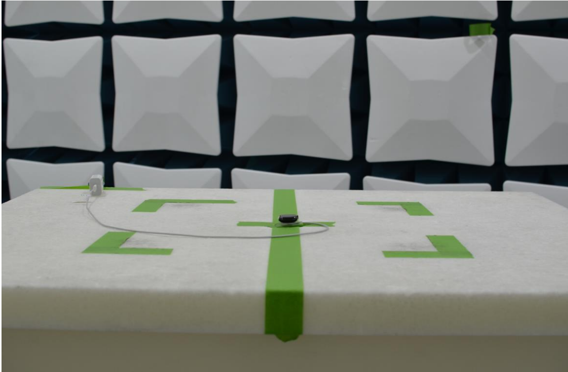
Figure 7: 30MHz-1GHz Test Setup (Front View)
