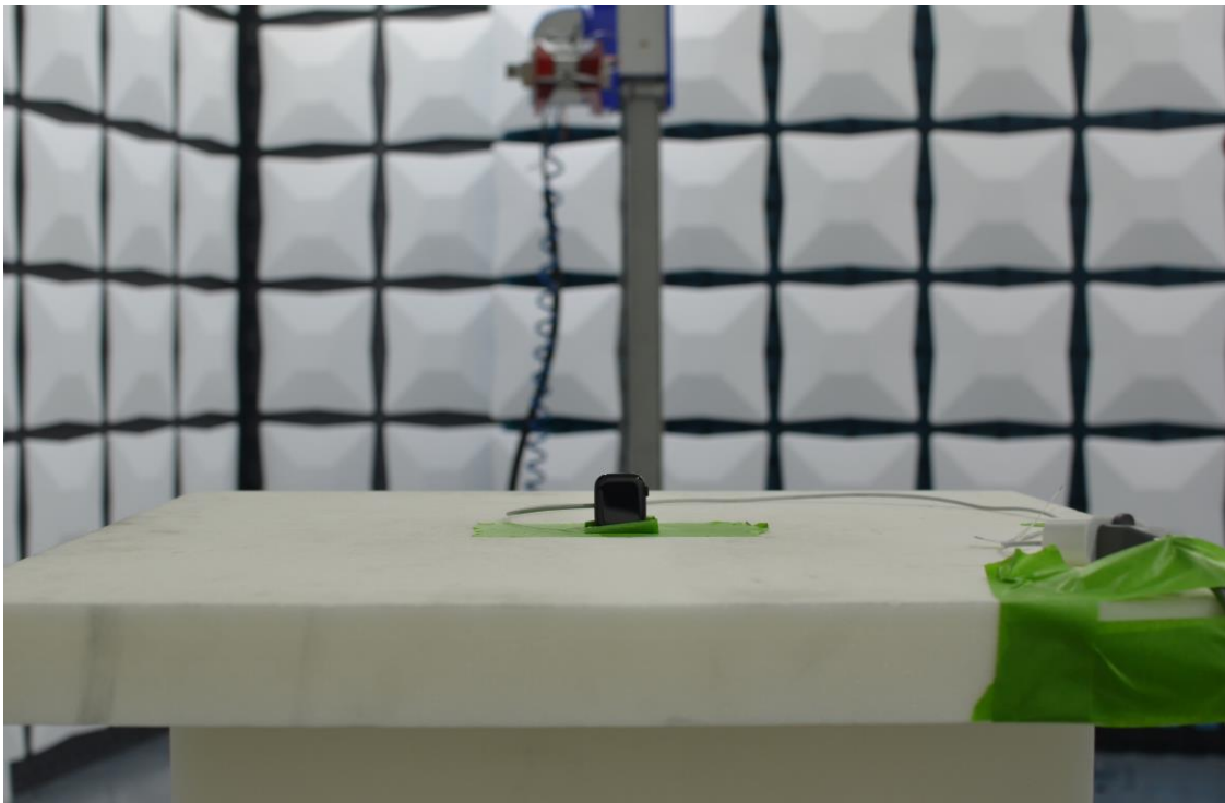
Figure 6: 1-18GHz Test Setup (Rear View)
