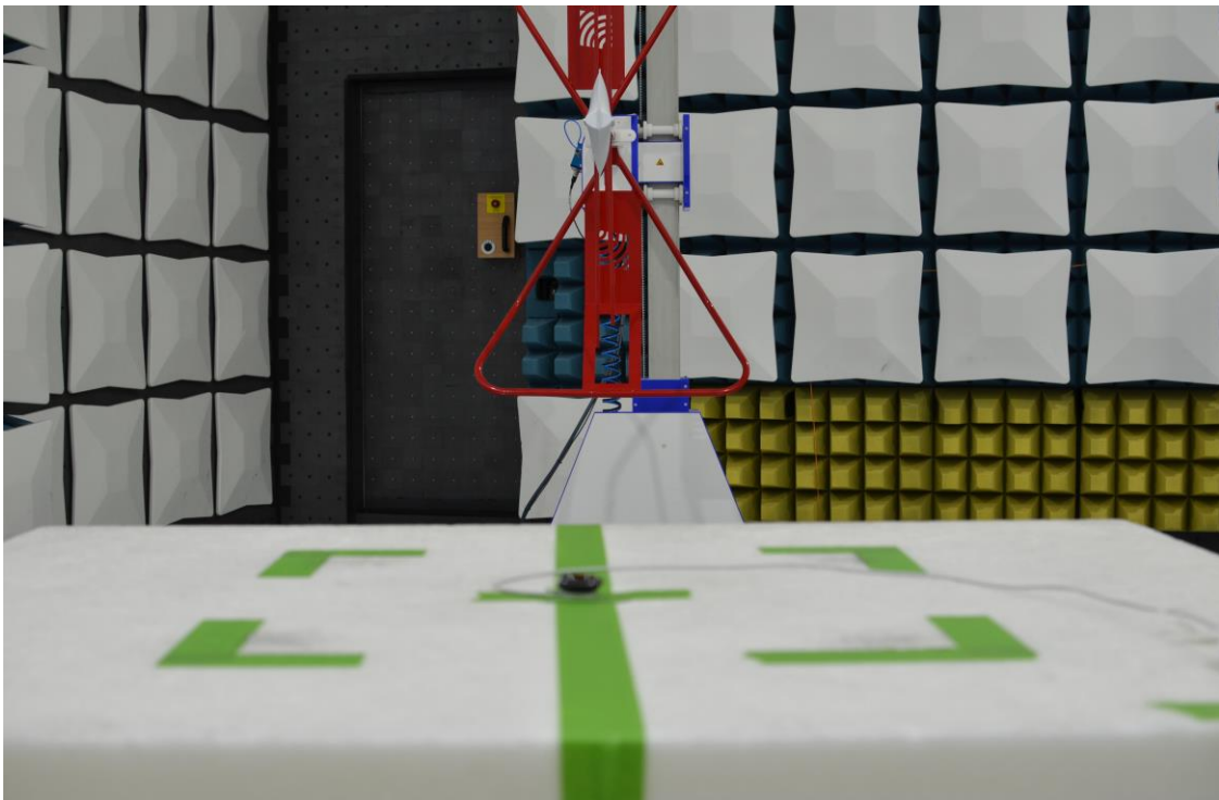
Figure 8: 30MHz-1GHz Test Setup (Rear View)
