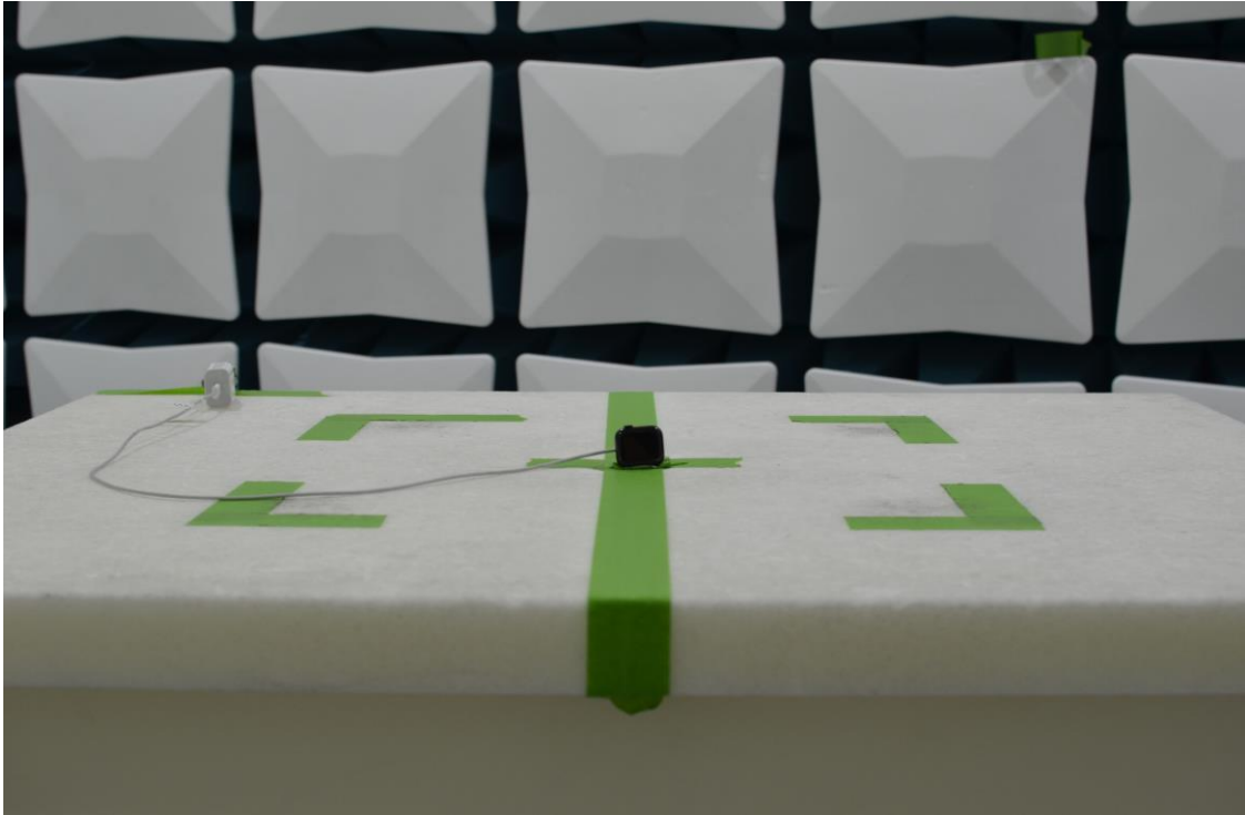
Figure 9: 30MHz-1GHz Test Setup (Front View)
