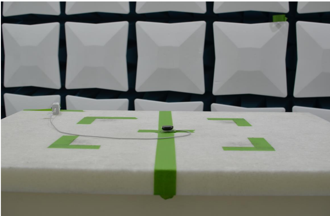
Figure 8: 30MHz-960MHz Test Setup (Front View)
