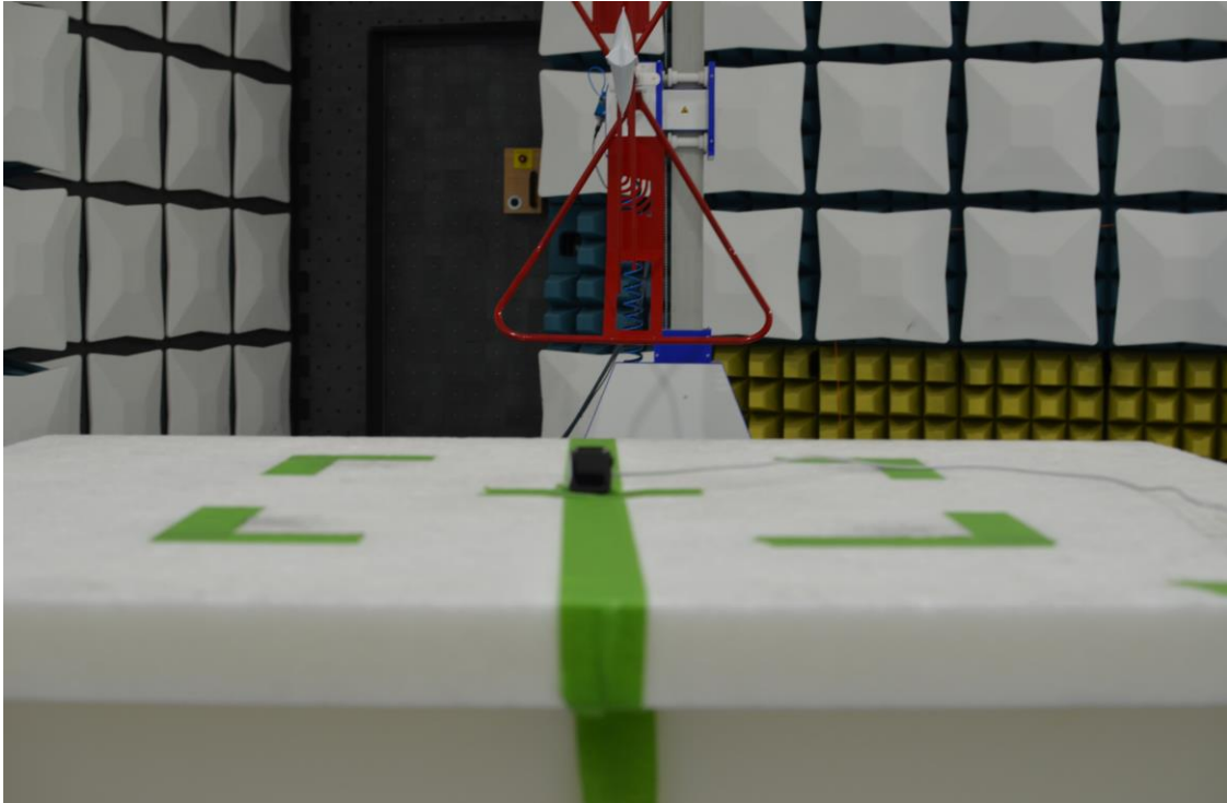
Figure 83: 30MHz-960MHz Test Setup (Rear View)
