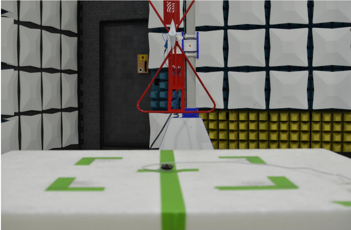
Figure 9: 30MHz-960MHz Test Setup (Rear View)
