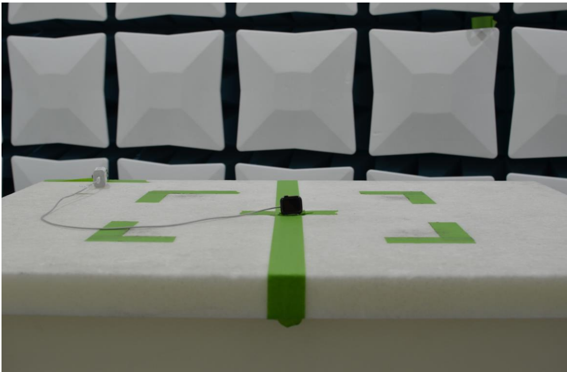
Figure 10: 30MHz-960MHz Test Setup (Front View)
