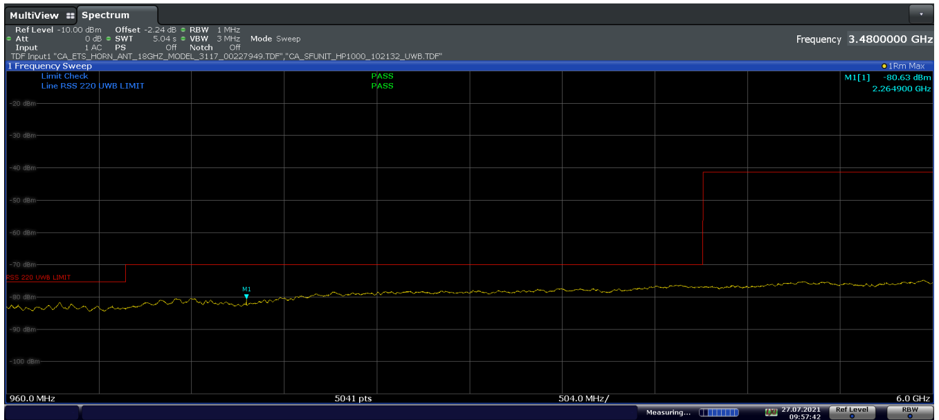
Plot 7-27. ISD Radiated Spurious Emission 960-6000MHz (Ch. 9, Config 3, Payload 125 Ant. Pol. H)
