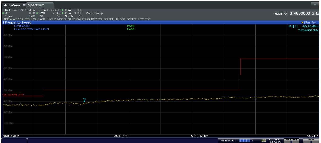
Plot 7-28. ISD Radiated Spurious Emission 960-6000MHz (Ch.9, Config 3, Payload 125 Ant. Pol. V)
