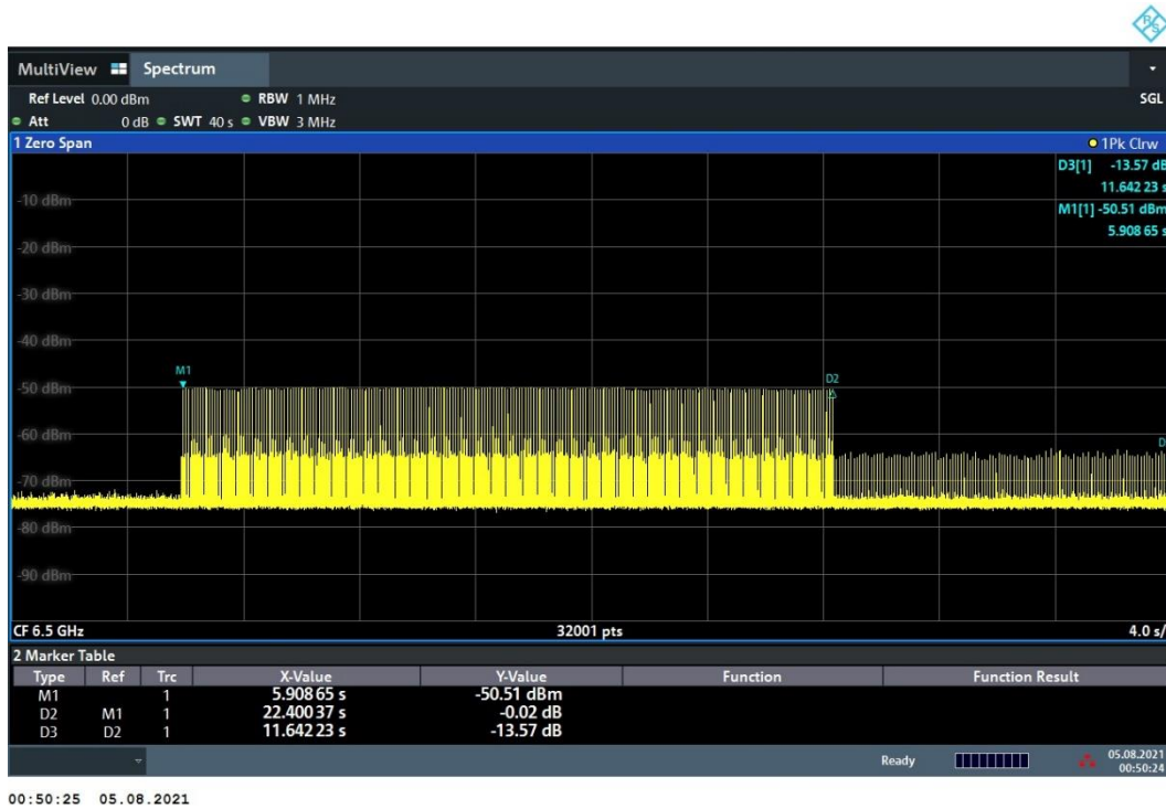
Plot 7-9. Cessation Time – Mode1 (Ch. 5, 6.5 GHz)
