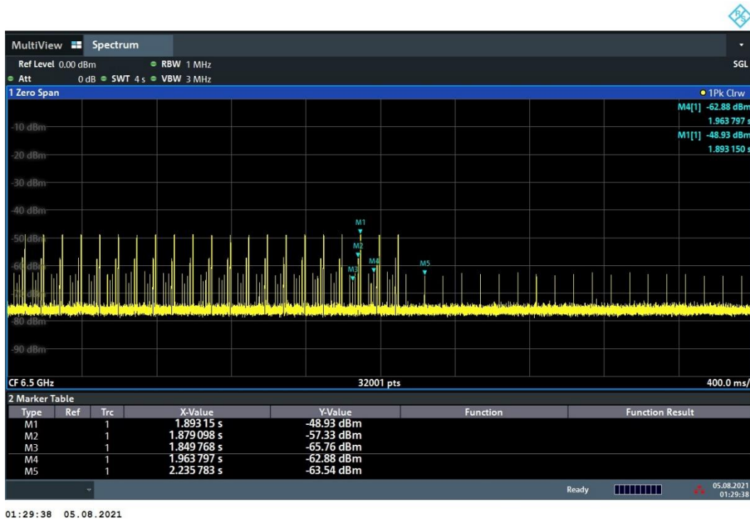
Plot 7-10. Zoom in Cessation Time – Mode1 (Ch. 5, 6.5 GHz)
