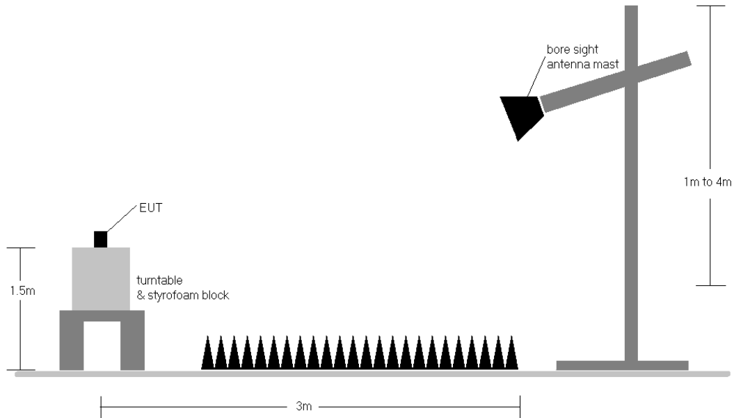
Figure 7-1. Test Setup
