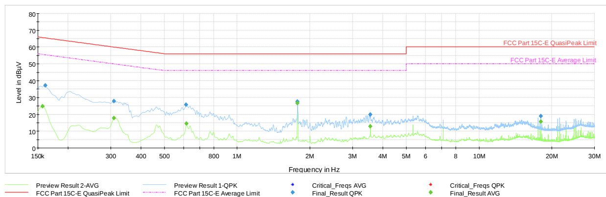
Plot 6-13. AC Line Conducted Plot (L1 - Mode 1, with AC/DC Adapter + Magnetic Charger)
