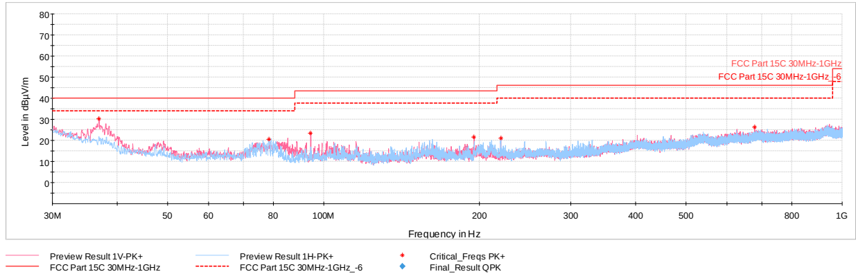
Plot 7-10. Radiated Spurious Emissions 30MHz – 1GHz (CE A 848kbps, with AC/DC Adapter and Magnetic Charger)
