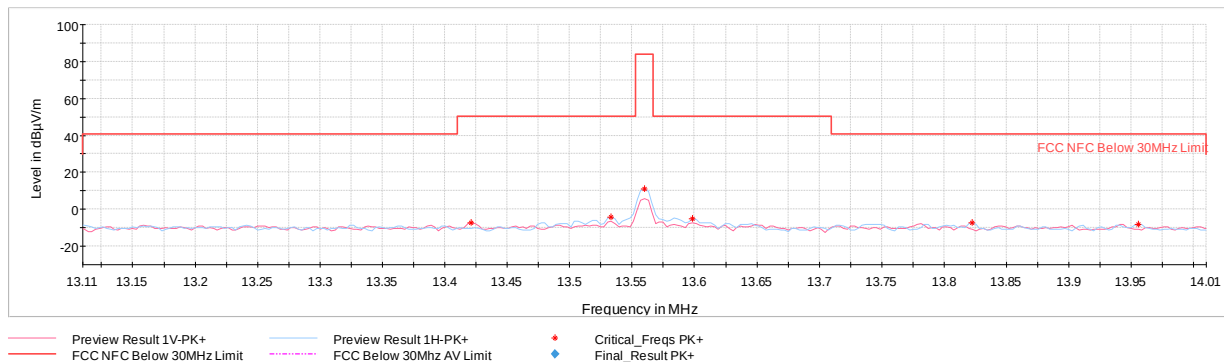
Plot 7-7. In Band Radiated Spurious Emissions (Reader 10% ASK 1 out of 256, AC/DC Adapter and Magnetic Charger)
