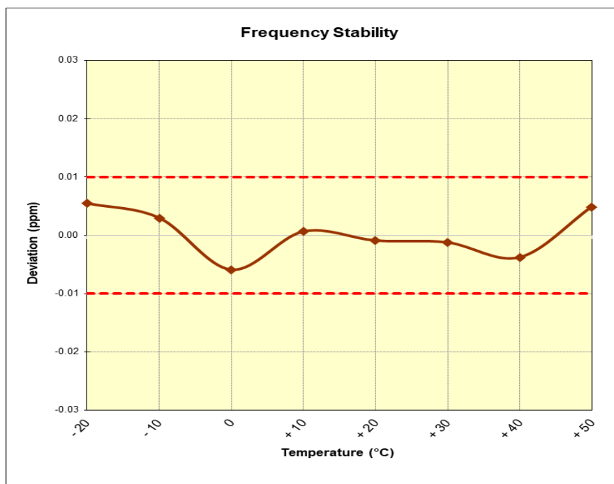
Figure 7-3. Frequency Stability Plot (CE A 848kbps)
