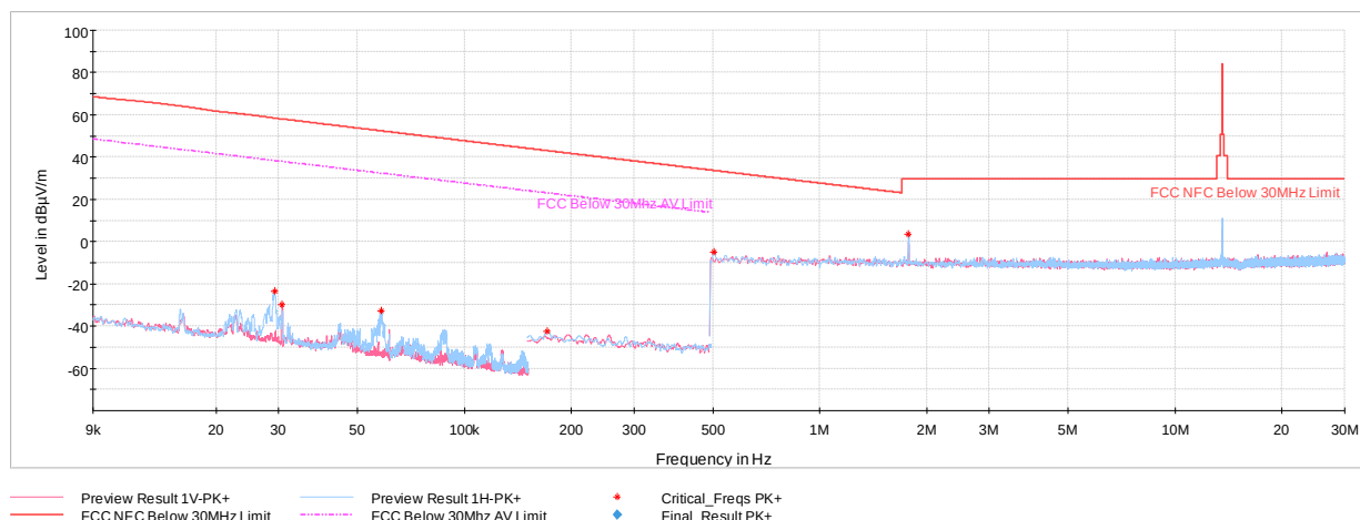
Plot 7-9. Radiated Spurious Emissions 9kHz – 30MHz (Reader 10% ASK 1 out of 256, with AC/DC Adapter and Magnetic Charger)
