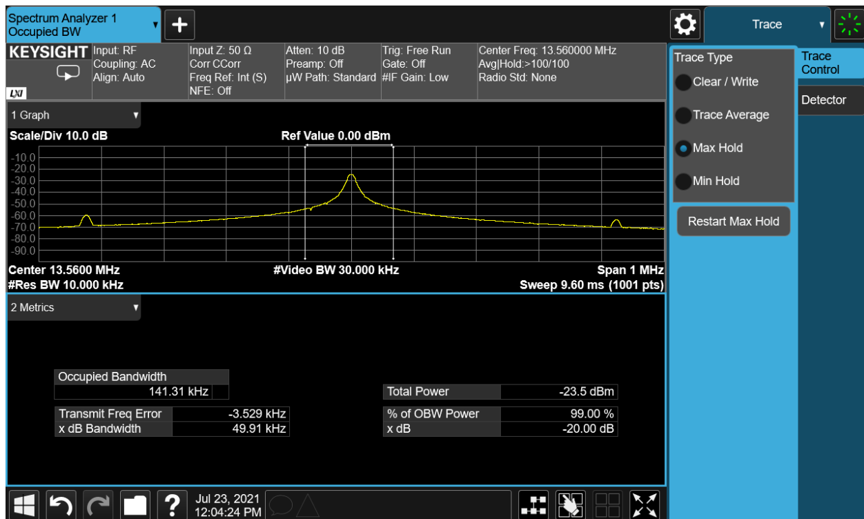
Plot 7-3. 20dB and 99% Bandwidth Plot (CE F 424kbps)
