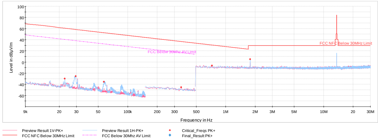
Plot 7-8. Radiated Spurious Emissions 9kHz – 30MHz (CE A 848kbps, with AC/DC Adapter and Magnetic Charger)
