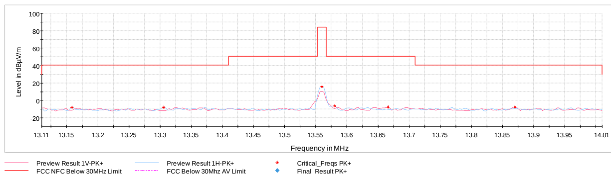
Plot 7-6. In Band Radiated Spurious Emissions (CE A 848kbps, with AC/DC Adapter and Magnetic Charger)
