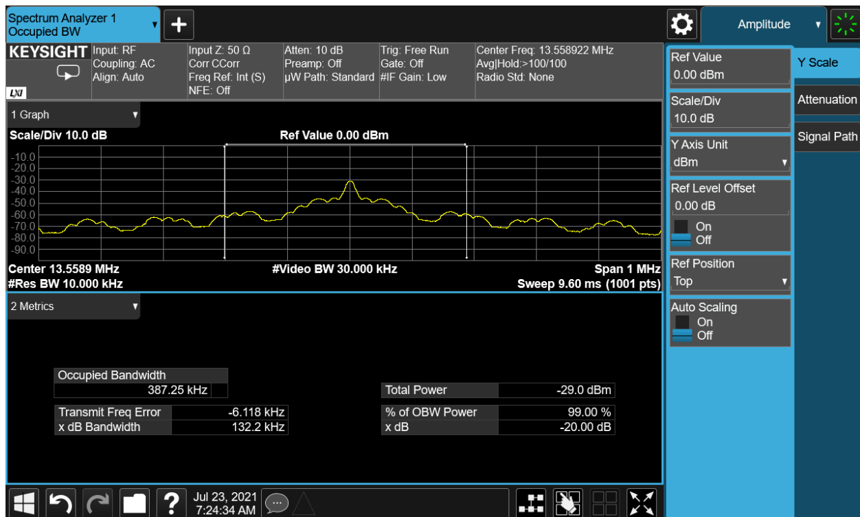
Plot 7-5. 20dB and 99% Bandwidth Plot (Reader 10% ASK 1 out of 256)
