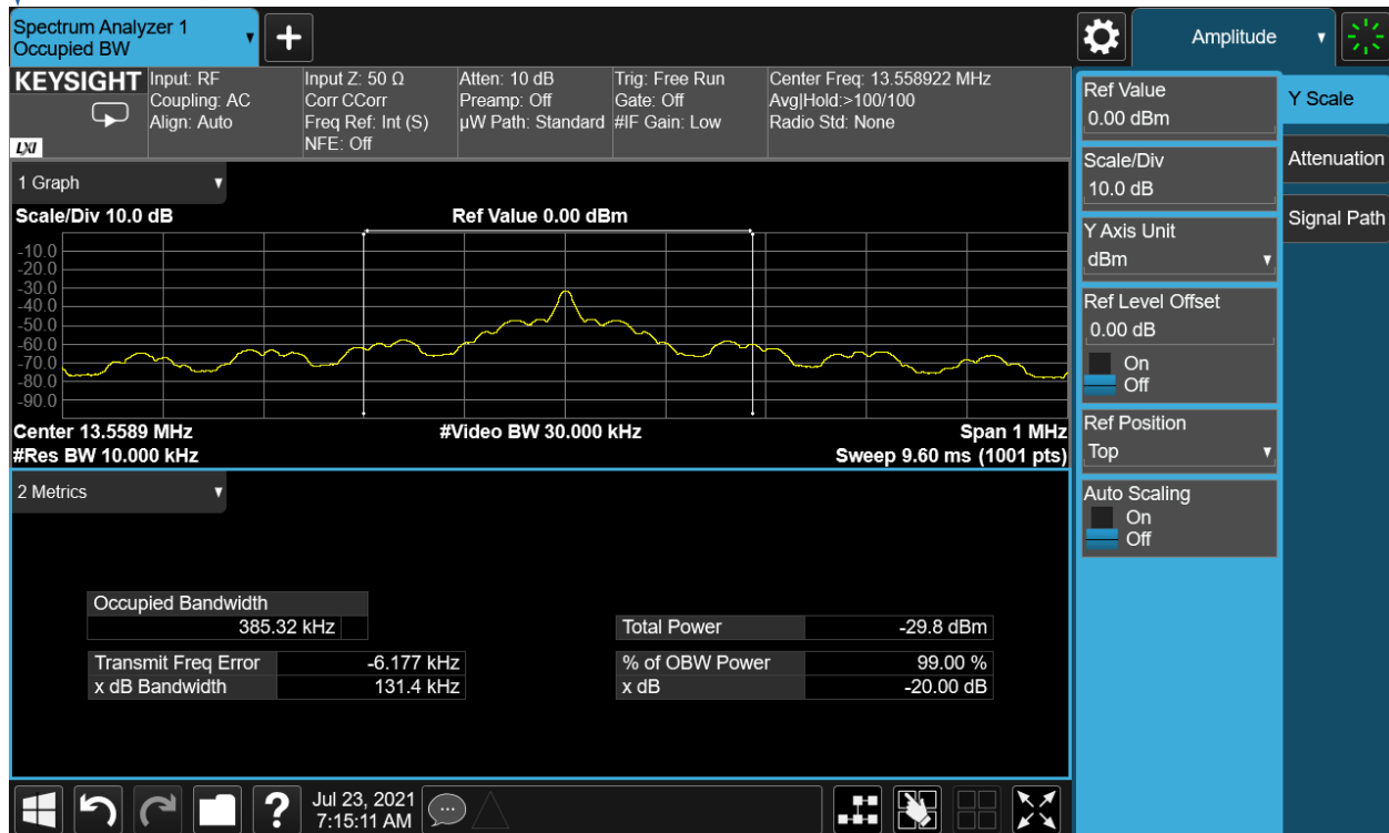
Plot 7-4. 20dB and 99% Bandwidth Plot (Reader 10% ASK 1 out of 4)
