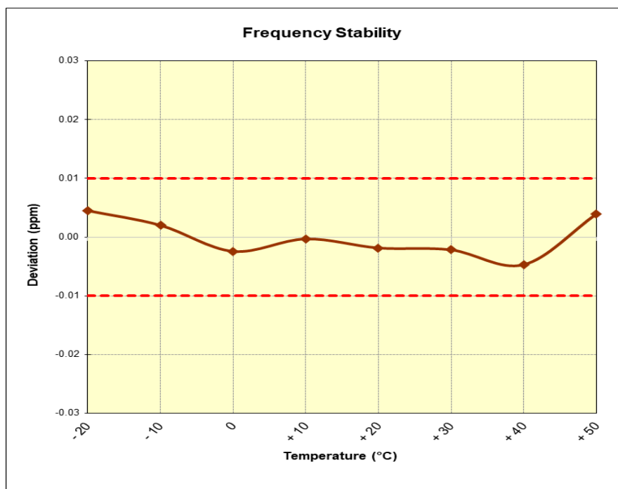
Figure 7-4. Frequency Stability Plot (Reader 10% ASK 1 out of 256)
