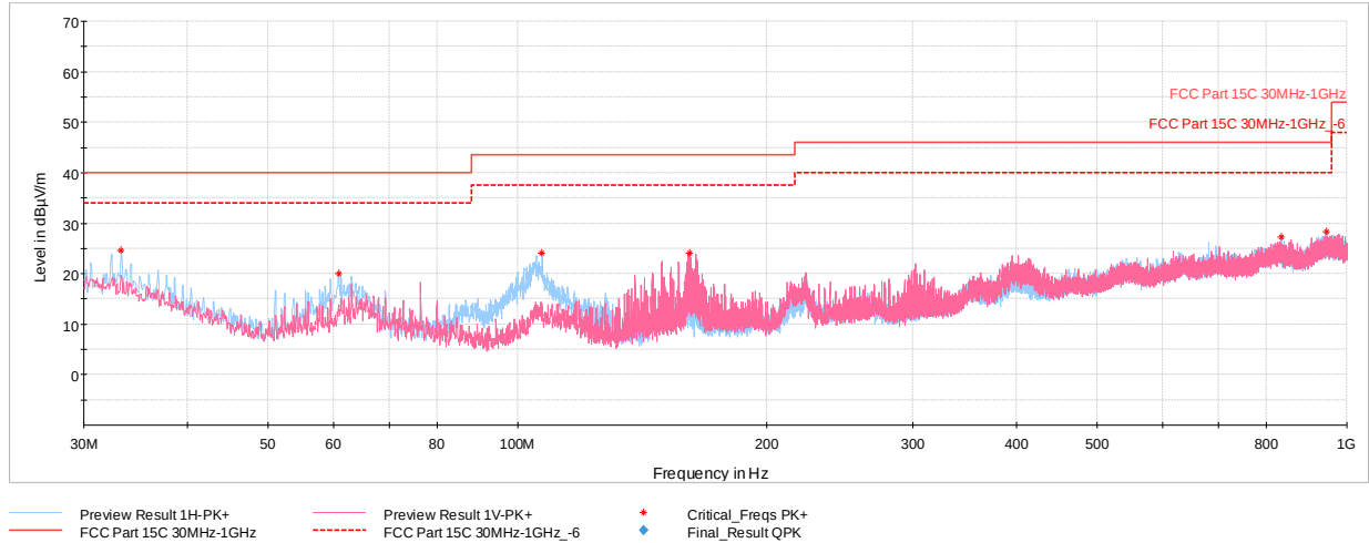
Plot 7-11. Radiated Spurious Emissions 30MHz – 1GHz (Reader 10% ASK 1 out of 256, with AC/DC Adapter and Magnetic Charger)
