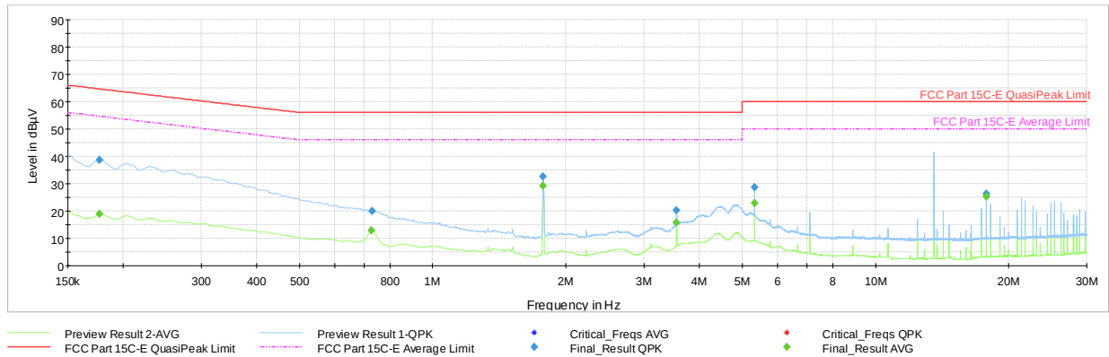
Plot 7-13. AC Line-Conducted Plot (N, CE A 848kbps, with AC/DC Adapter and Magnetic Charger)
