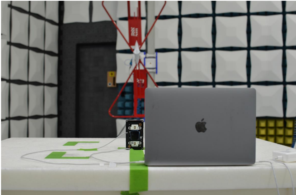
Figure 17: 30MHz-1GHz Test Setup (Rear View)
