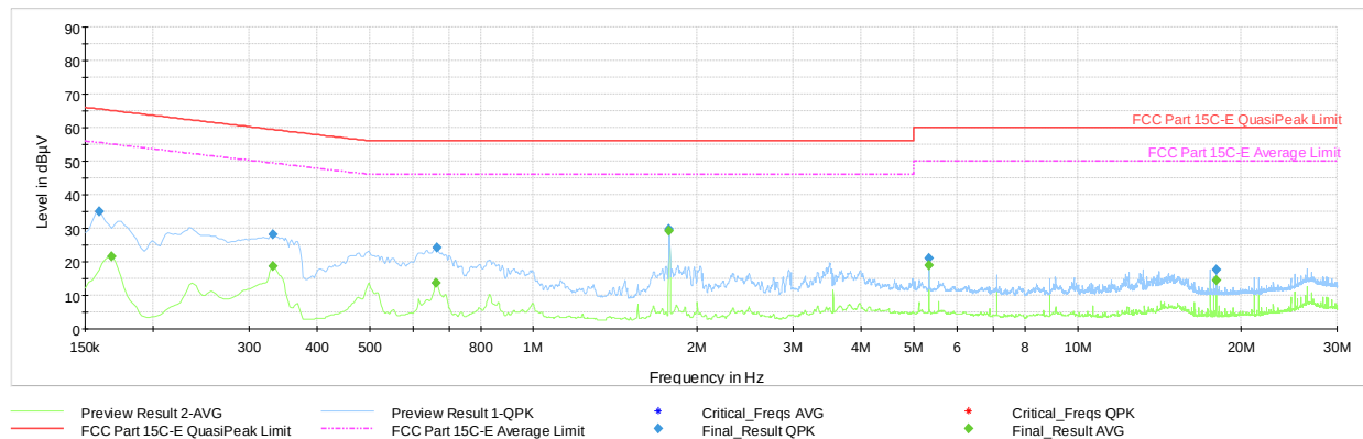
Plot 6-14. AC Line Conducted Plot (N - Mode 1, with AC/DC Adapter + Magnetic Charger)
