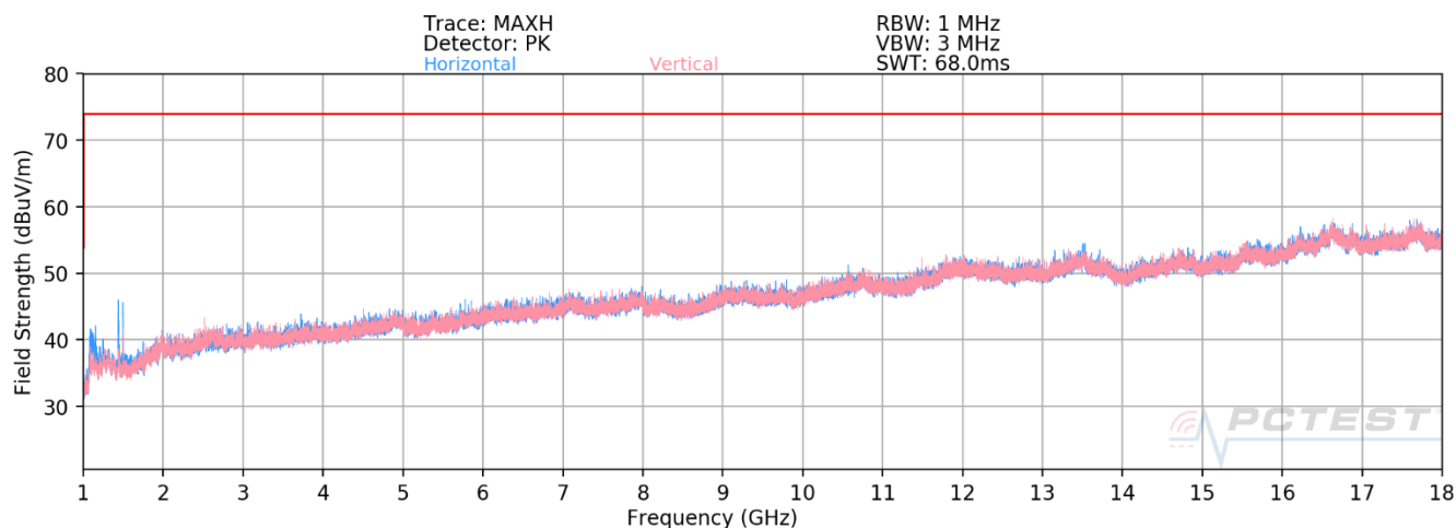
Plot 6-10. Radiated Spurious Emissions 1GHz – 18GHz (Mode 1)
