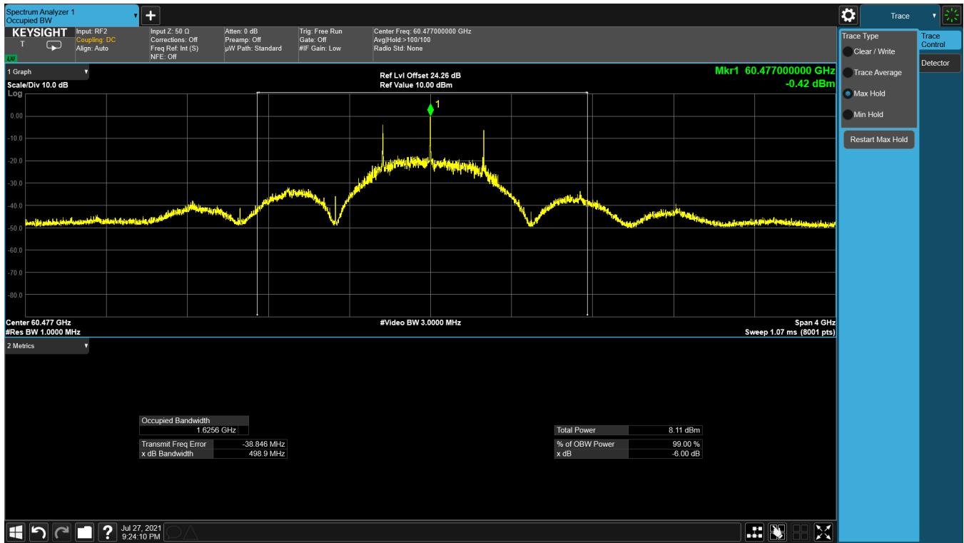
Plot 6-2. 99% Occupied Bandwidth Measurement (Mode 1)
