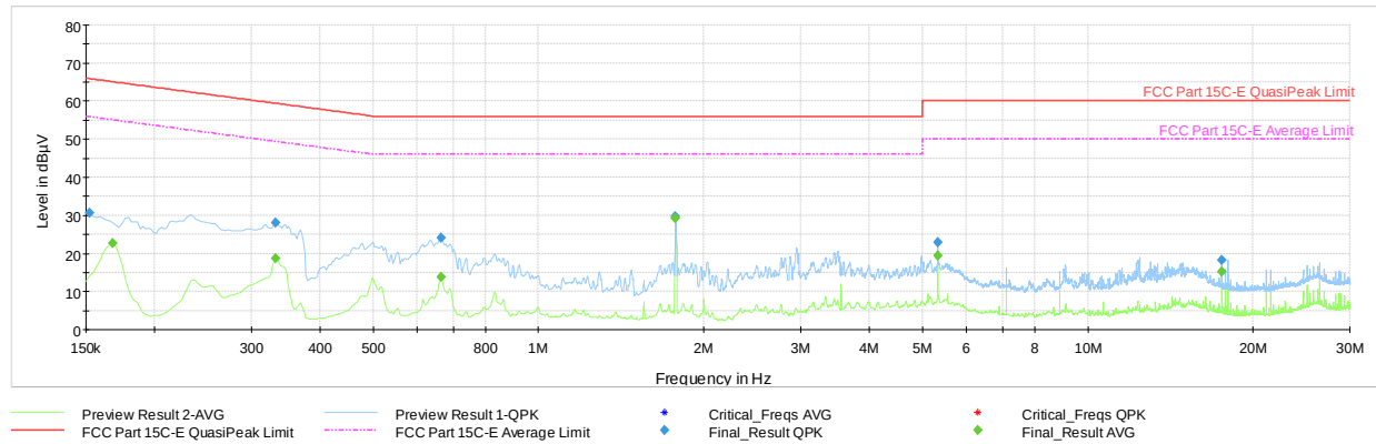
Plot 6-13. AC Line Conducted Plot (L1 - Mode 1, with AC/DC Adapter + Magnetic Charger)
