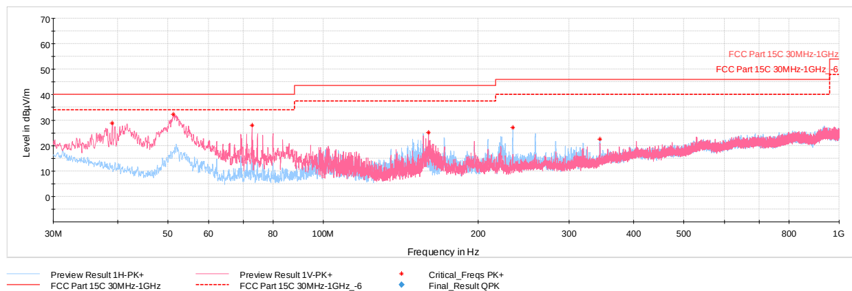
Plot 6-12. Radiated Spurious Emissions 30MHz – 1GHz (Mode 1, with AC/DC Adapter + Magnetic Charger)
