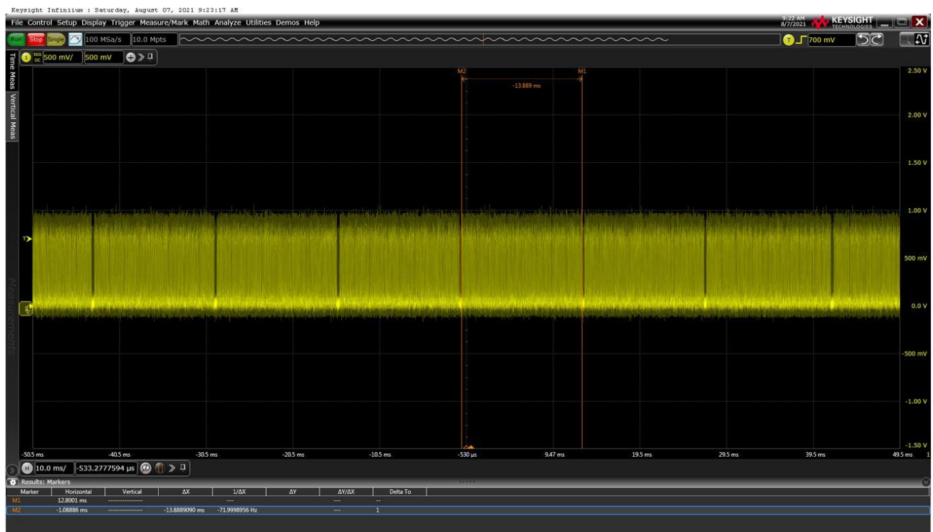
Plot 6-3. EUT RF Pulse Train (Mode 1)
