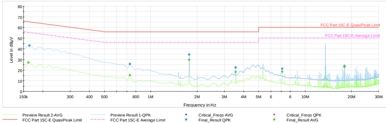
Plot 7-14. AC Line-Conducted Plot (L1, Reader 10% ASK 1 out of 256, with AC/DC Adapter and Magnetic Charger)
