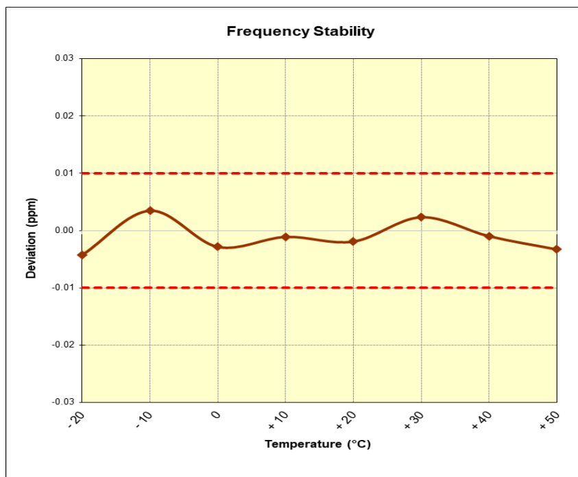
Figure 7-4. Frequency Stability Plot (Reader 10% ASK 1 out of 256)
