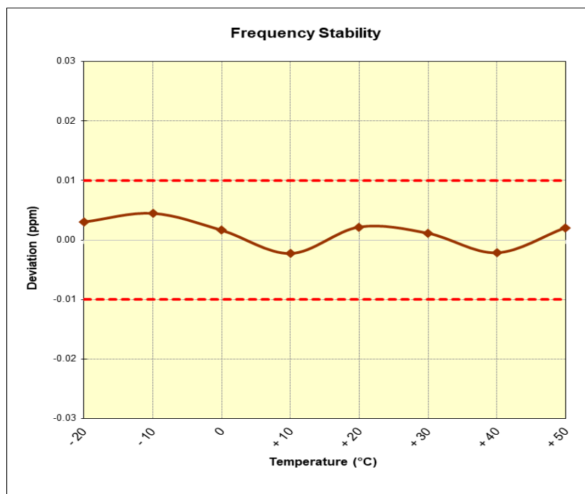
Figure 7-3. Frequency Stability Plot (CE A 848kbps)
