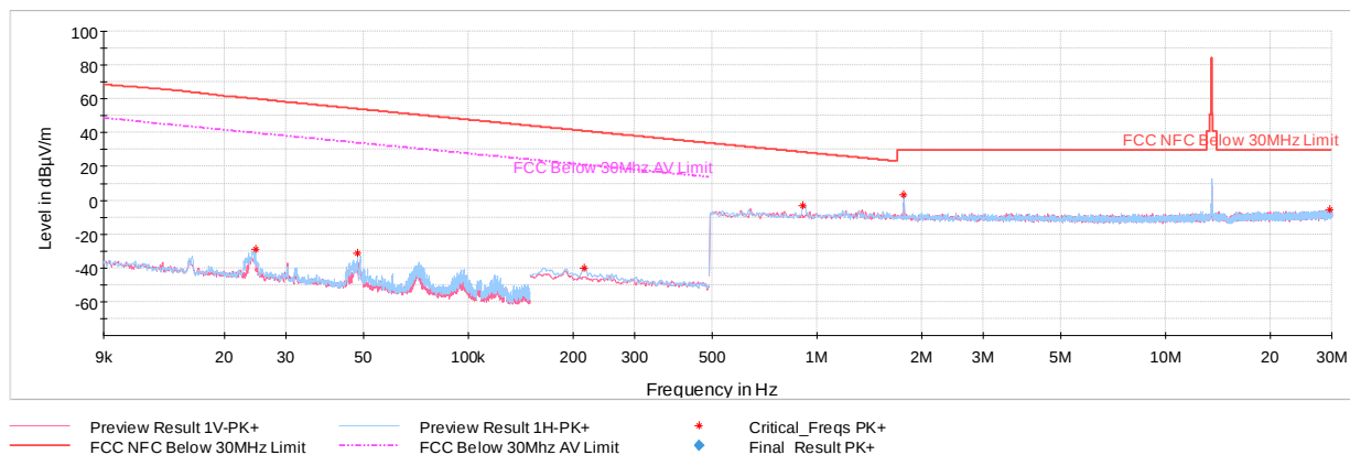
Plot 7-9. Radiated Spurious Emissions 9kHz – 30MHz (Reader 10% ASK 1 out of 256, with AC/DC Adapter and Magnetic Charger)
