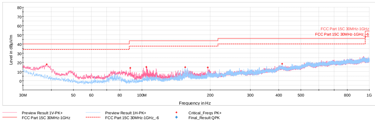
Plot 7-11. Radiated Spurious Emissions 30MHz – 1GHz (Reader 10% ASK 1 out of 256, with AC/DC Adapter and Magnetic Charger)
