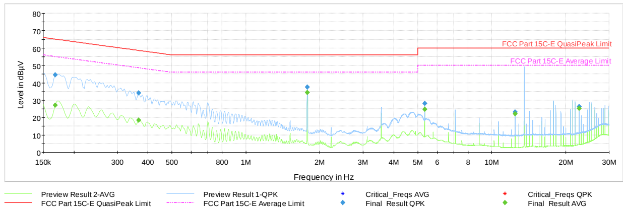
Plot 7-12. AC Line-Conducted Plot (L1, CE A 848kbps, with AC/DC Adapter and Magnetic Charger)
