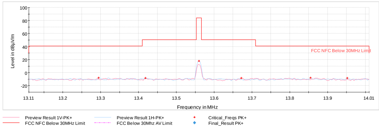
Plot 7-6. In Band Radiated Spurious Emissions (CE A 848kbps, with AC/DC Adapter and Magnetic Charger)
