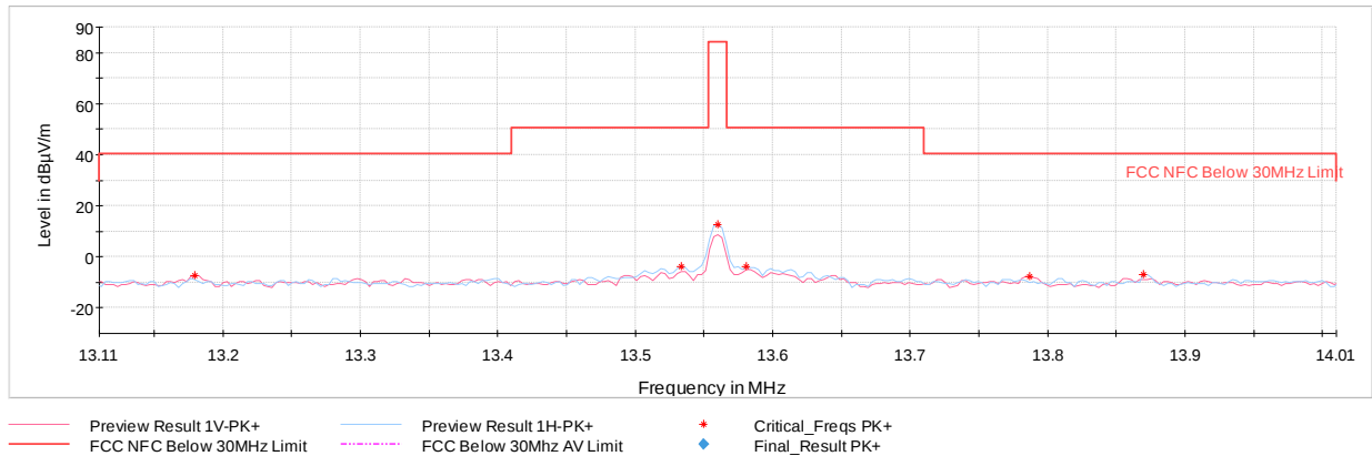
Plot 7-7. In Band Radiated Spurious Emissions (Reader 10% ASK 1 out of 256, AC/DC Adapter and Magnetic Charger)
