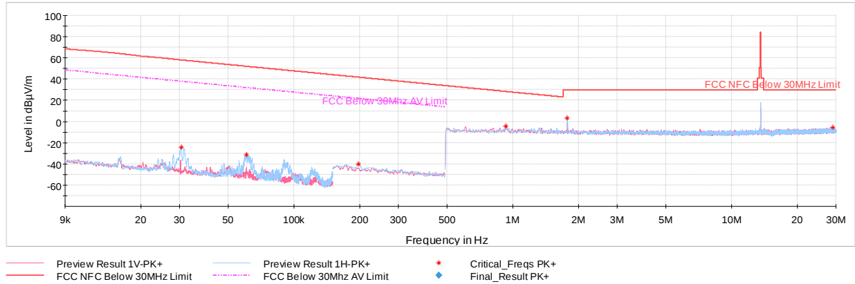
Plot 7-8. Radiated Spurious Emissions 9kHz – 30MHz (CE A 848kbps, with AC/DC Adapter and Magnetic Charger)
