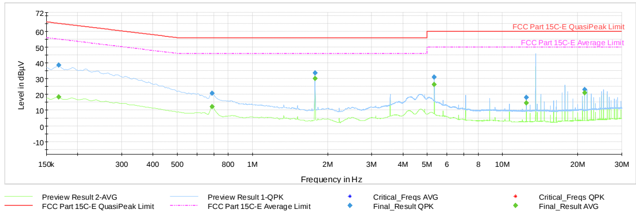
Plot 7-13. AC Line-Conducted Plot (N, CE A 848kbps, with AC/DC Adapter and Magnetic Charger)
