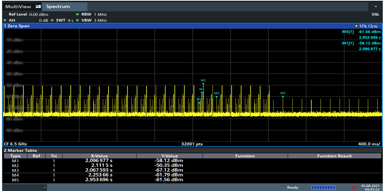
Plot 7-10. Zoom in Cessation Time – Mode1 (Ch. 5, 6.5 GHz)
