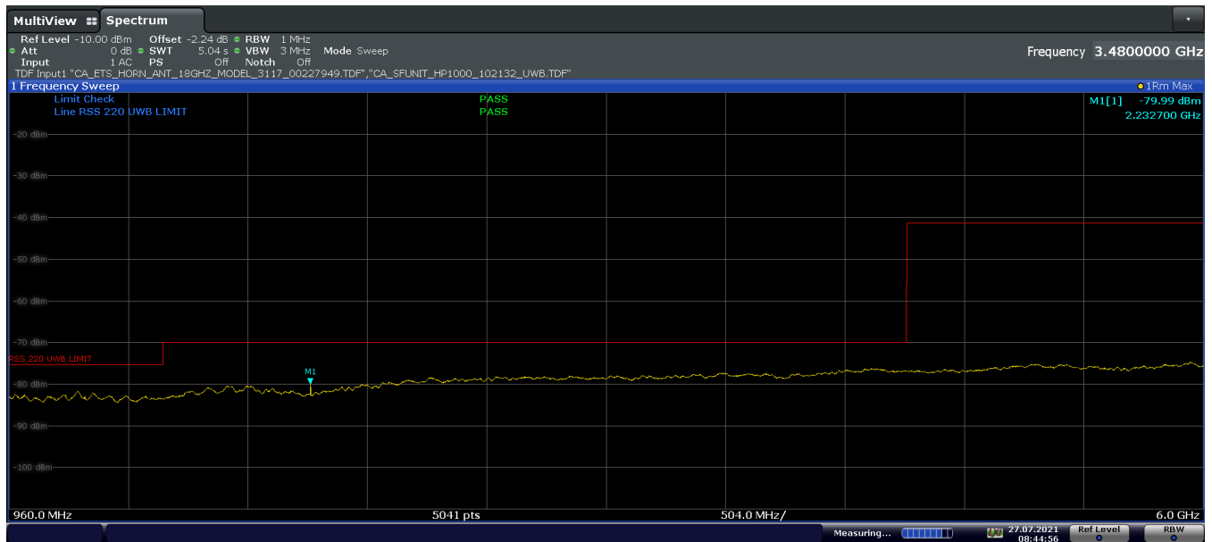
Plot 7-27. ISSED Radiated Spurious Emission 960-6000MHz (Ch. 9, Config 3, Payload 125 Ant. Pol. H)
