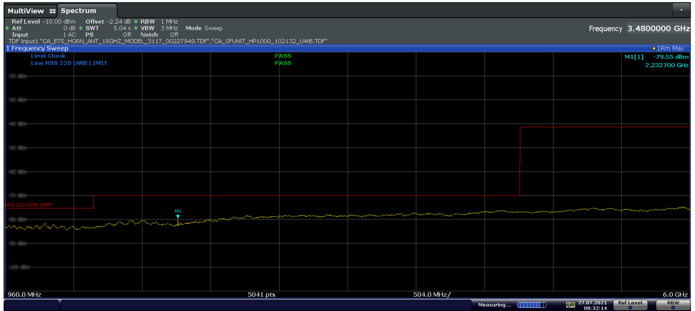
Plot 7-17. ISSED Radiated Spurious Emission 960-6000MHz (Ch. 5, Config 3, Payload 125 Ant. Pol. H)
