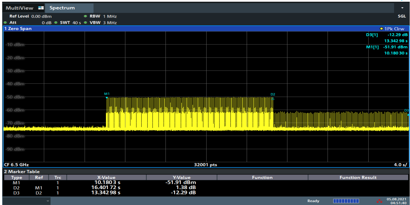
Plot 7-9. Cessation Time – Mode1 (Ch. 5, 6.5 GHz)
