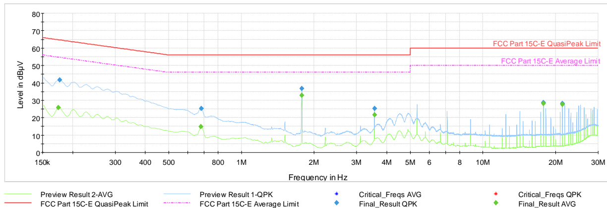
Plot 7-41. AC Line Conducted (Ch. 5, Config 3, Payload 125 L1, with AC/DC Adapter + Magnetic Charger)
