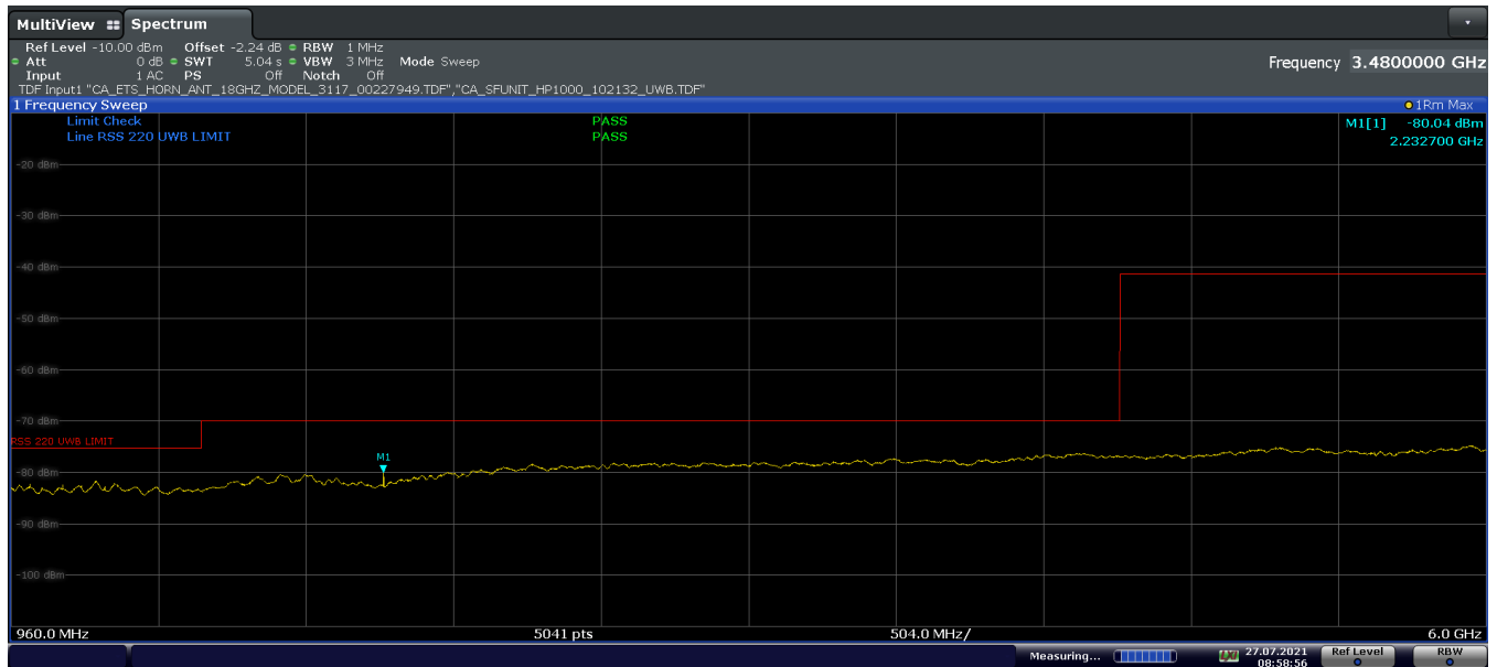
Plot 7-28. ISSED Radiated Spurious Emission 960-6000MHz (Ch.9, Config 3, Payload 125 Ant. Pol. V)
