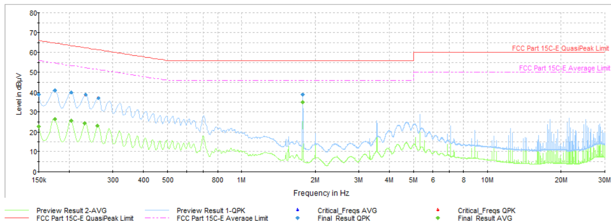
Plot 7-43.AC Line-Conducted Test Plot (L1, with AC/DC Adapter + Magnetic Charger)
