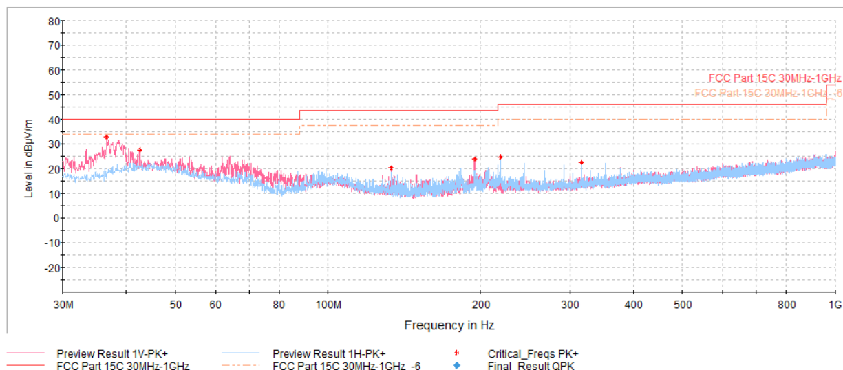
Plot 7-42. Radiated Spurious Plot below 1GHz (2.4GHz – 5GHz), with AC/DC Adapter and Magnetic Charger.
