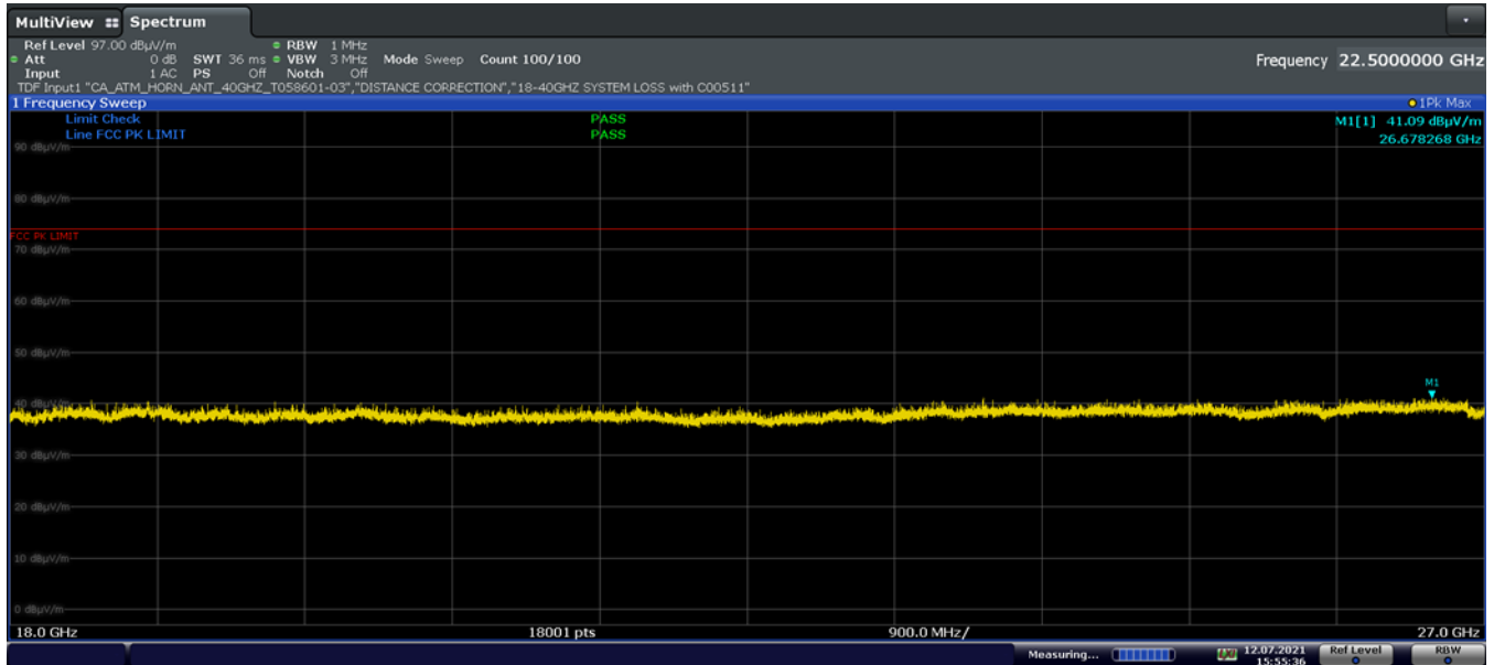
Plot 7-32. Radiated Spurious Plot above 18GHz (GFSK ePA – Ch.78, Pol. H)
