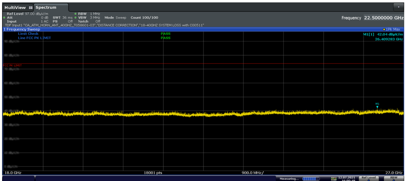
Plot 7-33. Radiated Spurious Plot above 18GHz (GFSK ePA – Ch.78, Pol. V)
