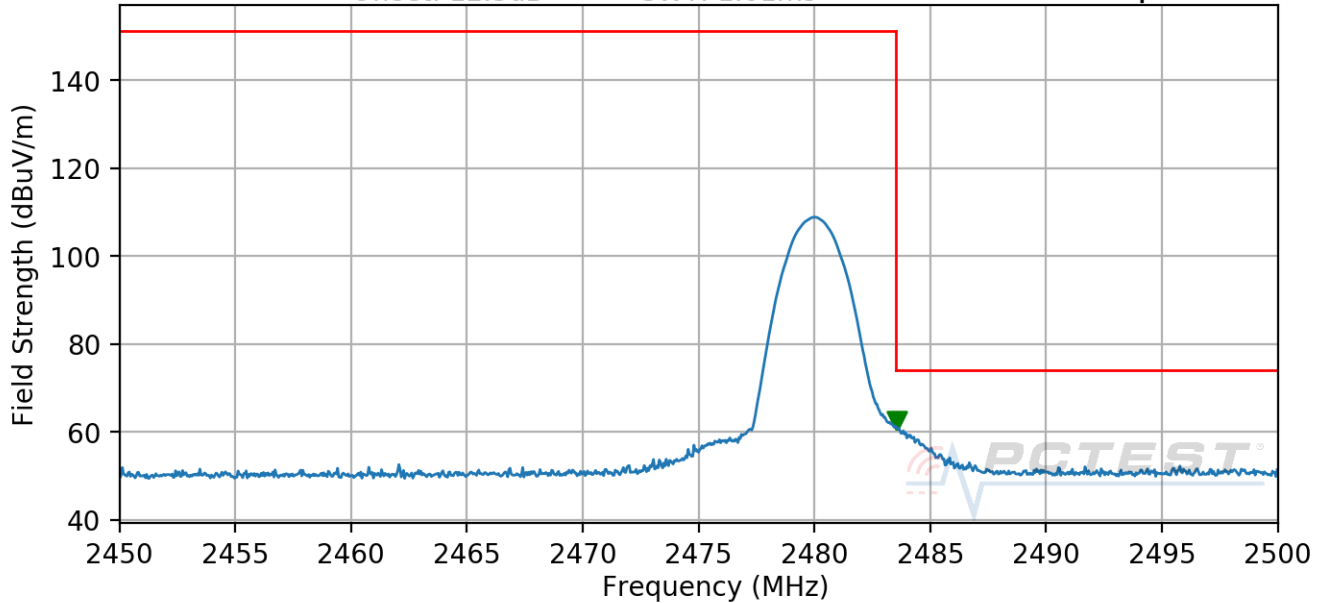
Plot 7-40. Radiated Restricted Upper Band Edge Measurement (Peak)
