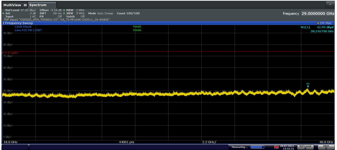
Plot 7-35. Radiated Spurious Plot 18GHz – 40GHz (2.4GHz – 5GHz) Pol. H
