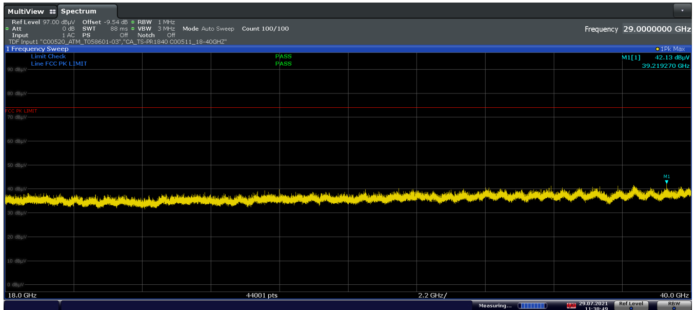
Plot 7-36. Radiated Spurious Plot 18GHz – 40GHz (2.4GHz – 5GHz) Pol. V
