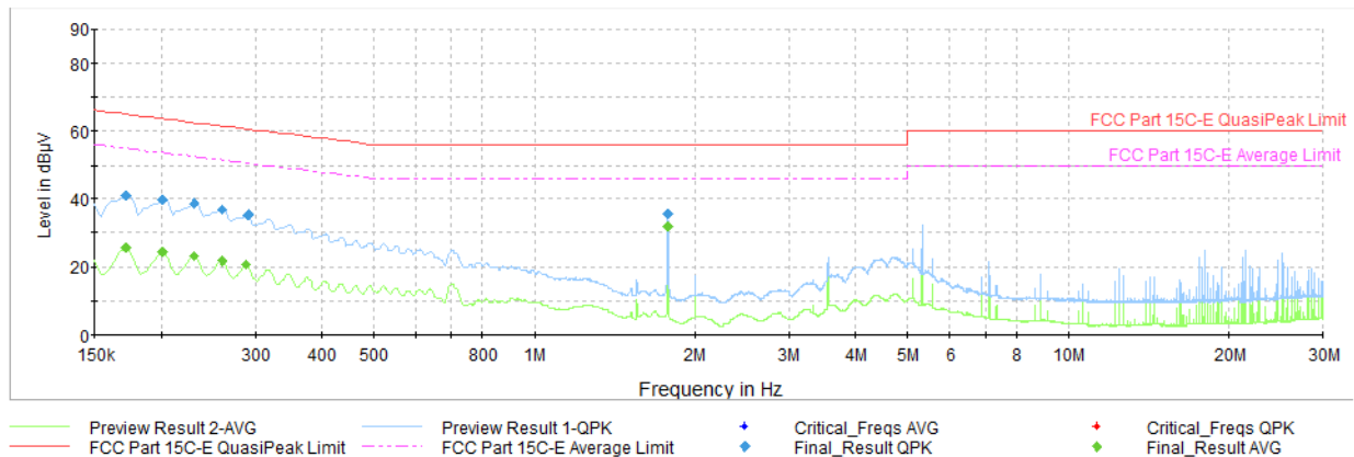
Plot 7-44.AC Line-Conducted Test Plot (N, with AC/DC Adapter + Magnetic Charger)
