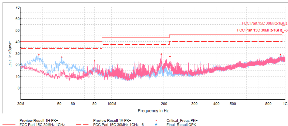
Plot 7-41. Radiated Spurious Plot below 1GHz (GFSK ePA – Ch.78, Pol. H & V, with AC/DC Adapter and Magnetic Charger)
