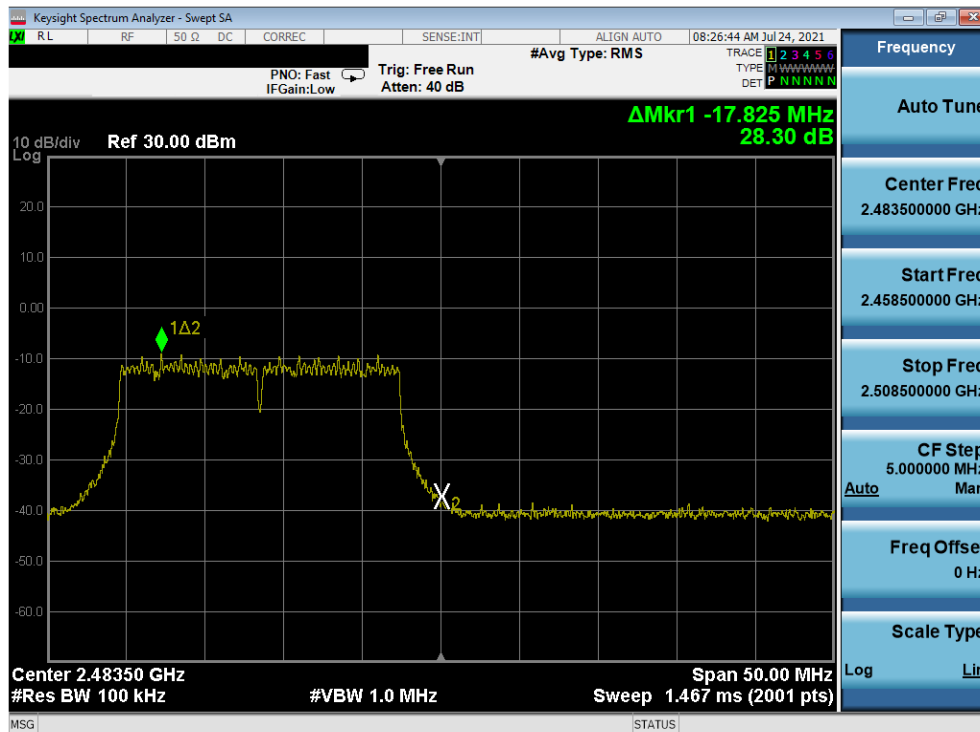
Plot 7-44. Band Edge Plot (802.11n MCS7 – Ch. 13)
