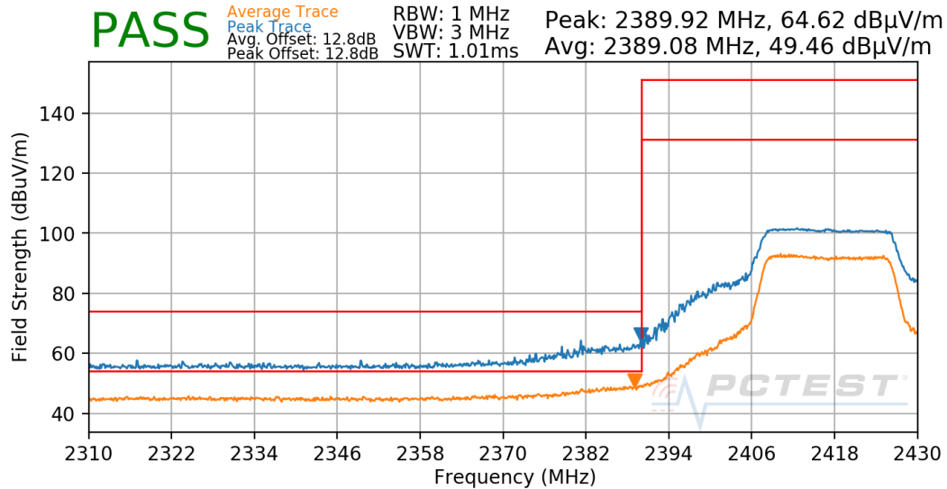
Plot 7-60. Radiated Restricted Lower Band Edge Measurement
