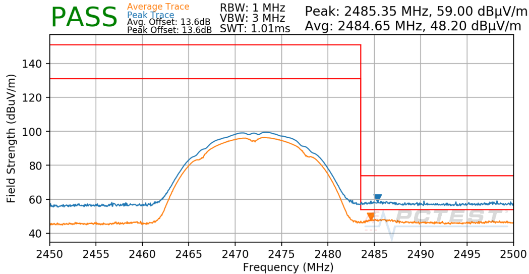
Plot 7-58. Radiated Restricted Upper Band Edge Measurement
