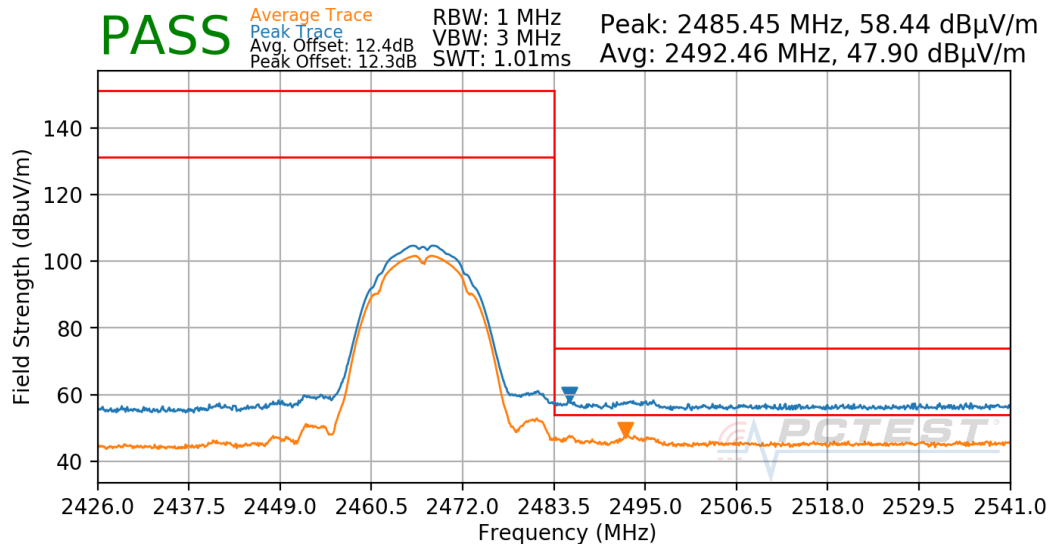
Plot 7-57. Radiated Restricted Upper Band Edge Measurement
