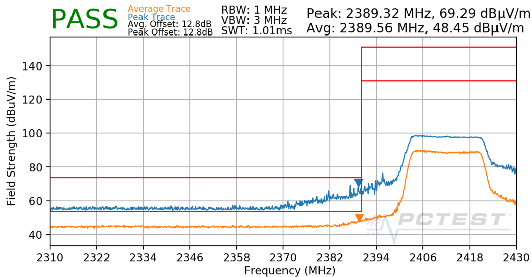
Plot 7-59. Radiated Restricted Lower Band Edge Measurement
