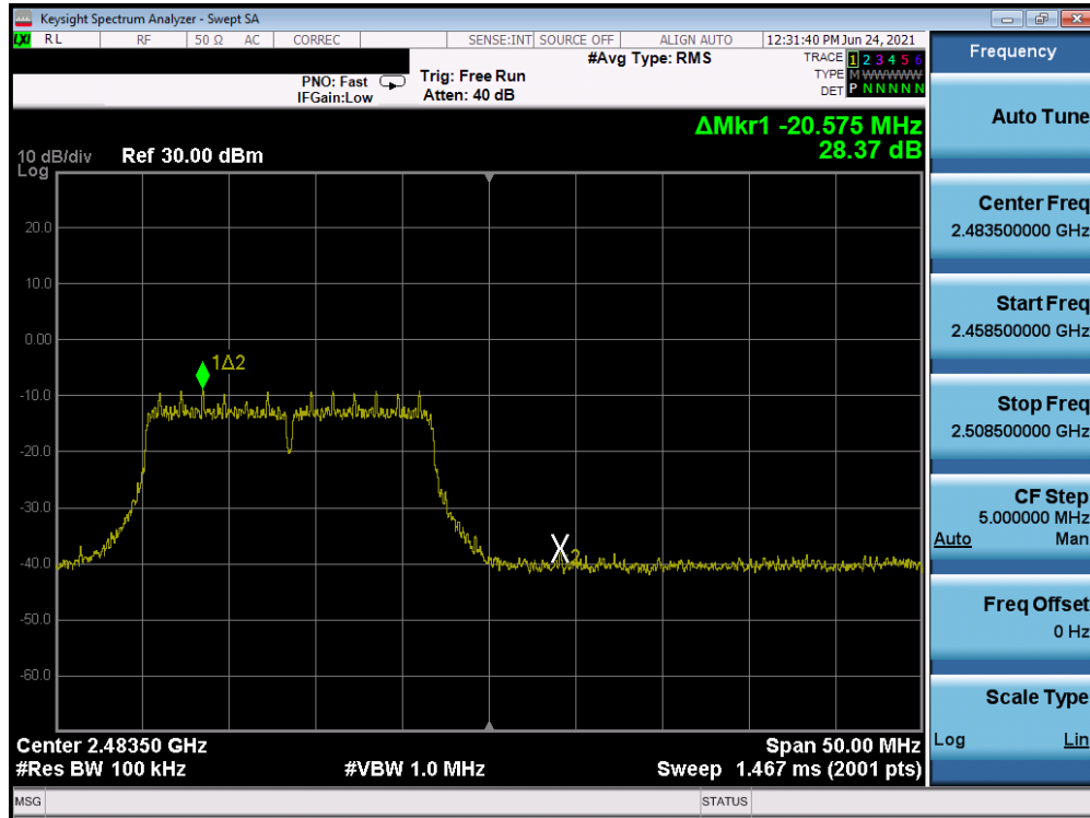
Plot 7-33. Band Edge Plot (802.11g – Ch. 13)
