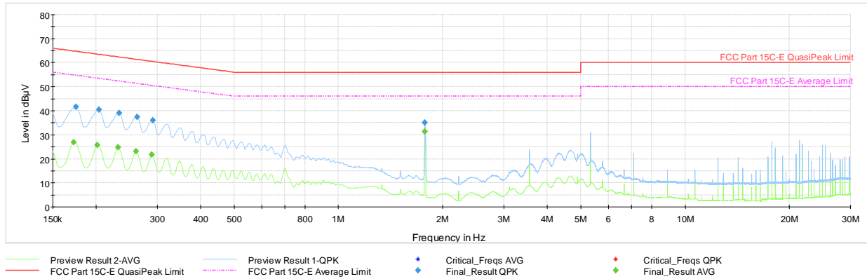
Plot 7-71.AC Line Conducted Plot 802.11b – Ch.1 (L1), with AC/DC Adapter and Magnetic Charger
