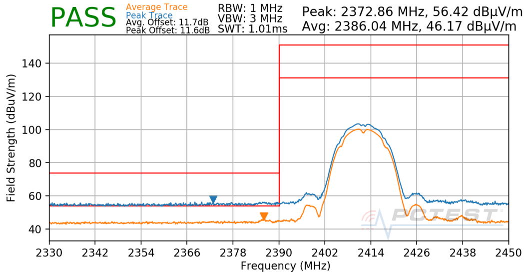
Plot 7-56. Radiated Restricted Lower Band Edge Measurement
