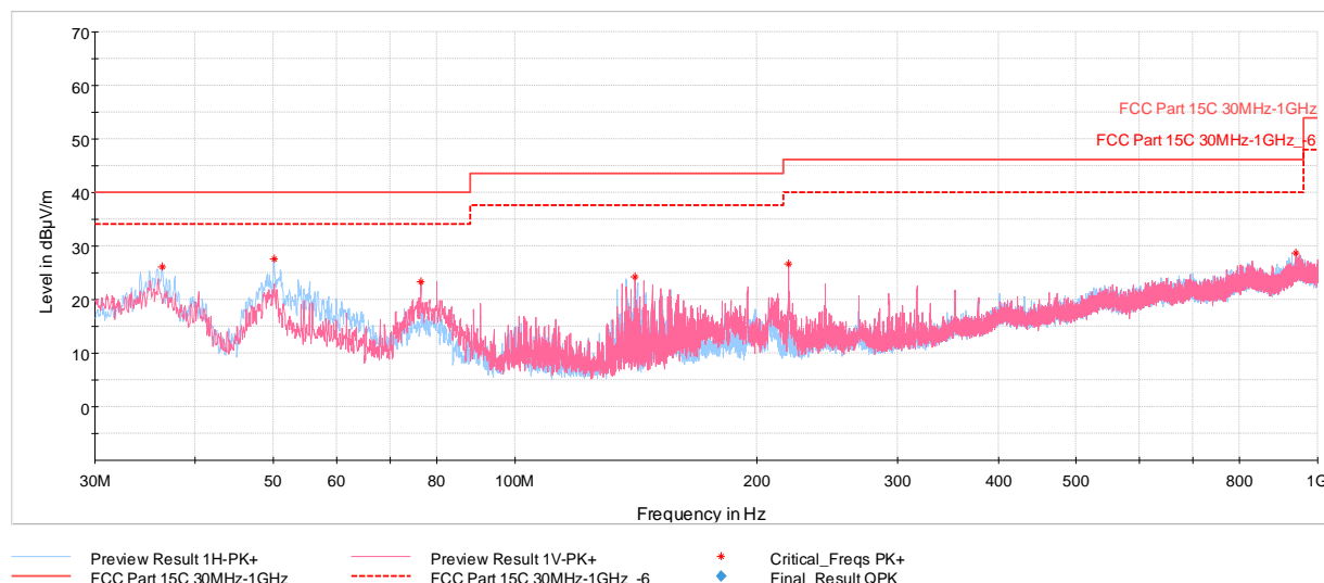
Plot 7-70. Radiated Spurious Emissions 30MHz-1GHz (802.11b – Ch.1, with AC/DC Adapter and Magnetic Charger
