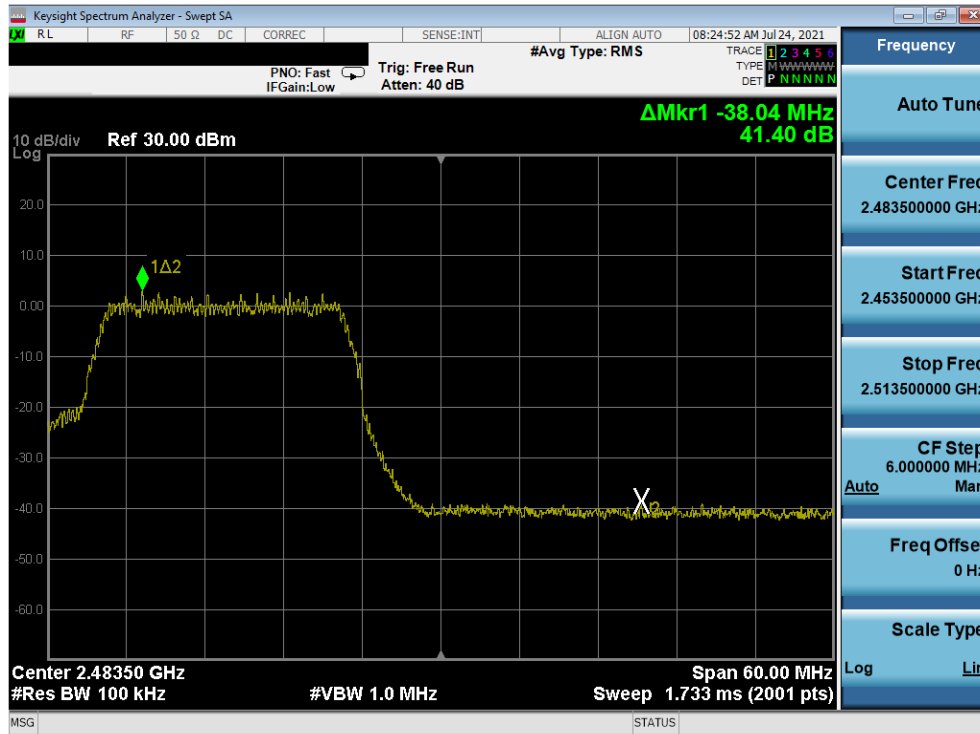
Plot 7-43. Band Edge Plot (802.11n MCS7 – Ch. 12)
