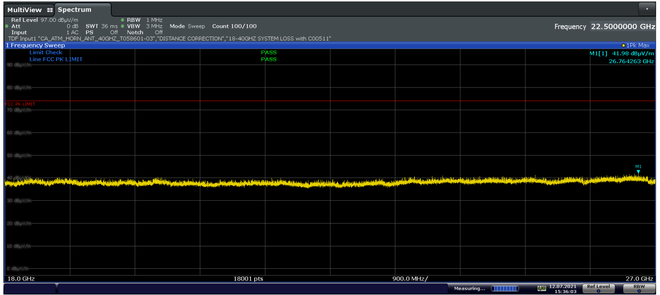
Plot 7-54. Radiated Spurious Plot above 18GHz (802.11b – Ch. 1 Pol H)
