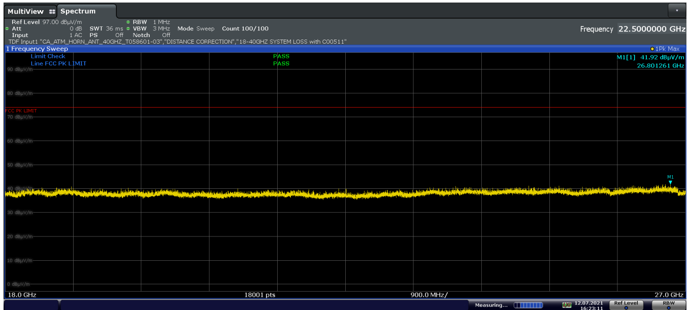
Plot 7-33. Radiated Spurious Plot above 18GHz (4Mbps, HDR4, ePA – Ch. 75, Ant. Pol V)
