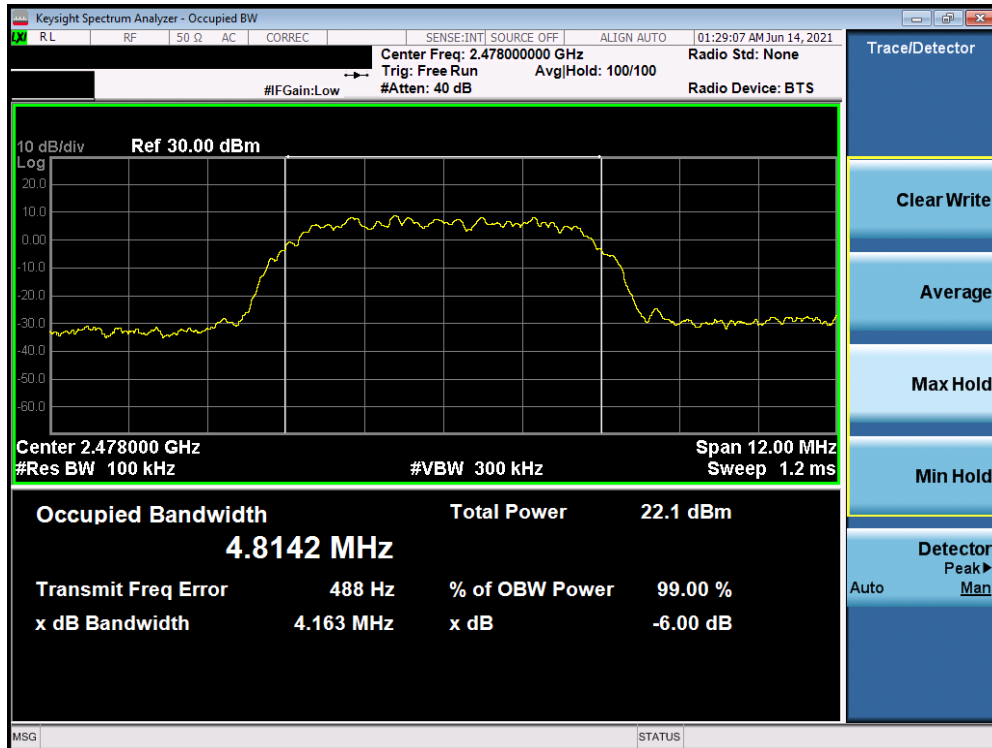
Plot 7-6. 6dB Bandwidth & 99% OBW Plot (Bluetooth (HDR8), 8Mbps, ePA – Ch. 75)
