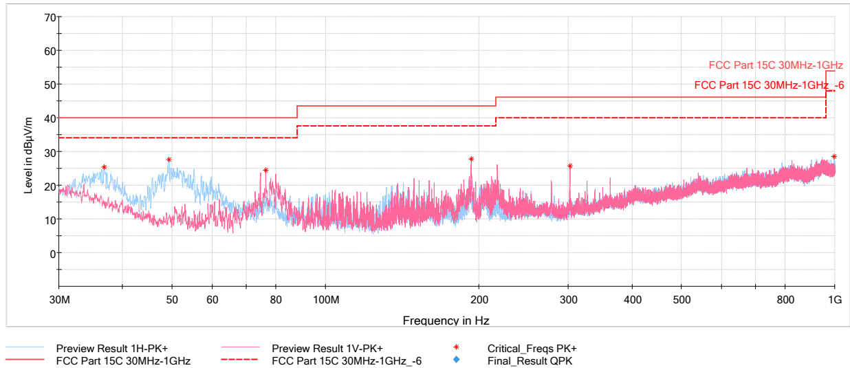
Plot 7-38. Radiated Spurious Emissions Plot below 1GHz (4Mbps, ePA – Ch. 38, Pol. H & V, with (AC/DC Adapter + Magnetic Charger)
