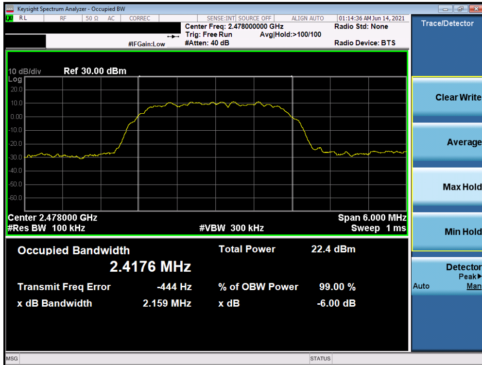
Plot 7-3. 6dB Bandwidth & 99% OBW Plot (Bluetooth (HDR4), 4Mbps, ePA – Ch. 75)
