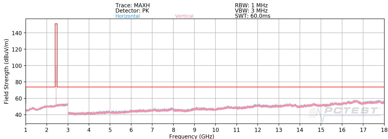
Plot 7-30. Radiated Spurious Emissions Above 1GHz (4Mbps, HDR4, ePA – Ch. 38, Ant. Pol. H & V)
