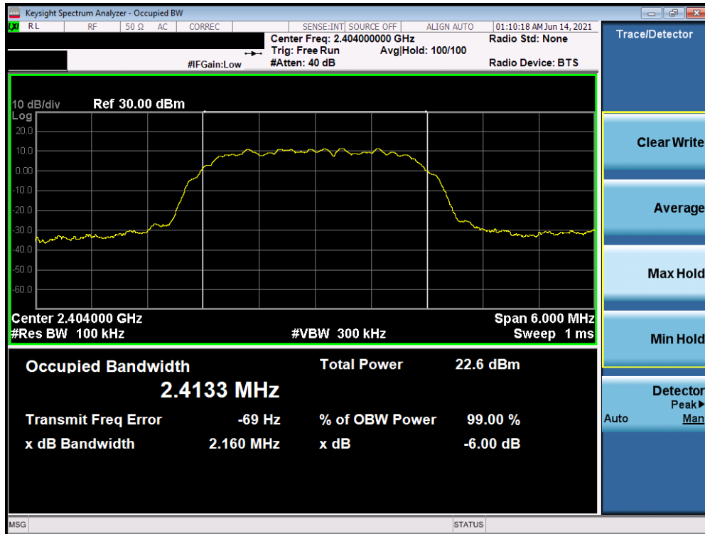
Plot 7-1. 6dB Bandwidth & 99% OBW Plot (Bluetooth (HDR4), 4Mbps, ePA – Ch. 1)
