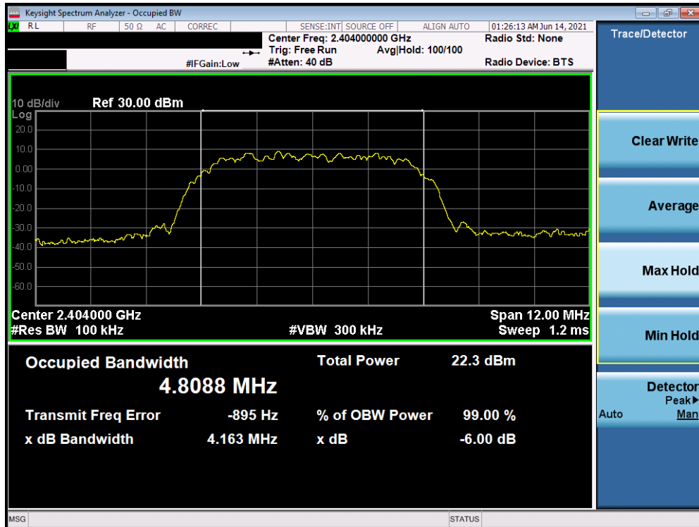
Plot 7-4. 6dB Bandwidth & 99% OBW Plot (Bluetooth (HDR8), 8Mbps, ePA – Ch. 1)
