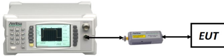
Figure 7-2. Test Instrument & Measurement Setup for Peak and Average Power Measurement
