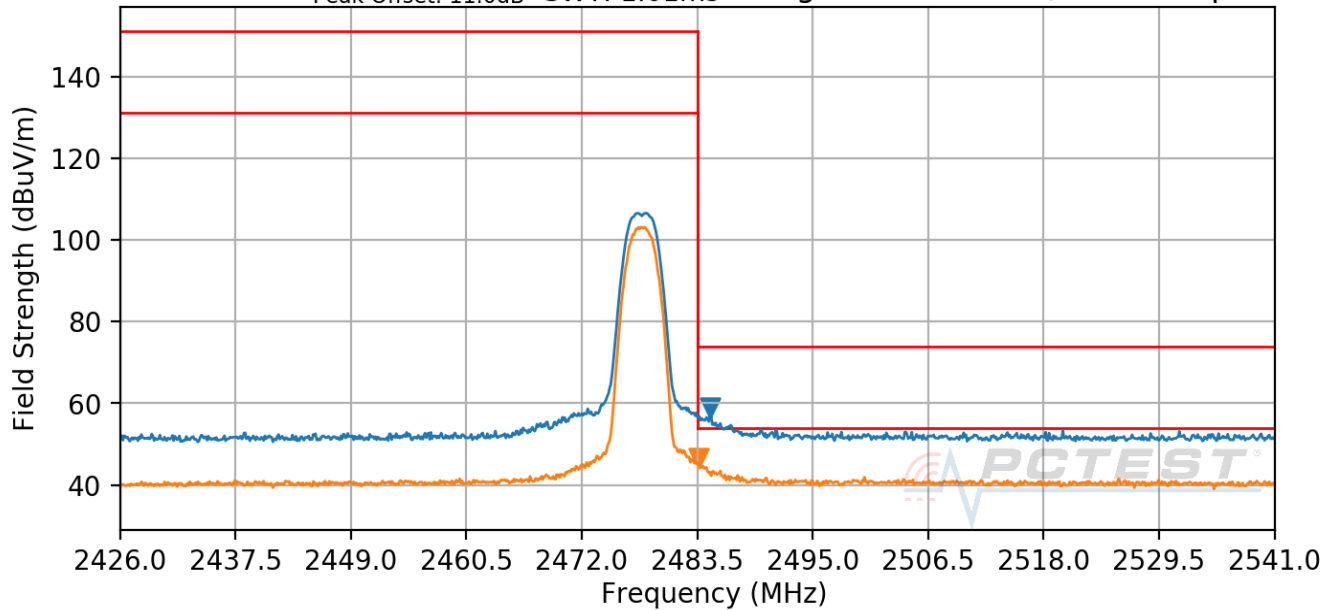
Plot 7-35. Radiated Restricted Upper Band Edge Measurement (Average & Peak)
