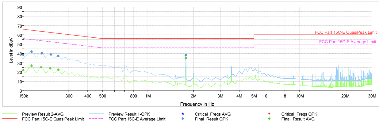
Plot 7-40. Line Conducted Plot with Bluetooth HDR (4Mbps, ePA – Ch.38, N, with AC/DC Adapter + Magnetic Charger)
