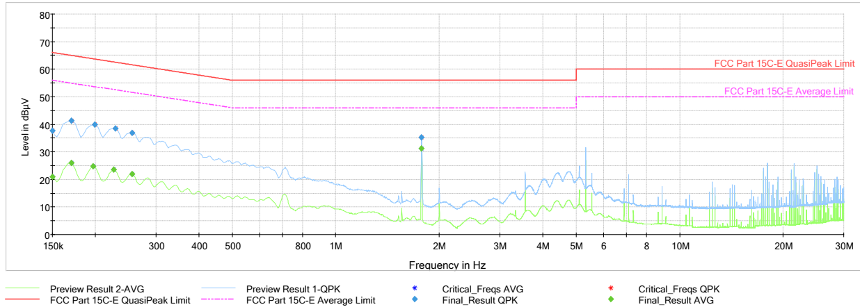
Plot 7-39. Line Conducted Plot with Bluetooth HDR4 (4Mbps, ePA – Ch.38, L1, with AC/DC Adapter + Magnetic Charger)
