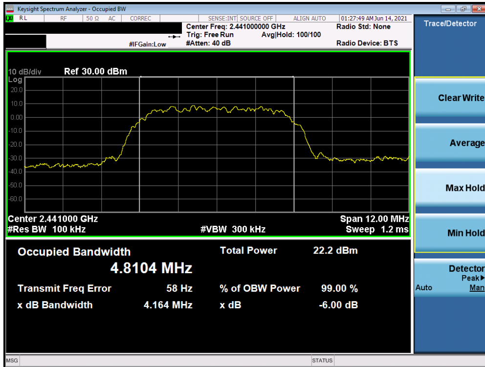
Plot 7-5. 6dB Bandwidth & 99% OBW Plot (Bluetooth (HDR8), 8Mbps, ePA – Ch. 38)
