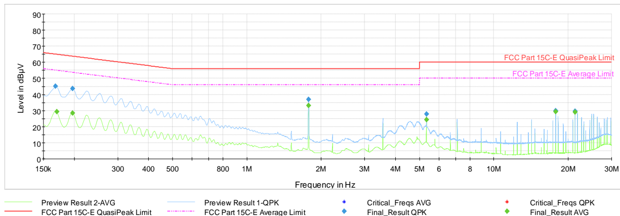
Plot 7-59. AC Line Conducted Plot with 802.11n UNII Band 2C – Ch.144 (N) with AC/DC Adaptor & Magnetic Charger
