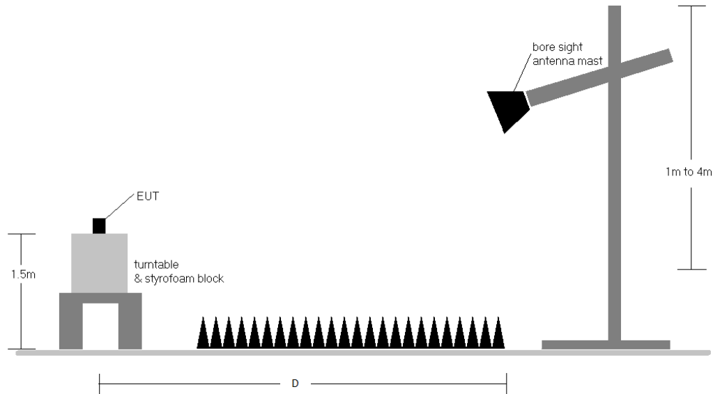
Figure 7-5. Radiated Measurement Setup
