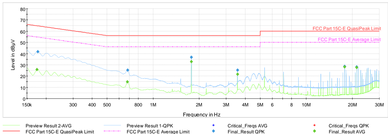
Plot 7-58. AC Line Conducted Plot with 802.11n UNII Band 2C – Ch.144 (L1) with AC/DC Adaptor & Magnetic Charger
