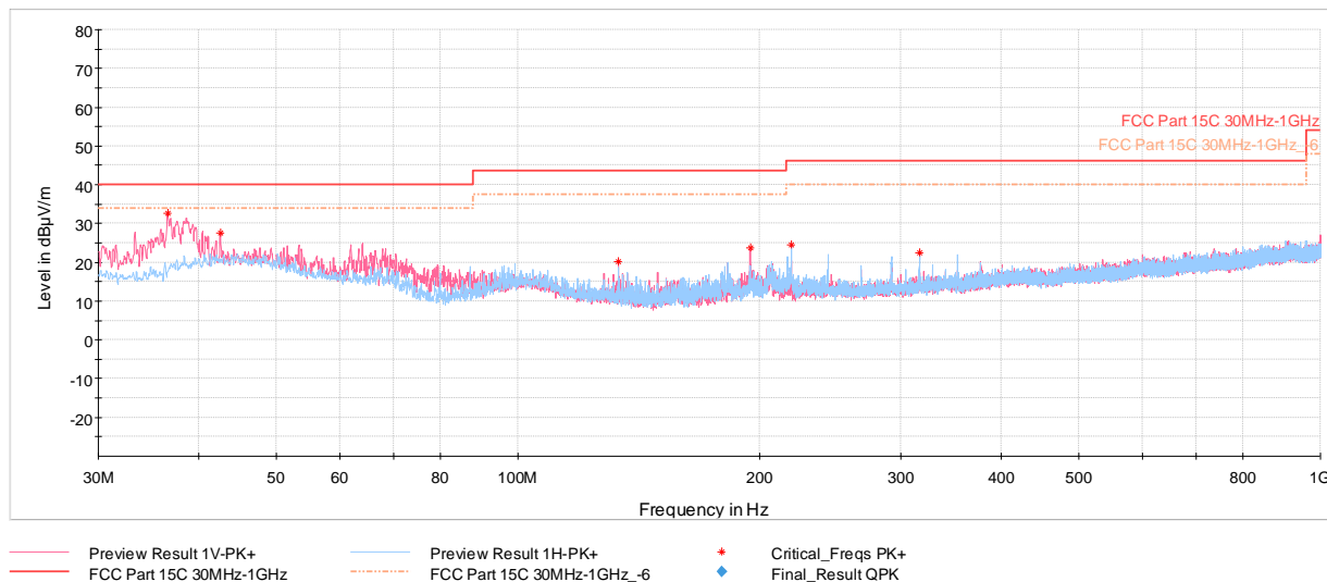
Plot 7-57. Radiated Spurious Emissions – Simultaneous Transmission below 1GHz with AC/DC Adaptor & Magnetic Charger
