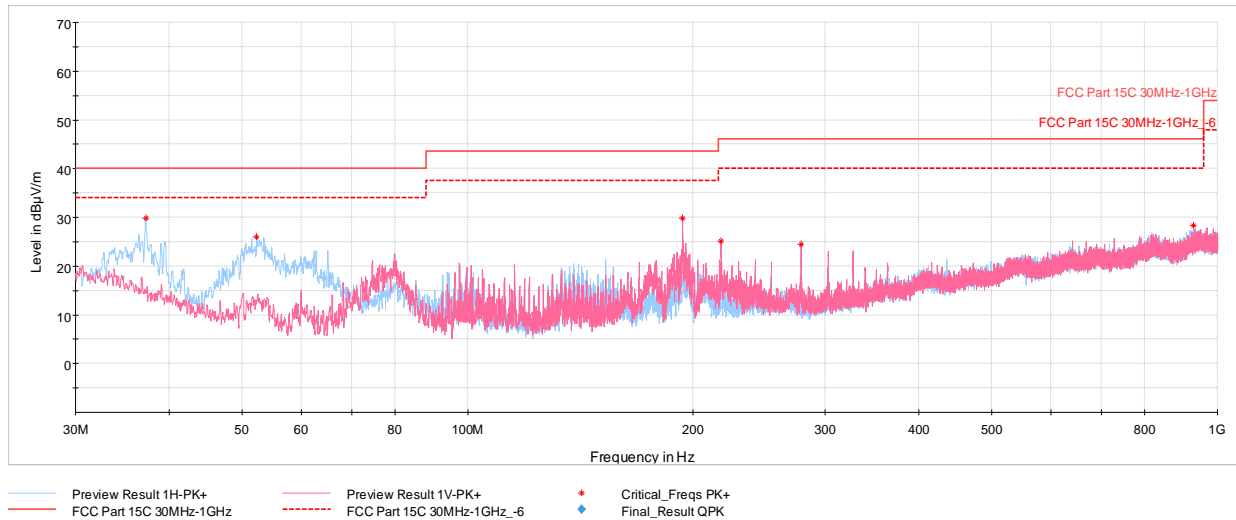
Plot 7-56. Radiated Spurious Emissions below 1GHz (802.11n – UNII 2C Ch. 144) with AC/DC Adaptor & Magnetic Charger
