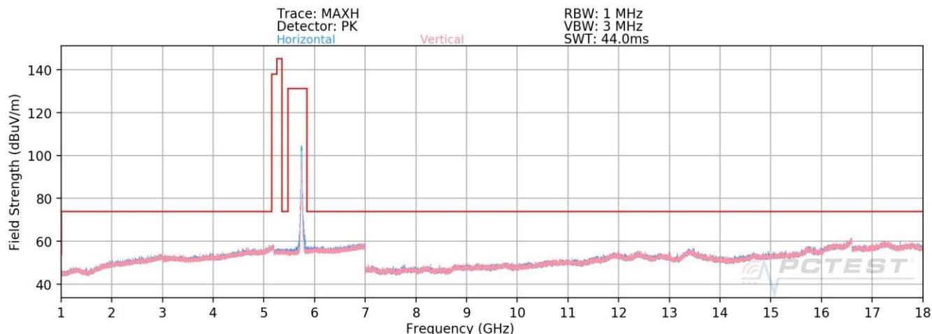
Plot 7-36. Radiated Spurious Emissions above 1GHz (802.11n – UNII 3 Ch. 149)
