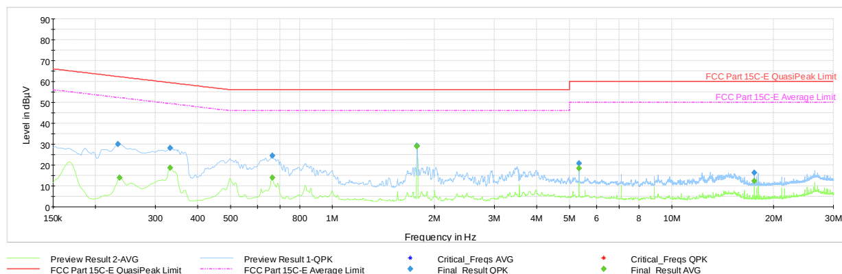
Plot 6-14. AC Line Conducted Plot (N - Mode 1, with AC/DC Adapter + Magnetic Charger)
