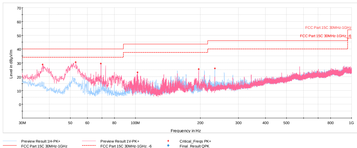
Plot 6-12. Radiated Spurious Emissions 30MHz – 1GHz (Mode 1, with AC/DC Adapter + Magnetic Charger)
