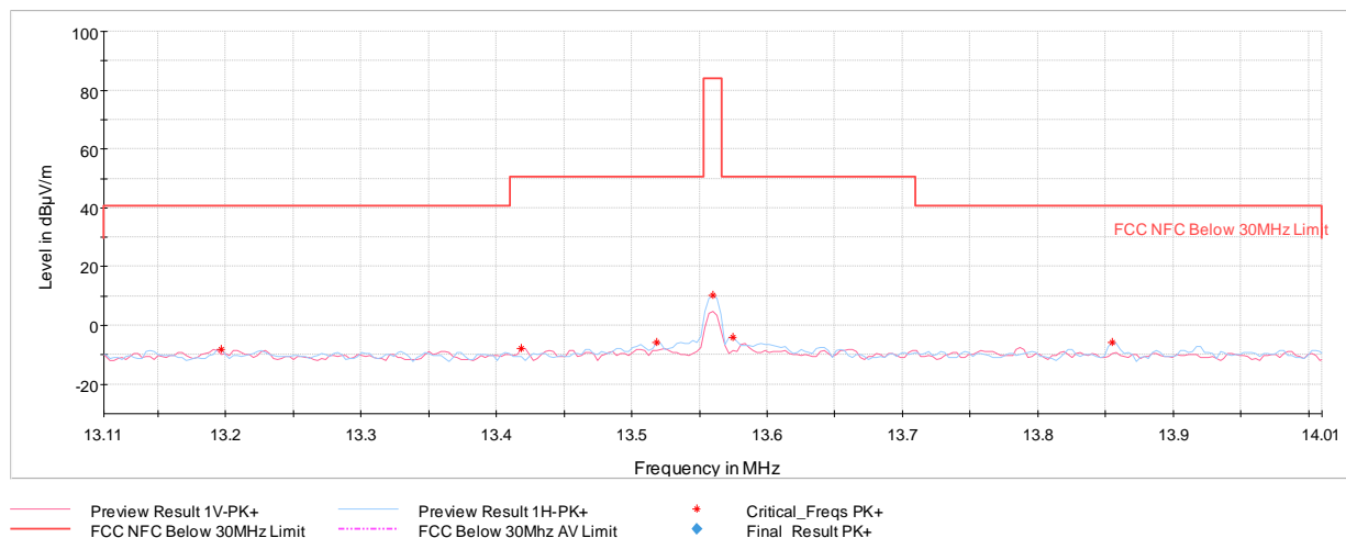
Plot 7-7. In Band Radiated Spurious Emissions (Reader 10% ASK 1 out of 256, AC/DC Adapter and Magnetic Charger)
