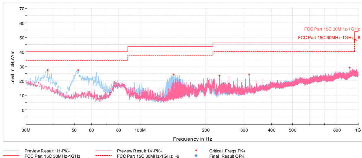
Plot 7-38. Radiated Spurious Plot below 1GHz (GFSK ePA – Ch.39, Pol. H & V, with AC/DC Adapter+ Magnetic Charger)
