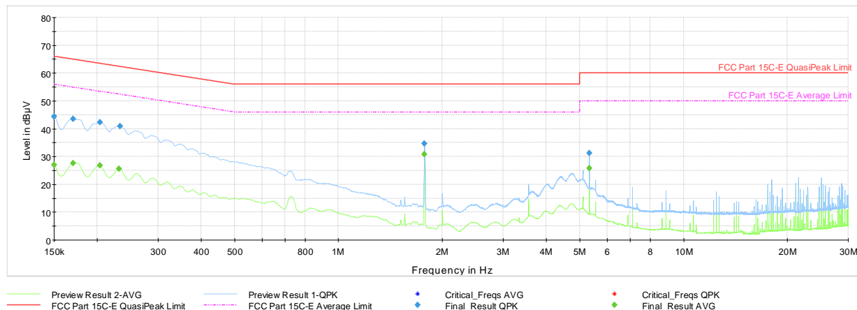
Plot 7-39. AC Line-Conducted Emissions (L1, GFSK ePA – Ch.39 with AC/DC Adapter + Magnetic Charger)
