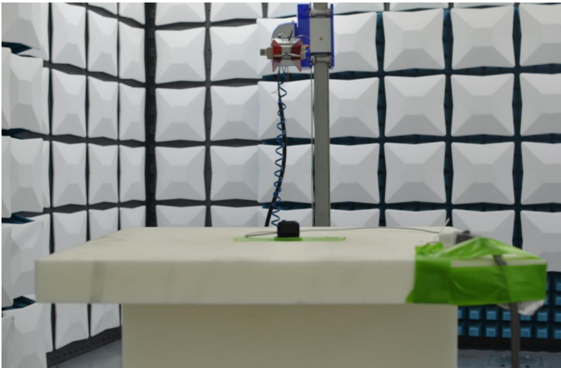
Figure 8: 1-18GHz Test Setup (Rear View)
