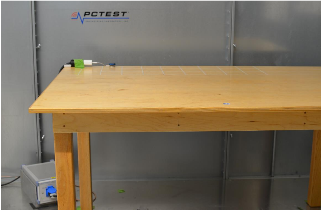
Figure 1: AC Line Conducted Emissions (Front View)
