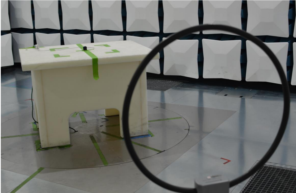
Figure 25: 9kHz-30MHz Test Setup (Front View)
