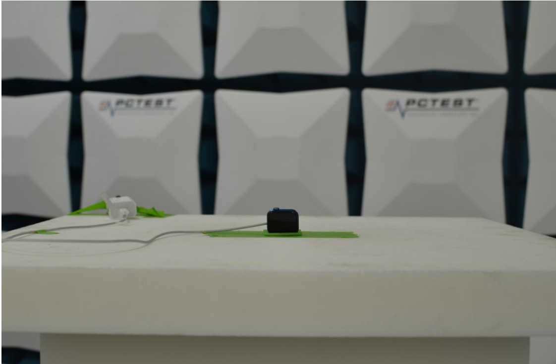
Figure 7: 1-18GHz Test Setup (Front View)
