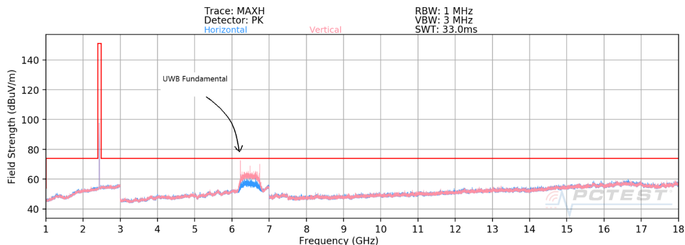
Plot 7-56. Radiated Spurious Simultaneous Transmission 1-18GHz
