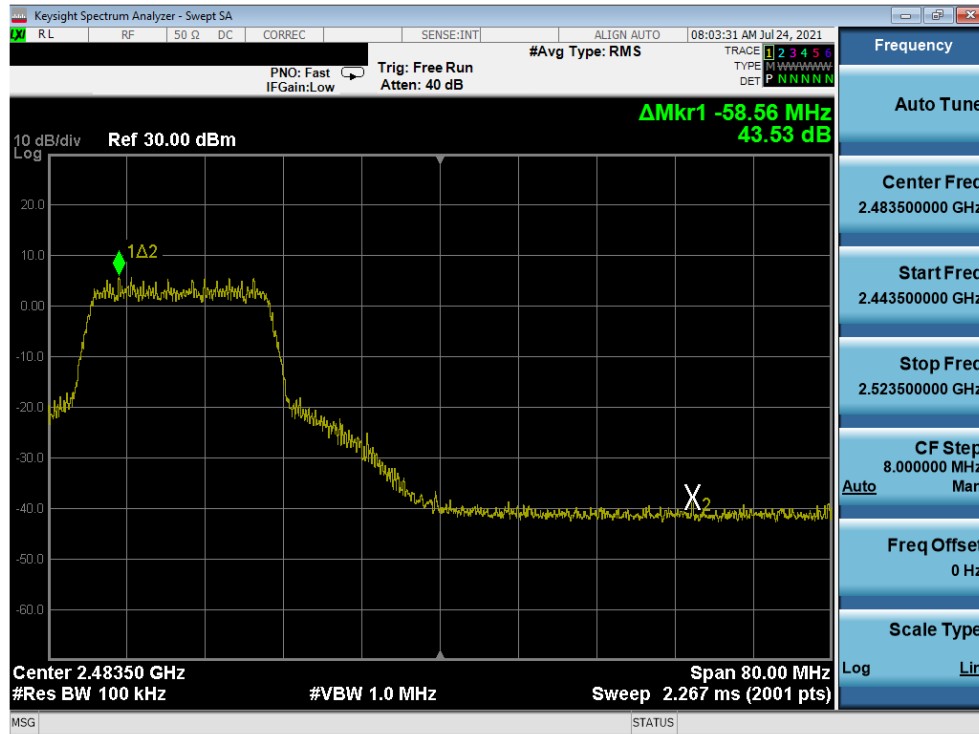
Plot 7-41. Band Edge Plot (802.11n MCS7 – Ch. 10)
