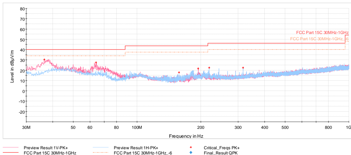
Plot 7-74. Radiated Spurious Emissions 30MHz-1GHz, with AC/DC Adaptor and Magnetic Charger
