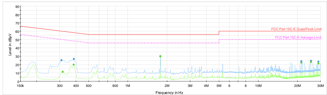
Plot 7-18.AC Line Conducted Plot 802.11b – Ch.1 (N), with Magnetic Charger and Laptop
