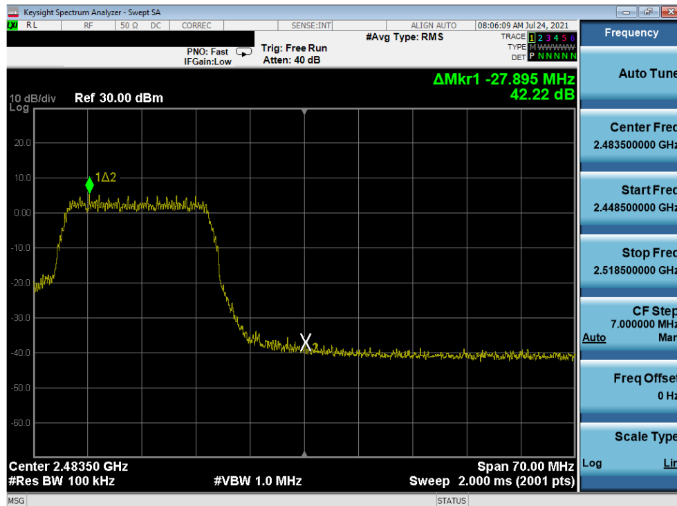
Plot 7-42. Band Edge Plot (802.11n MCS7 – Ch. 11)
