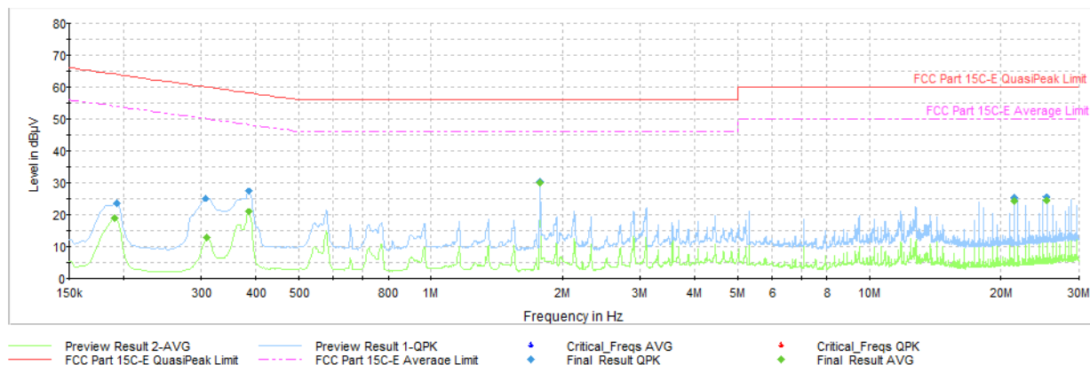
Plot 7-75.AC Line Conducted Plot 802.11b – Ch.1 (L1), with Magnetic Charger and Laptop
