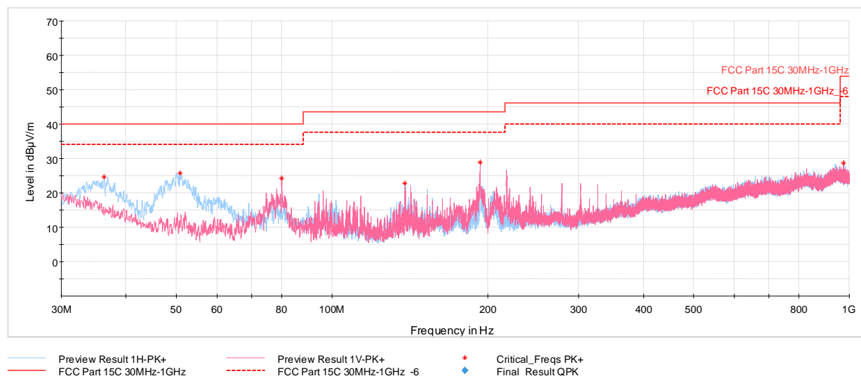
Plot 7-73. Radiated Spurious Emissions 30MHz-1GHz (802.11b – Ch.1, with AC/DC Adaptor and Magnetic Charger)
