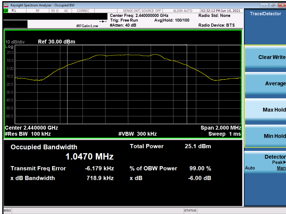
Plot 7-2. 6dB Bandwidth & 99% OBW Plot (Bluetooth (LE), 1Mbps, ePA – Ch. 19)
