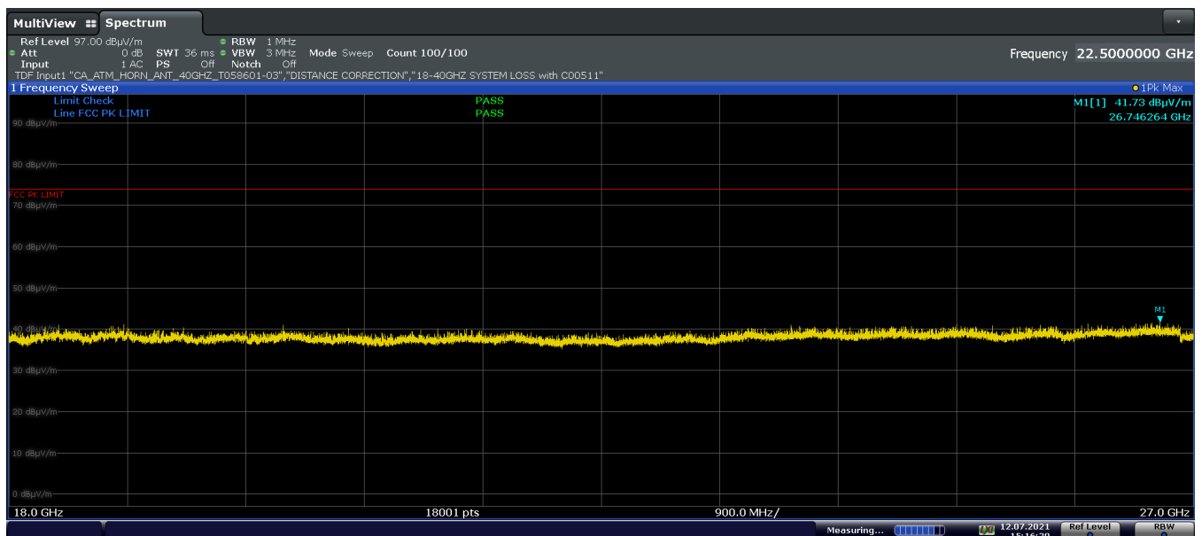
Plot 7-33. Radiated Spurious Plot Above 18GHz (1Mbps, ePA – Ch.19, Pol. V)
