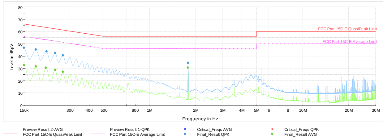
Plot 7-39. AC Line Conducted Plot with Bluetooth LE (1Mbps, ePA – Ch.19, L1, with AC/DC Adapter + Magnetic Charger)
