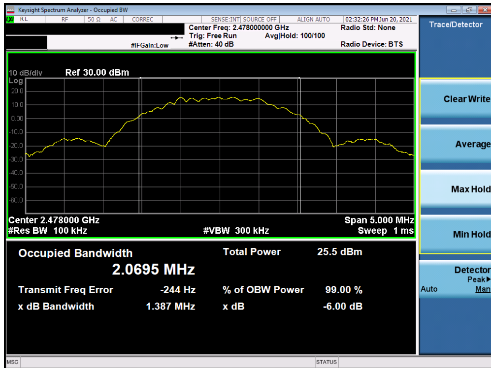
Plot 7-6. 6dB Bandwidth & 99% OBW Plot (Bluetooth (LE), 2Mbps, ePA – Ch. 38)
