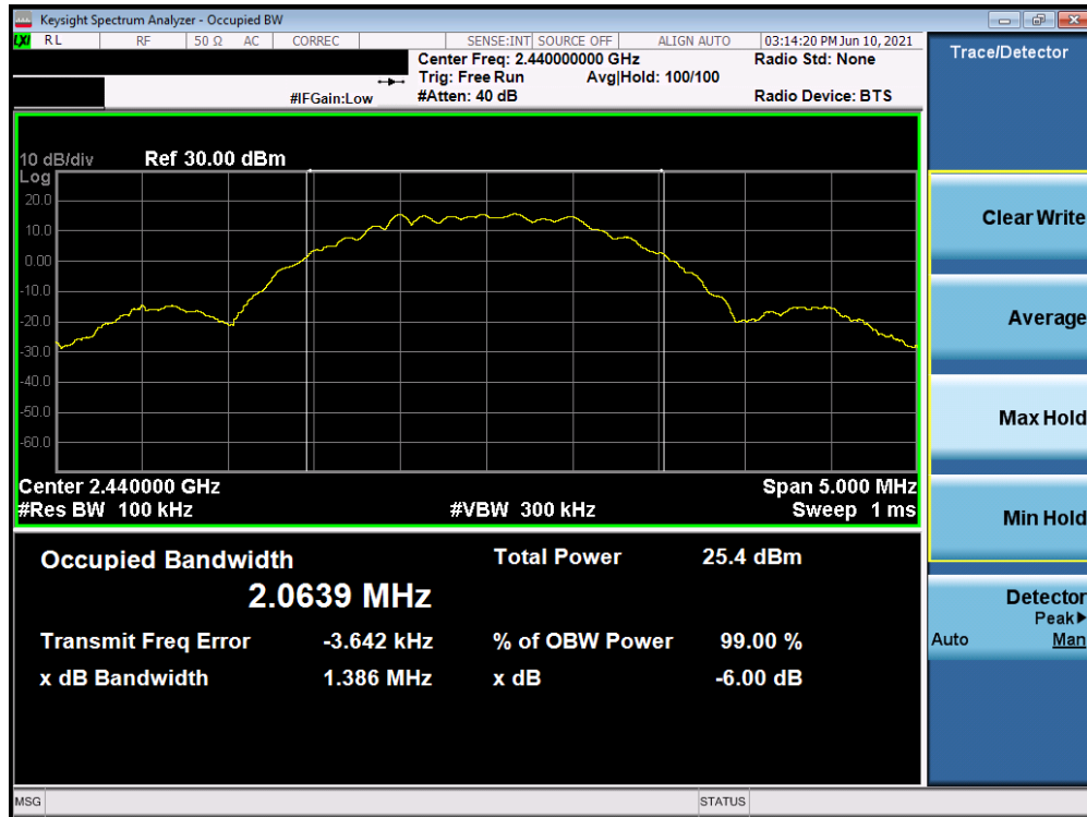
Plot 7-5. 6dB Bandwidth & 99% OBW Plot (Bluetooth (LE), 2Mbps, ePA – Ch. 19)
