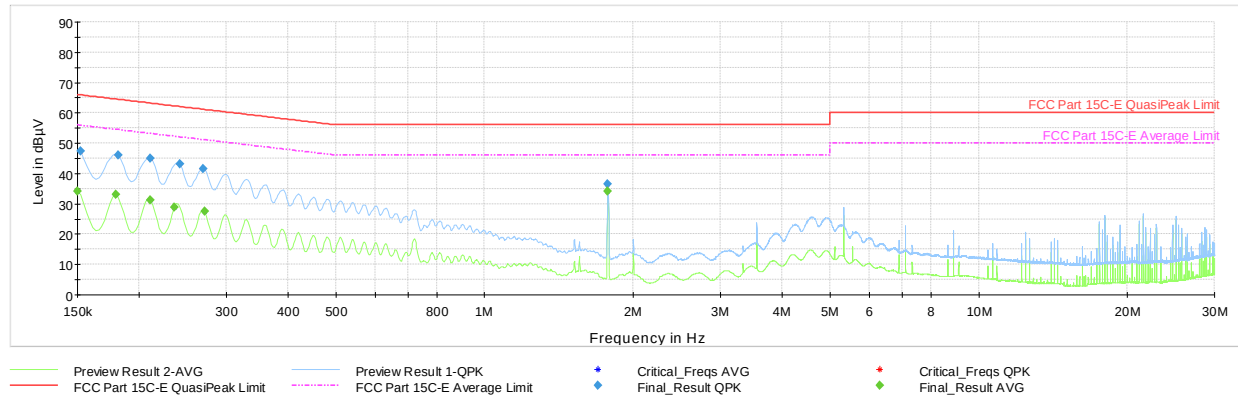
Plot 7-40. Line Conducted Plot with Bluetooth LE (1Mbps, ePA – Ch.19, N, with AC/DC Adapter + Magnetic Charger)
