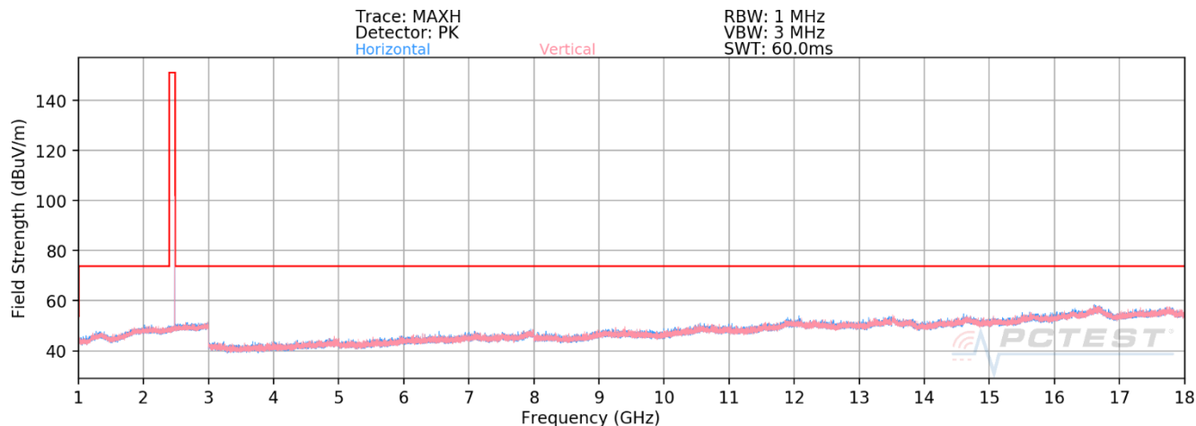
Plot 7-31. Radiated Spurious Plot Above 1GHz (1Mbps ePA – Ch. 39, Ant. Pol. H & V)
