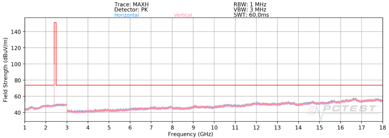
Plot 7-29. Radiated Spurious Plot Above 1GHz (1Mbps, ePA – Ch. 0, Ant. Pol. H & V)
