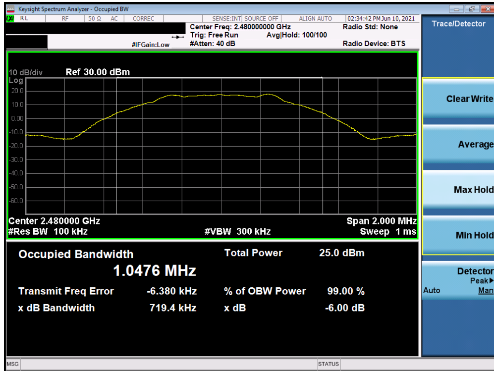
Plot 7-3. 6dB Bandwidth & 99% OBW Plot (Bluetooth (LE), 1Mbps, ePA – Ch. 39)
