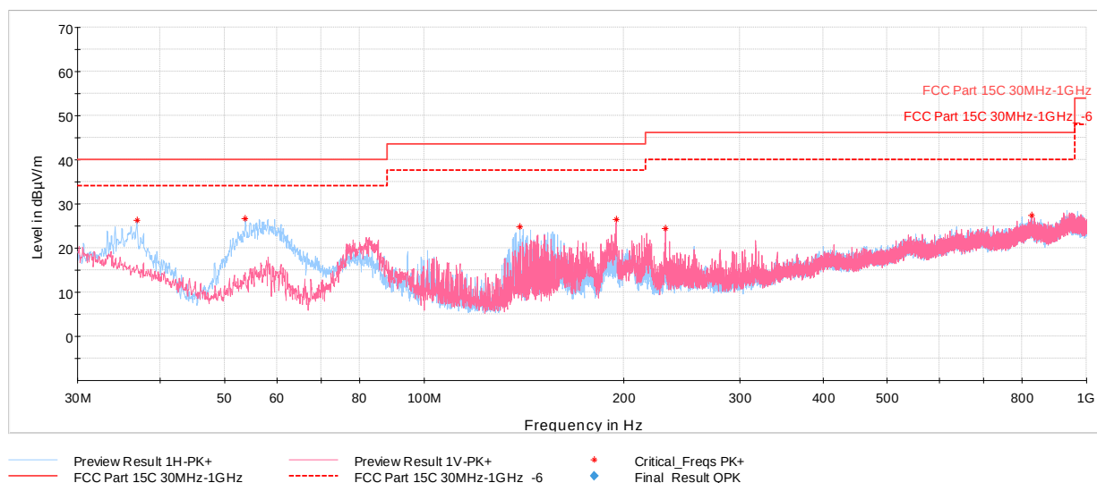
Plot 7-38. Radiated Spurious Plot Below 1GHz 1Mbps, ePA – Ch.19, Pol. H & V, with AC/DC Adapter + Magnetic Charger)
