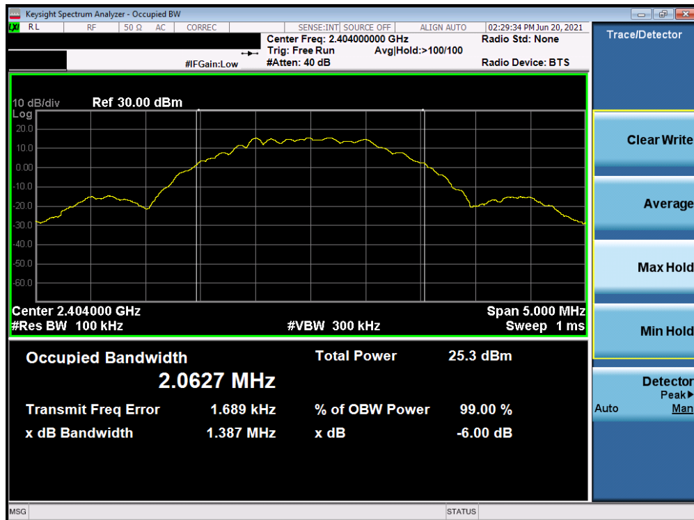
Plot 7-4. 6dB Bandwidth & 99% OBW Plot (Bluetooth (LE), 2Mbps, ePA – Ch. 1)
