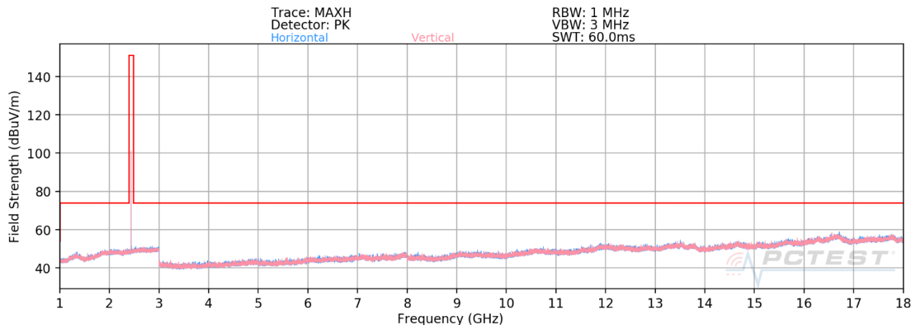
Plot 7-30. Radiated Spurious Plot Above 1GHz (1Mbps, ePA – Ch. 19, Ant. Pol. H & V)
