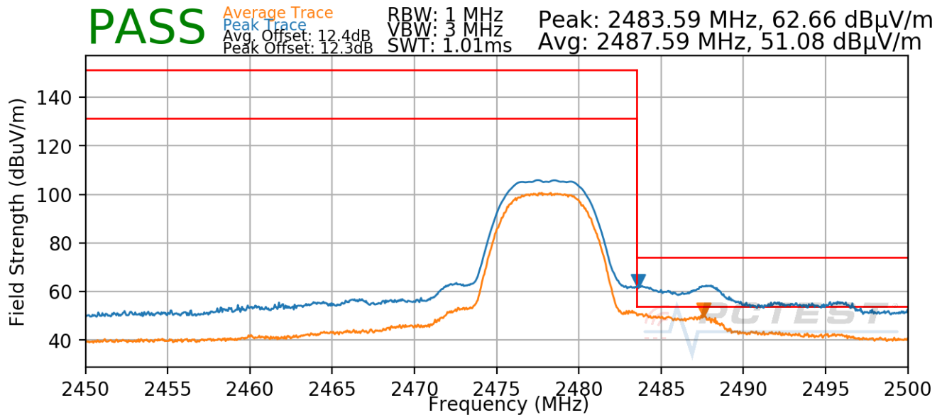
Plot 7-37. Radiated Restricted Upper Band Edge Measurement (Average & Peak)
