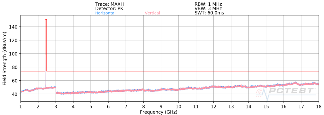
Plot 7-29. Radiated Spurious Emissions Above 1GHz (4Mbps, HDR4, ePA – Ch. 1, Ant. Pol. H & V)
