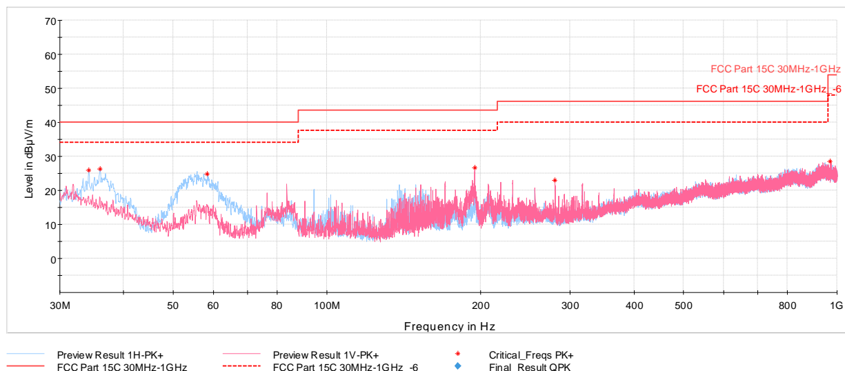
Plot 7-38. Radiated Spurious Emissions below 1GHz (HDR4 ePA – Ch.38, Pol. H & V, with AC/DC Adapter + Magnetic Charger)
