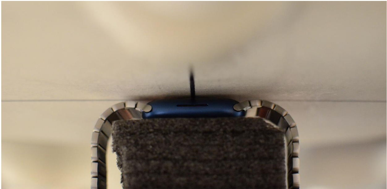
SAR Test Setup Photo 5: Extremity, Aluminum with Metal Links Wristband, Back side at 0.0 cm
