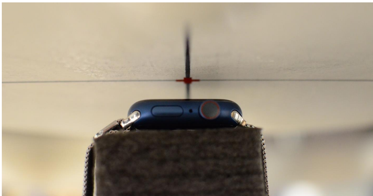
SAR Test Setup Photo 3: Head, Aluminum with Metal Loop Wristband, Front side at 1.0 cm
