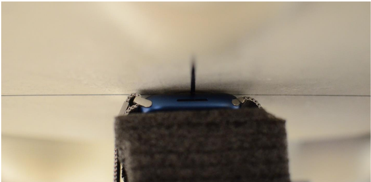
SAR Test Setup Photo 6: Extremity, Aluminum with Metal Loop Wristband, Back side at 0.0 cm
