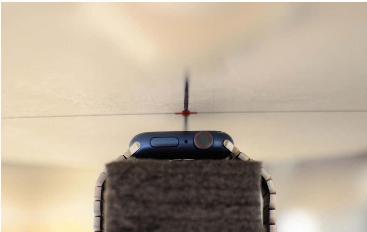
SAR Test Setup Photo 2: Head, Aluminum with Metal Links Wristband, Front side at 1.0 cm
