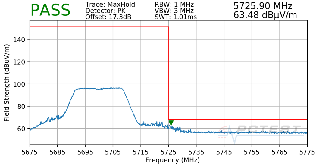
Plot 7-47. Radiated Upper Band Edge Plot (Peak - UNII Band 2C)
