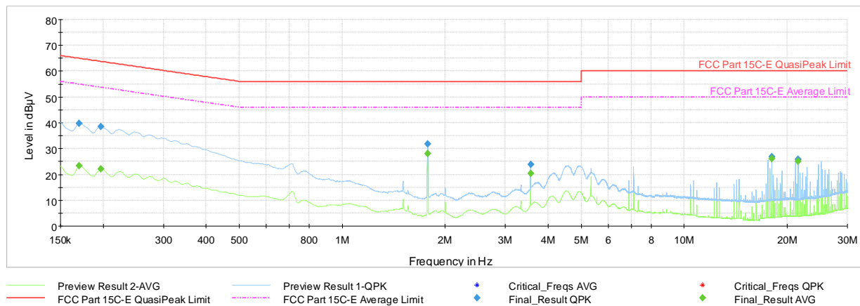
Plot 7-54. AC Line Conducted Plot with 802.11n UNII Band 2C – Ch.157 (L1) with AC/DC Adaptor & Magnetic Charger
