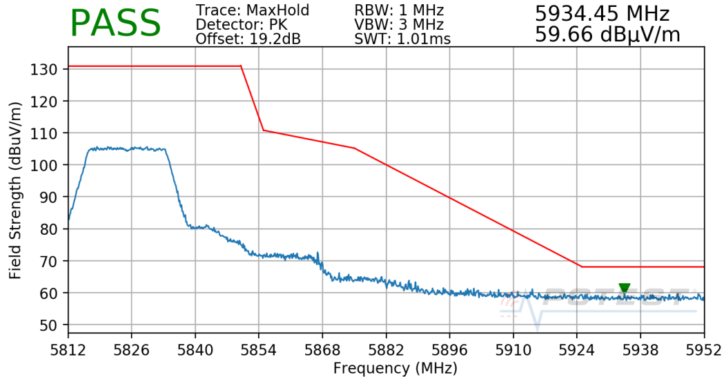
Plot 7-51. Radiated Upper Band Edge Plot (Peak – UNII Band 3)
