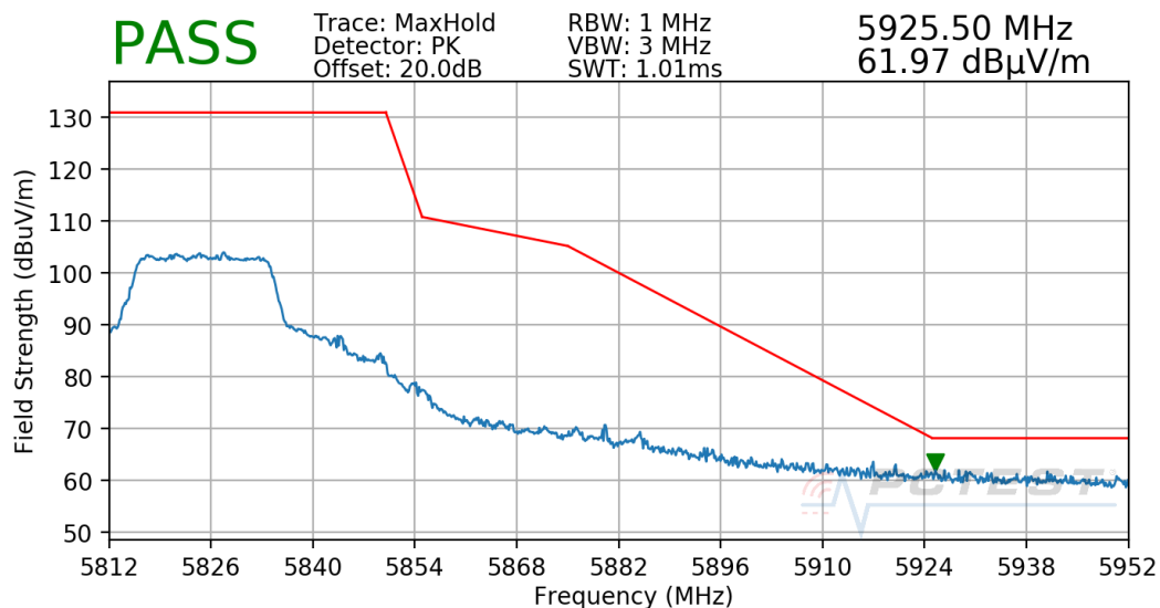
Plot 7-52. Radiated Upper Band Edge Plot (Peak – UNII Band 3)
