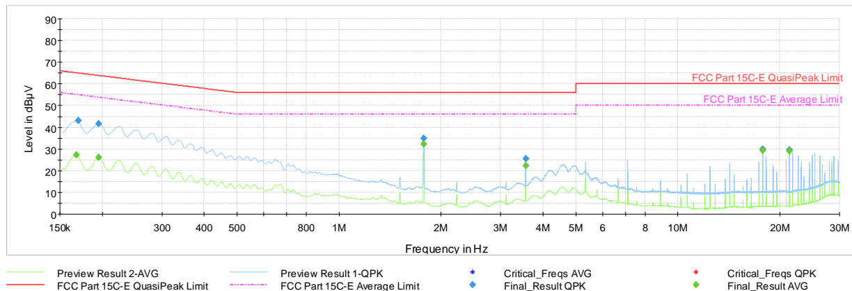
Plot 7-55. AC Line Conducted Plot with 802.11n UNII Band 2C – Ch.157 (N) with AC/DC Adaptor & Magnetic Charger
