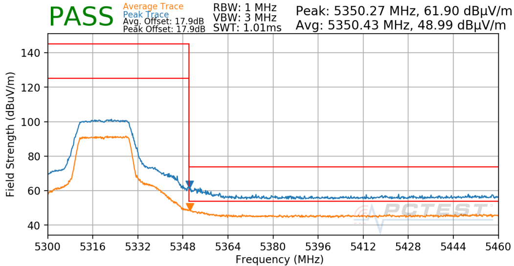
Plot 7-41. Radiated Upper Band Edge Plot (UNII Band 2A)
