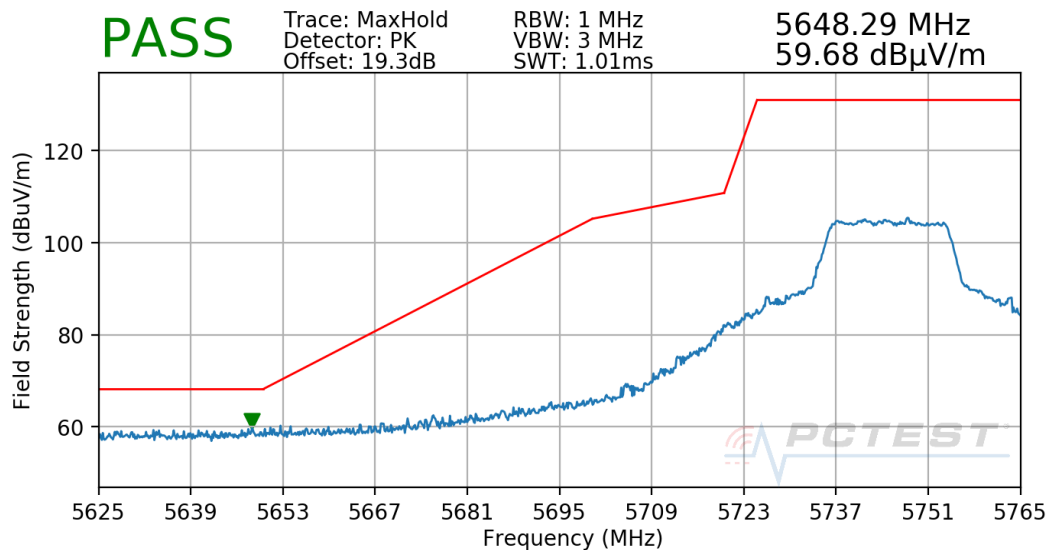
Plot 7-50. Radiated Lower Band Edge Plot (Peak – UNII Band 3)
