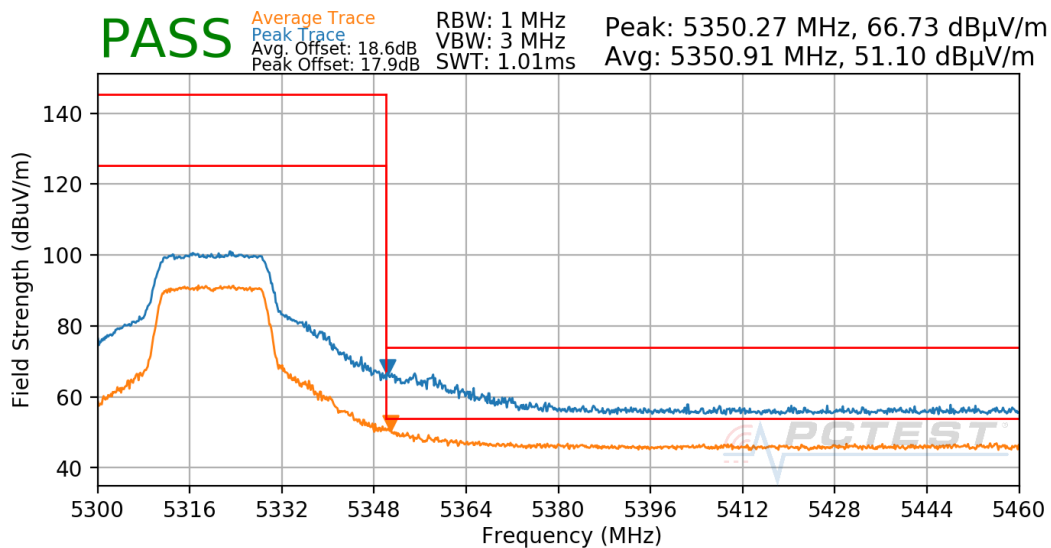
Plot 7-42. Radiated Upper Band Edge Plot (UNII Band 2A)
