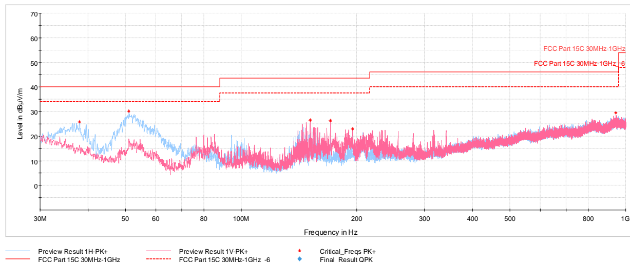
Plot 7-53. Radiated Spurious Emissions below 1GHz (802.11n – UNII 3 Ch. 157) with AC/DC Adaptor & Magnetic Charger
