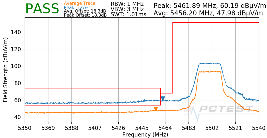
Plot 7-43. Radiated Lower Band Edge Plot (UNII Band 2C)
