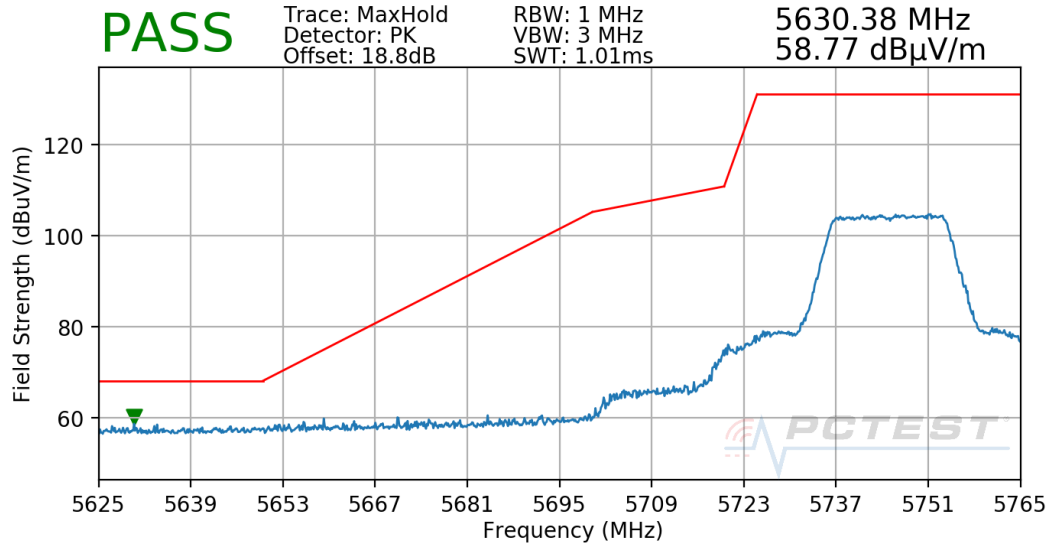
Plot 7-49. Radiated Lower Band Edge Plot (Peak – UNII Band 3)
