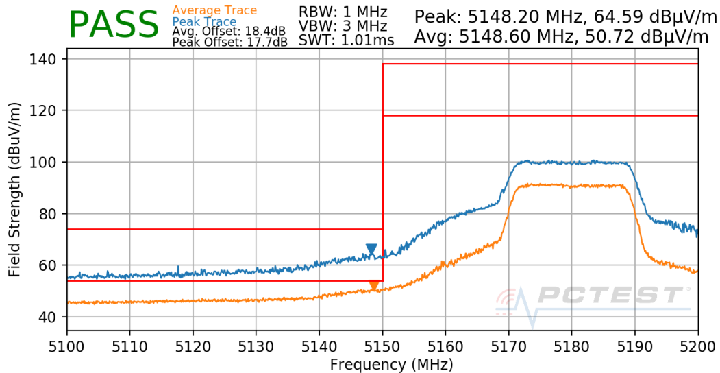
Plot 7-40. Radiated Lower Band Edge Plot (UNII Band 1)
