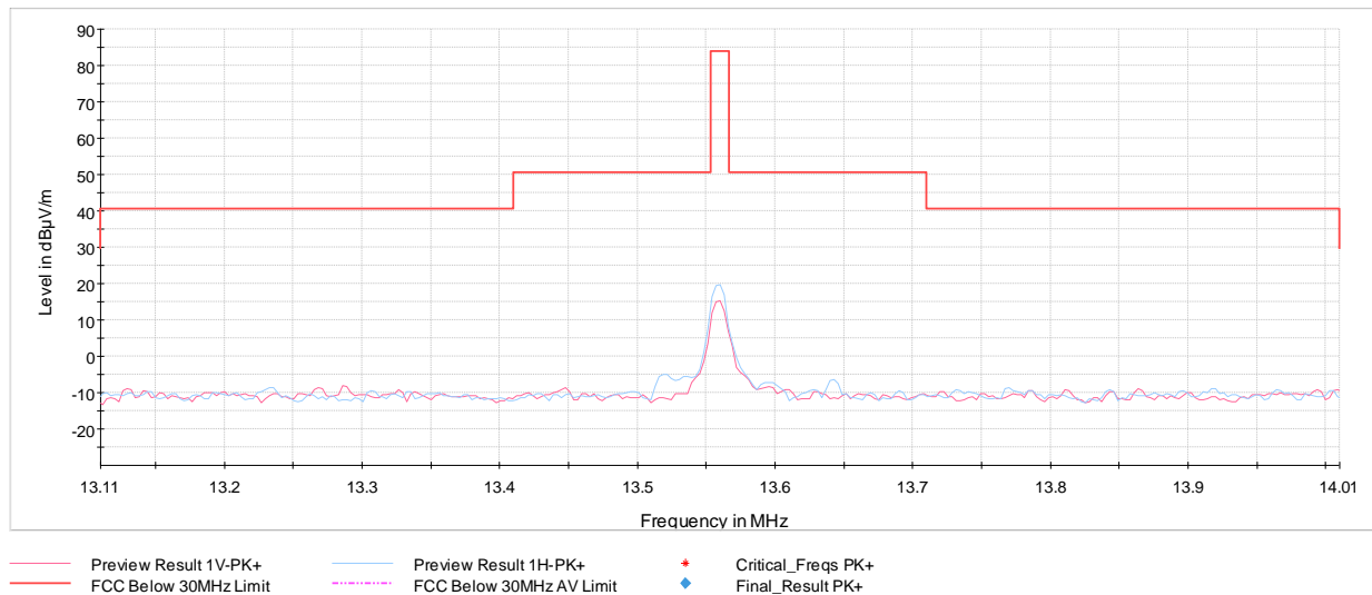
Plot 7-6. In Band Radiated Spurious Emissions (CE A 848kbps, with WCP + AC/DC Adapter)
