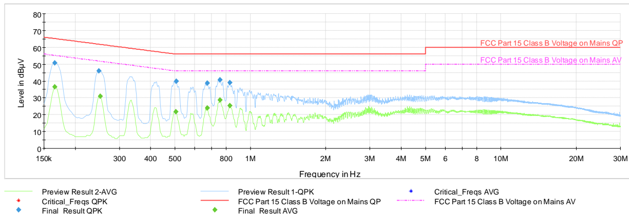
Plot 7-64. AC Line Conducted Emissions with 802.11b Ch.6 (N, with WCP + AC/DC Adapter)
