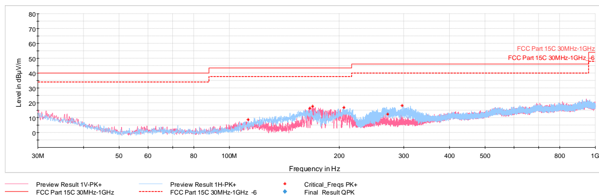
Plot 7-50. Radiated Spurious Emissions – Simultaneous Transmission below 1GHz with WCP + AC/DC Adapter
