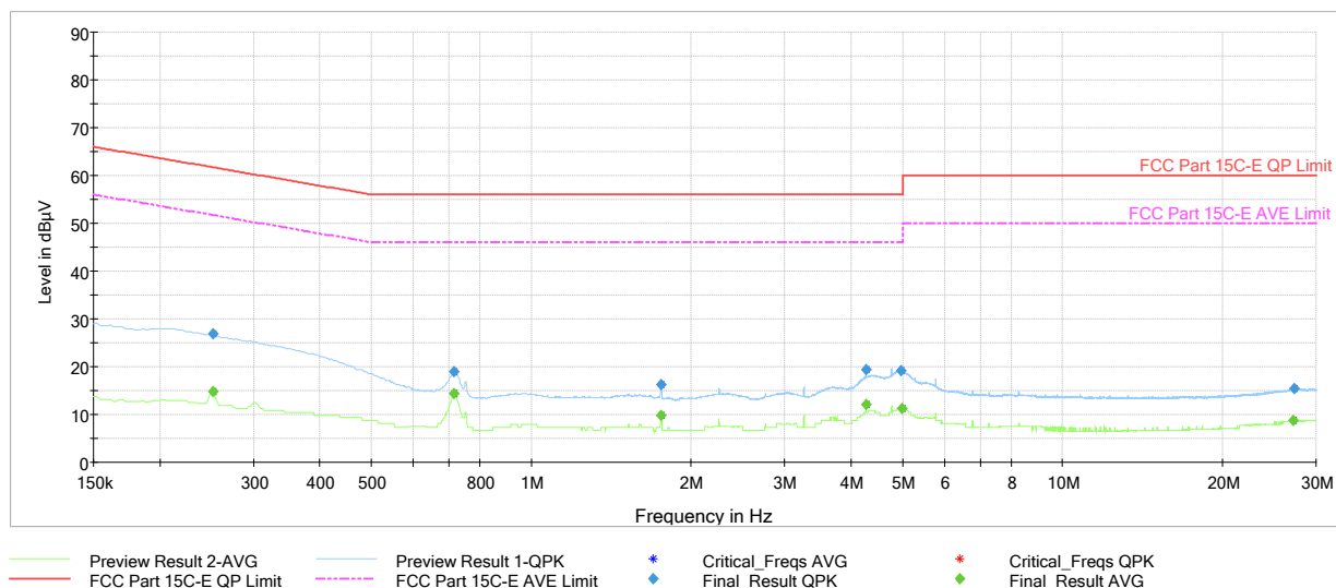
Plot 7-44. AC Line Conducted Emission with GFSK ePA Ch.0 (N, with AC/DC Adapter)
