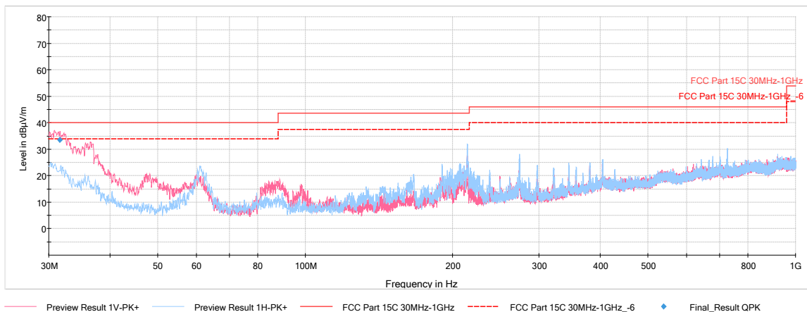
Plot 7-41. Radiated Spurious Emissions 30MHz-1GHz (GFSK ePA – Ch.0, with AC/DC Adapter)
