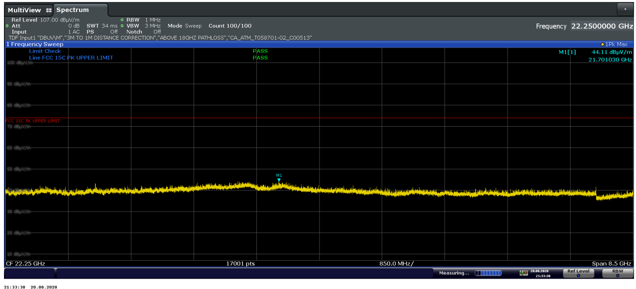
Plot 7-32. Radiated Spurious Emissions 18-26.5GHz (BT GFSK ePA – Ch.0, Pol. H)
