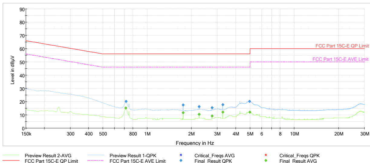
Plot 7-43. AC Line Conducted Emission with GFSK ePA Ch.0 (L1, with AC/DC Adapter)
