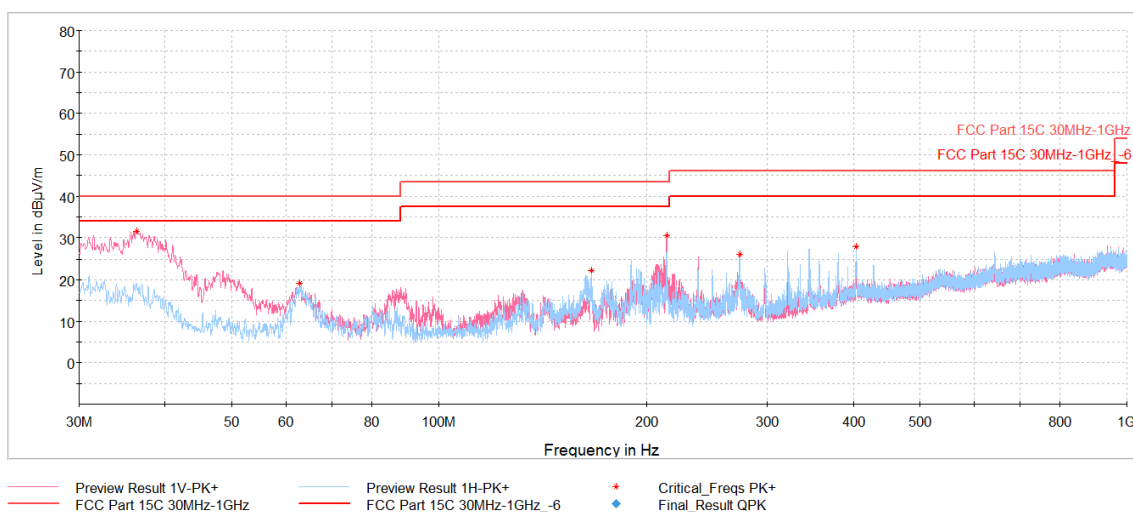
Plot 7-42. Radiated Spurious Emissions 30MHz-1GHz (Simultaneous Transmission, with AC/DC Adapter)
