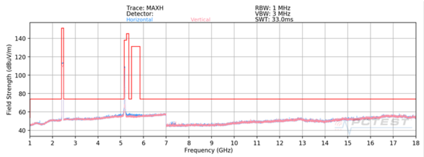
Plot 7-34. Radiated Spurious Emissions 1-18GHz (Simultaneous Transmission)
