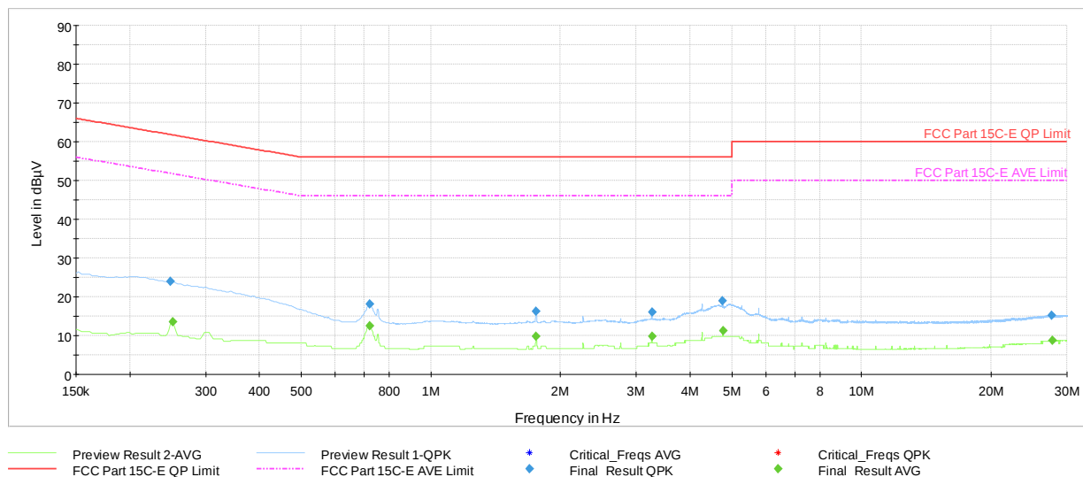
Plot 7-24. AC Line Conducted Emission with Thread (N, Ch.25, with AC/DC Adapter)
