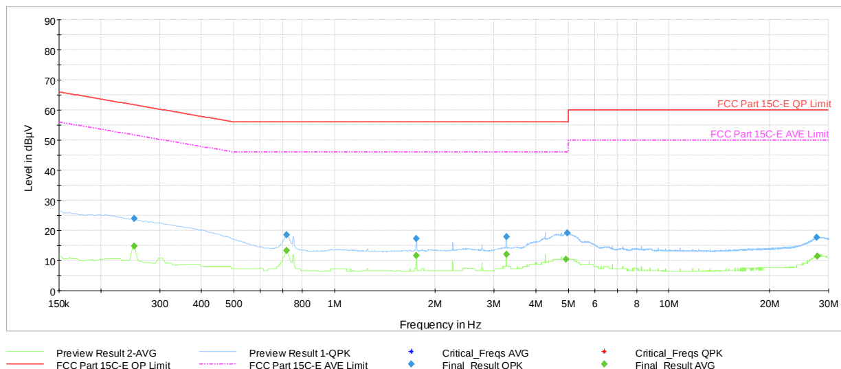
Plot 7-23. AC Line Conducted Emission with Thread (L1, Ch.25, with AC/DC Adapter via USB-C Cable)
