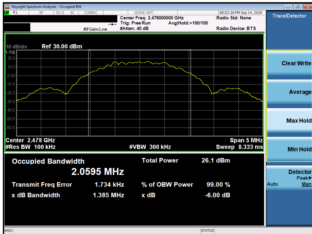
Plot 7-6. 6dB Bandwidth Plot (Bluetooth (LE), 2Mbps, ePA – Ch. 38)
