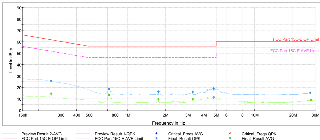
Plot 7-40. AC Line Conducted Emission with Bluetooth HDR (N – 4Mbps, ePA, Ch.1, with AC/DC Adapter)
