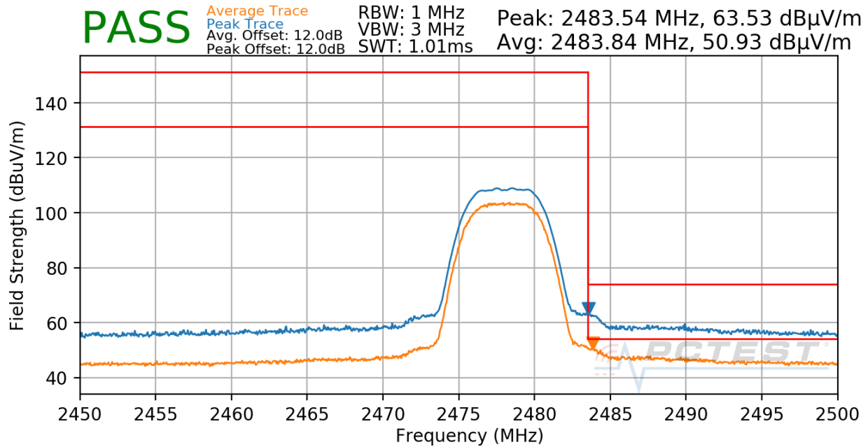
Plot 7-37. Radiated Restricted Upper Band Edge Measurement
