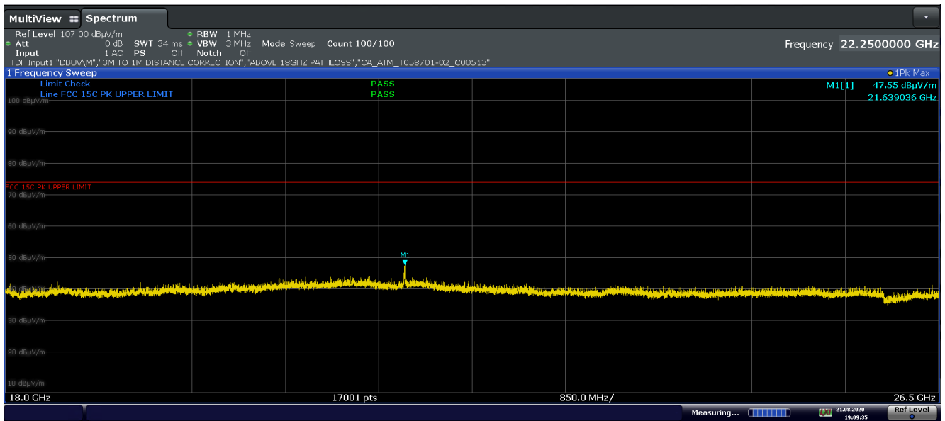
Plot 7-33. Radiated Spurious Emissions 18-26.5GHz (4Mbps, ePA – Ch.1, Ant. Pol. V)
