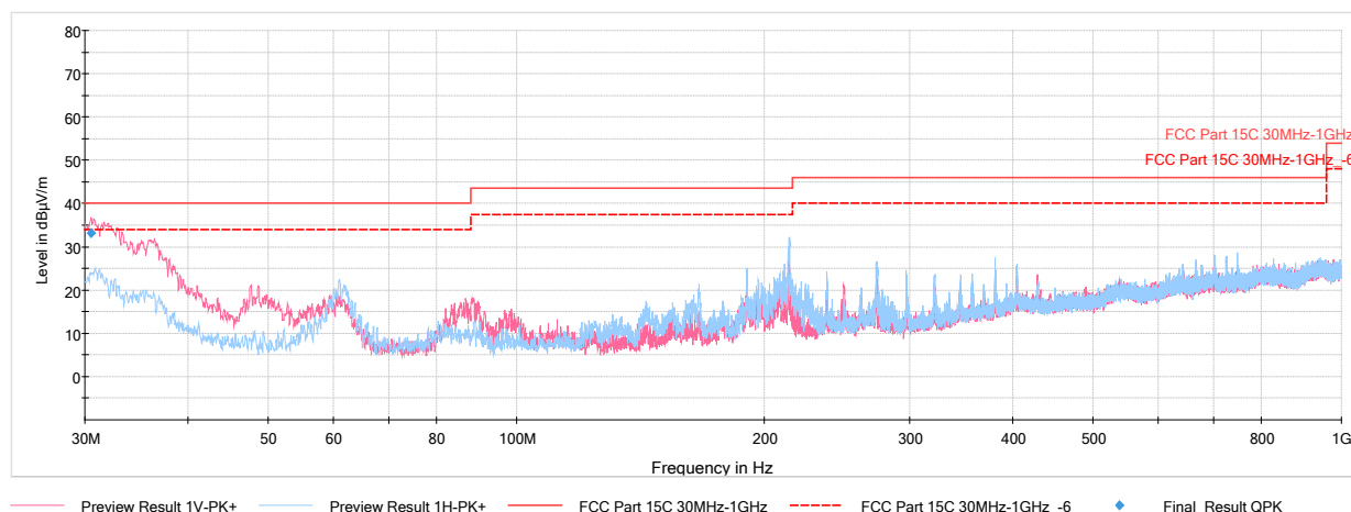
Plot 7-38. Radiated Spurious Emissions 30MHz-1GHz (4Mbps, ePA – Ch.1, with AC/DC Adapter)
