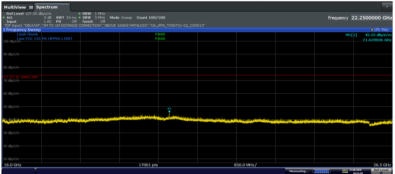
Plot 7-32. Radiated Spurious Emissions 18-26.5GHz (4Mbps, ePA – Ch.1, Ant. Pol. H)
