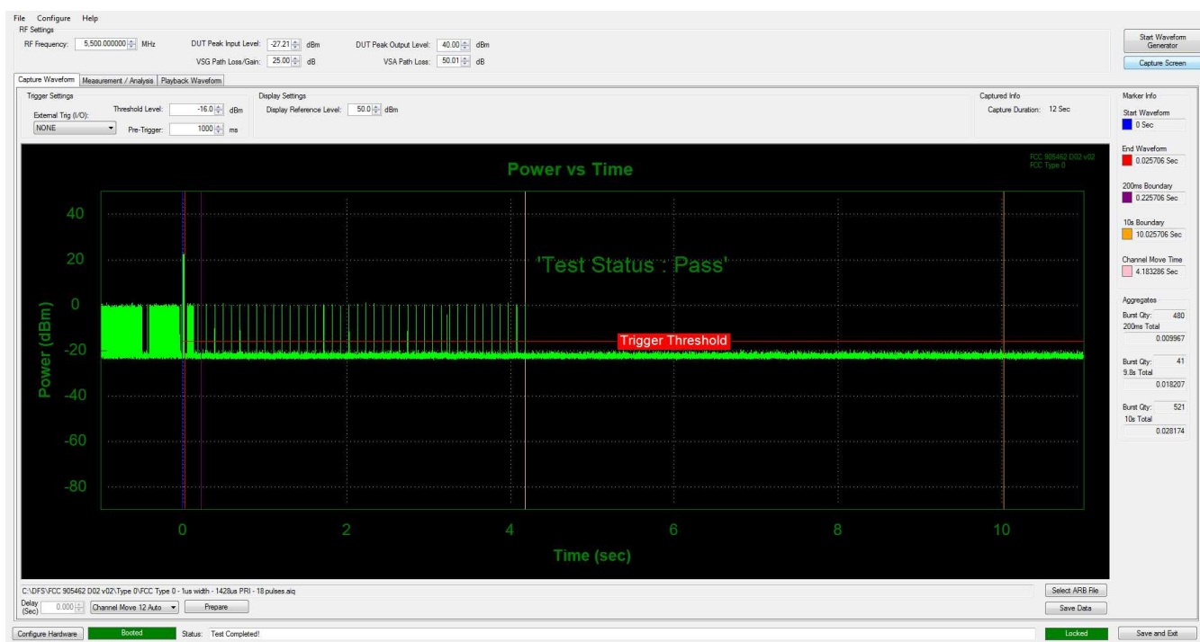
Figure 9-8: 5500MHz - Channel Move/ Closing Transmission Time – Mode 2 (20 MHz)
