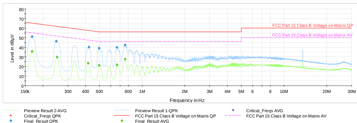
Plot 7-13. AC Line-Conducted Test Plot (N, Reader 10% Ask 1 out of 4, with WCP + AC/DC Adapter)
