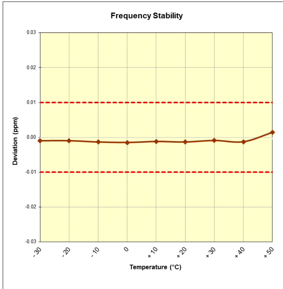
Figure 7-3. Frequency Stability Plot (CE B 848kbps)
