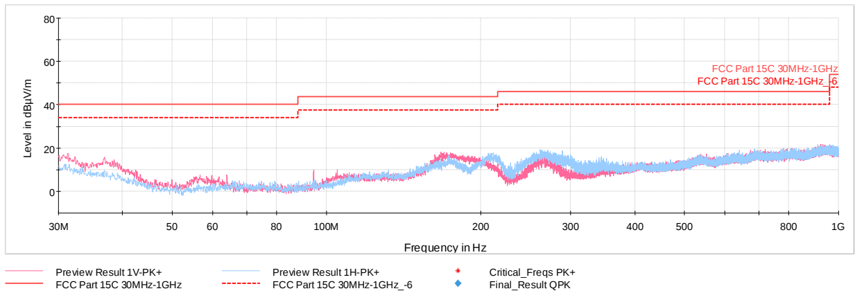
Plot 7-11. Radiated Spurious Emissions 30MHz – 1GHz (Reader 10% Ask 1 out of 4, with WCP + AC/DC Adapter)
