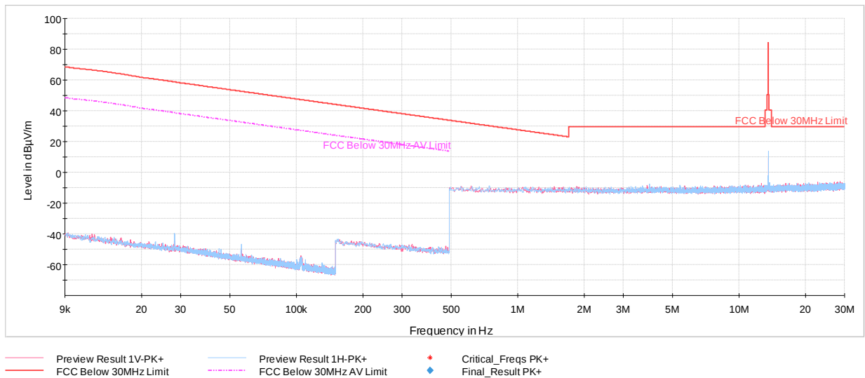
Plot 7-9. Radiated Spurious Emissions 9kHz – 30MHz (Reader 10% Ask 1 out of 4, with WCP + AC/DC Adapter)
