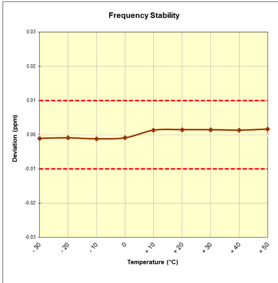
Figure 7-4. Frequency Stability Plot (Reader 10% Ask 1 out of 4)
