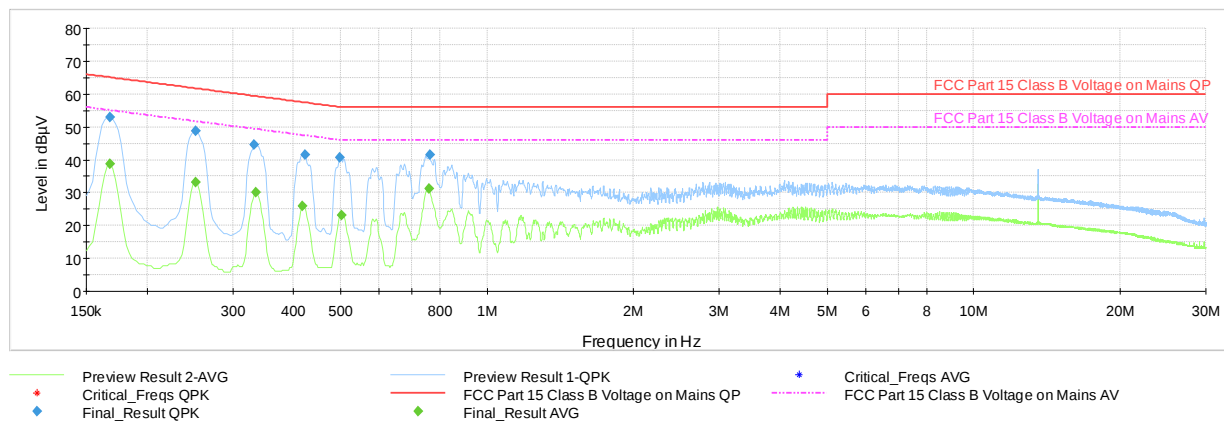
Plot 7-12. AC Line-Conducted Test Plot (L1, Reader 10% Ask 1 out of 4, with WCP + AC/DC Adapter)
